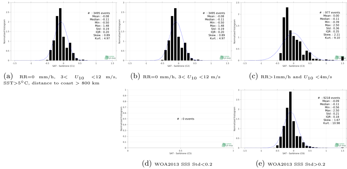
Figure 12: Normalized histogram of \Delta SSS (SMAP SSS L3 v4 - Monthly (RSS) - Saildrone) for 5 different subdatasets corresponding to: RR=0 mm/h, 3 < U_{10} < 12 m/s, SST > 5°C, distance to coast > 800 km (a), RR=0 mm/h, 3 < U_{10} < 12 m/s (b), RR > 1mm/h and U_{10} < 4 m/s (c), WOA2013 SSS Std < 0.2 (d), WOA2013 SSS Std > 0.2 (e).
