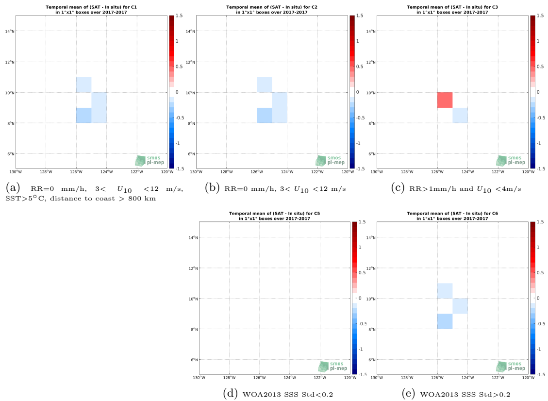
Figure 11: Temporal mean gridded over spatial boxes of size 1^\circ \times 1^\circ of \Delta SSS (SMAP SSS L3 v4 - Monthly (RSS) - Saildrone) for 5 different subdatasets corresponding to:RR=0 mm/h, 3 < U_{10} < 12 m/s, SST >5^\circ C, distance to coast > 800 km (a), RR=0 mm/h, 3 < U_{10} < 12 m/s (b), RR >1 mm/h and U_{10} < 4 m/s (c), WOA2013 SSS Std <0.2 (d), WOA2013 SSS Std >0.2 (e).
