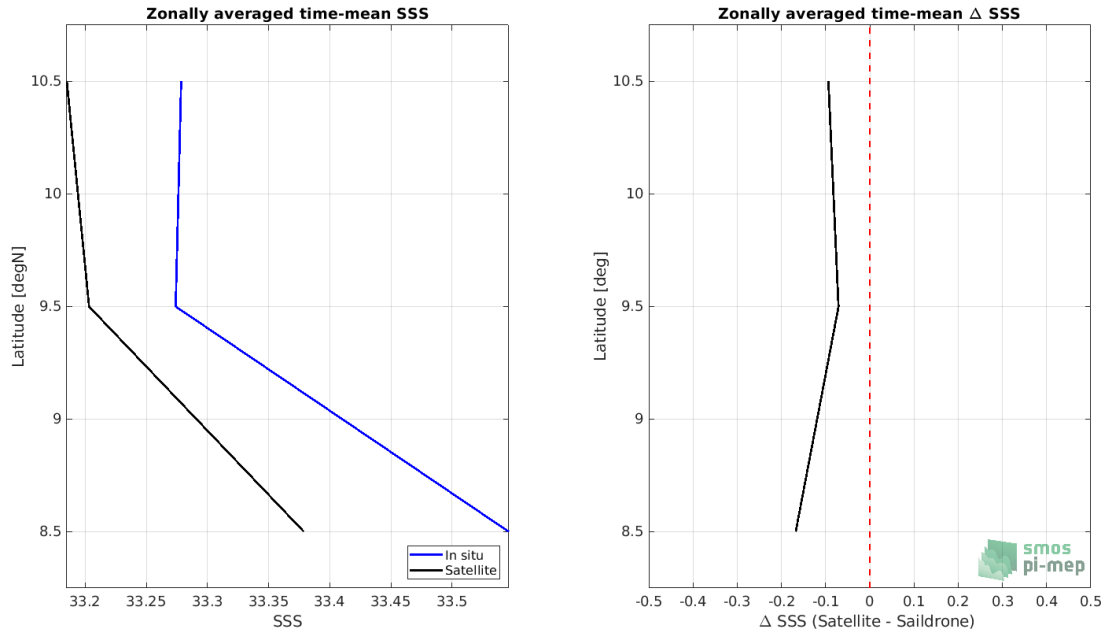
Figure 7: Left panel: Zonal mean SSS from SMAP SSS L3 v4 - Monthly (RSS) satellite product (black) and from Sairdrone (blue). Right panel: Zonal mean of \Delta SSS (Satellite - Sairdrone) for all the collected Pi-MEP match-up pairs estimated over the full satellite product period.
