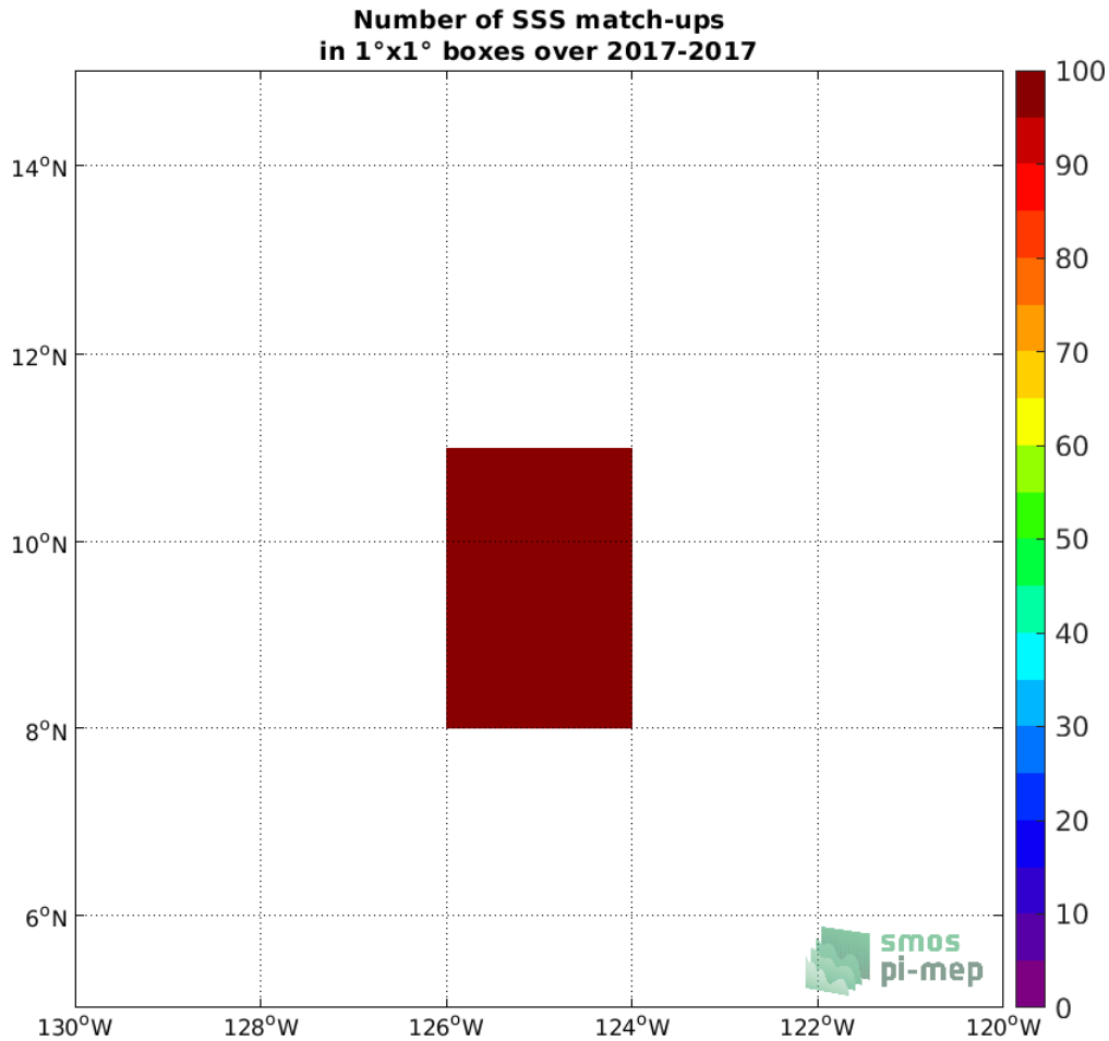
Figure 3: Number of SSS match-ups between Sairdrone SSS and the SMAP SSS L3 v4 - Monthly (RSS) SSS product for the SPURS 2 Pi-MEP region over 1^\circ \times 1^\circ boxes and for the full satellite product period.
