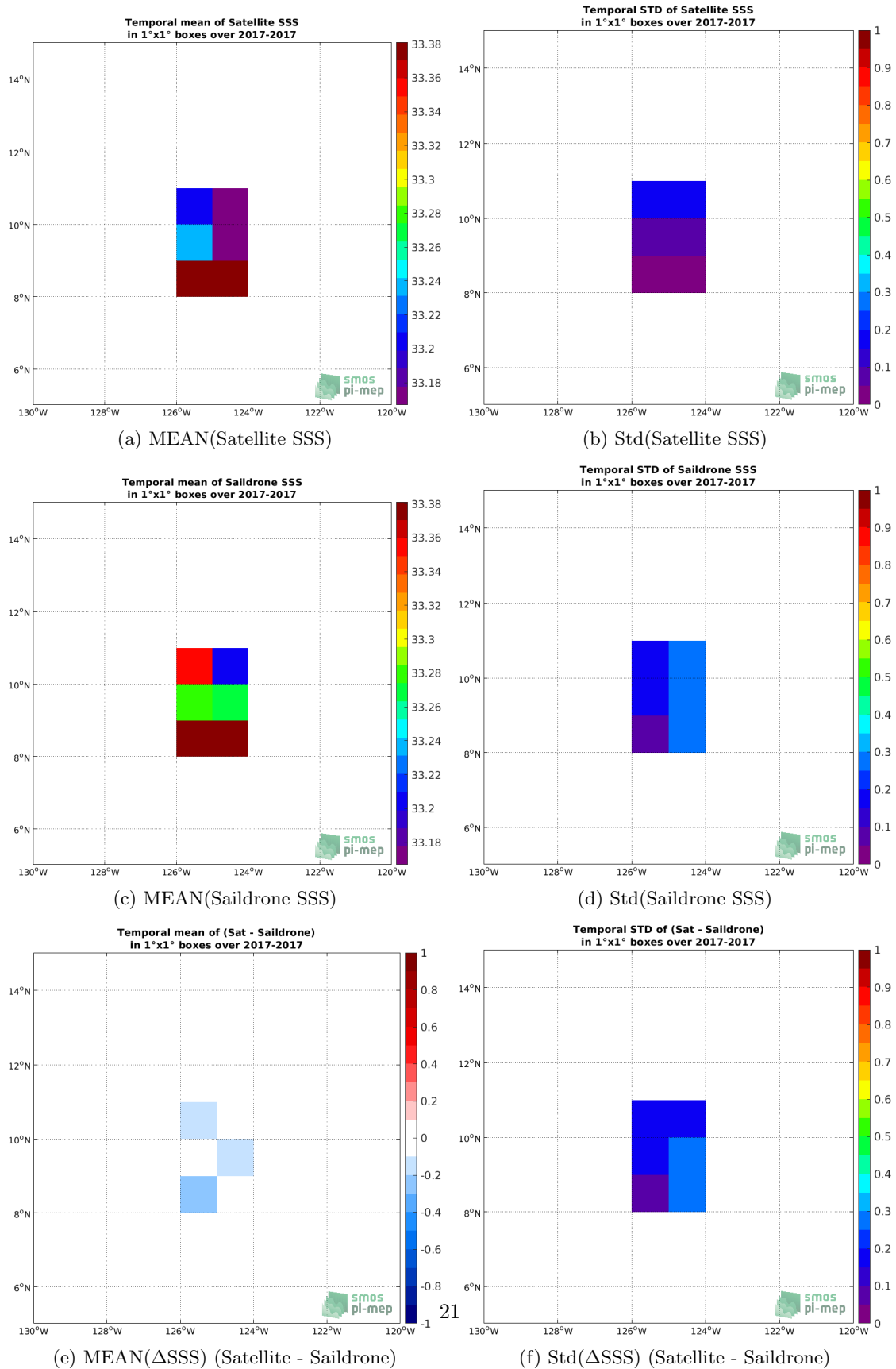
Figure 5: Temporal mean (left) and Std (right) of SSS from SMAP SSS L3 v4 - Monthly (RSS) (top), Saildrone (middle), and of \Delta SSS (Satellite - Saildrone). Only match-up pairs are used to generate these maps.
