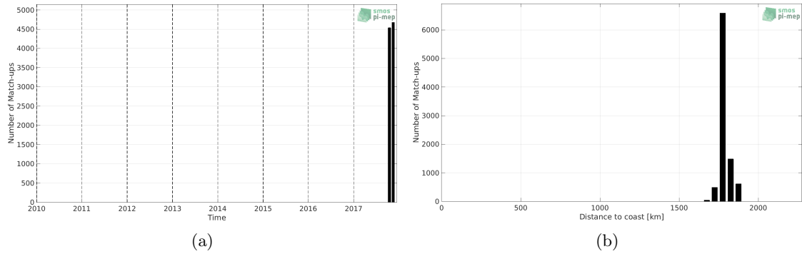
Figure 1: Number of match-ups between Saildrone and SMAP SSS L3 v4 - Monthly (RSS) SSS as a function of time (a) and as function of the distance to coast (b) over the SPURS 2 Pi-MEP region and for the full satellite product period.
