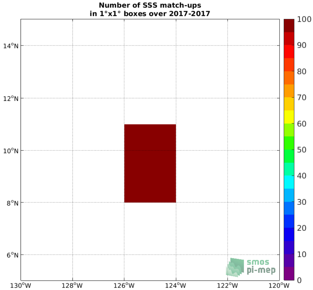
Figure 4: Number of SSS match-ups between Sairdrone SSS and the SMAP SSS L3 v4 - Monthly (RSS) SSS product for the SPURS 2 Pi-MEP region over 1°x1° boxes and for the full satellite product period.
