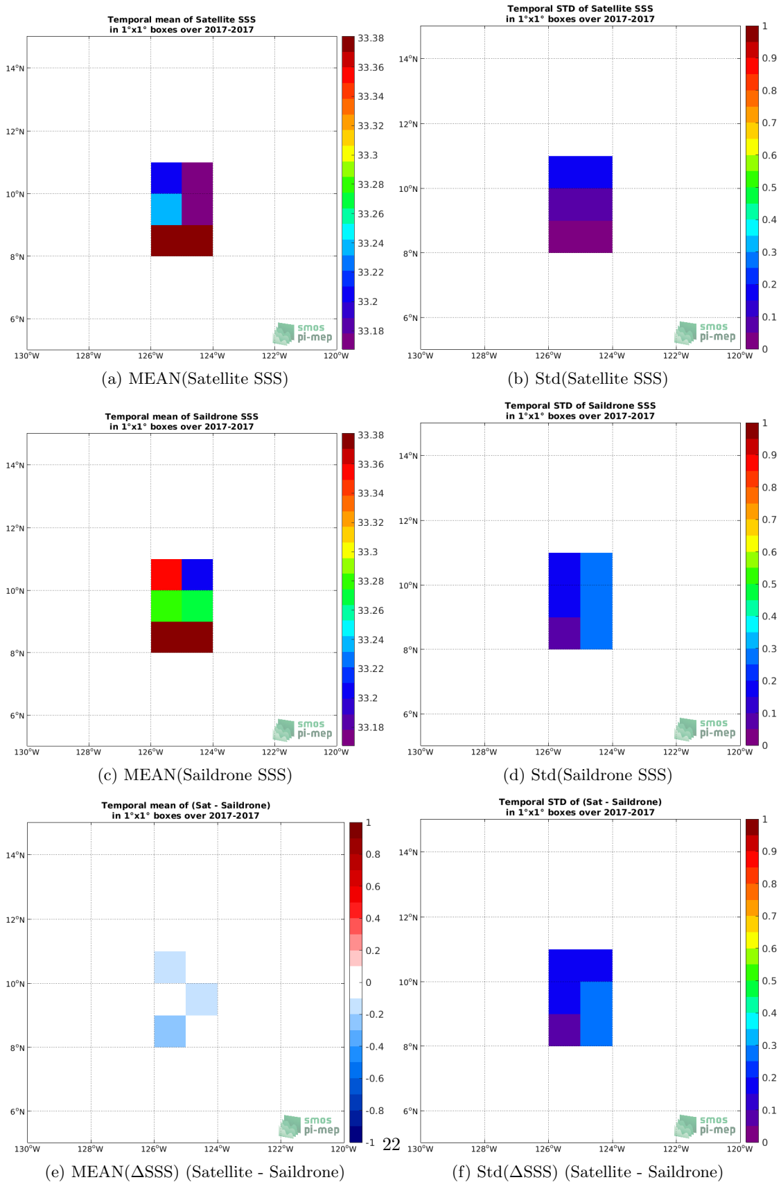
Figure 6: Temporal mean (left) and Std (right) of SSS from SMAP SSS L3 v4 - Monthly (RSS) (top), Saildrone (middle), and of \Delta SSS (Satellite - Saildrone). Only match-up pairs are used to generate these maps.
