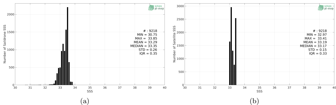
Figure 2: Histograms of SSS from Saildrone (a) and SMAP SSS L3 v4 - Monthly (RSS) (b) considering all match-up pairs per bins of 0.1 over the SPURS 2 Pi-MEP region and for the full satellite product period.
