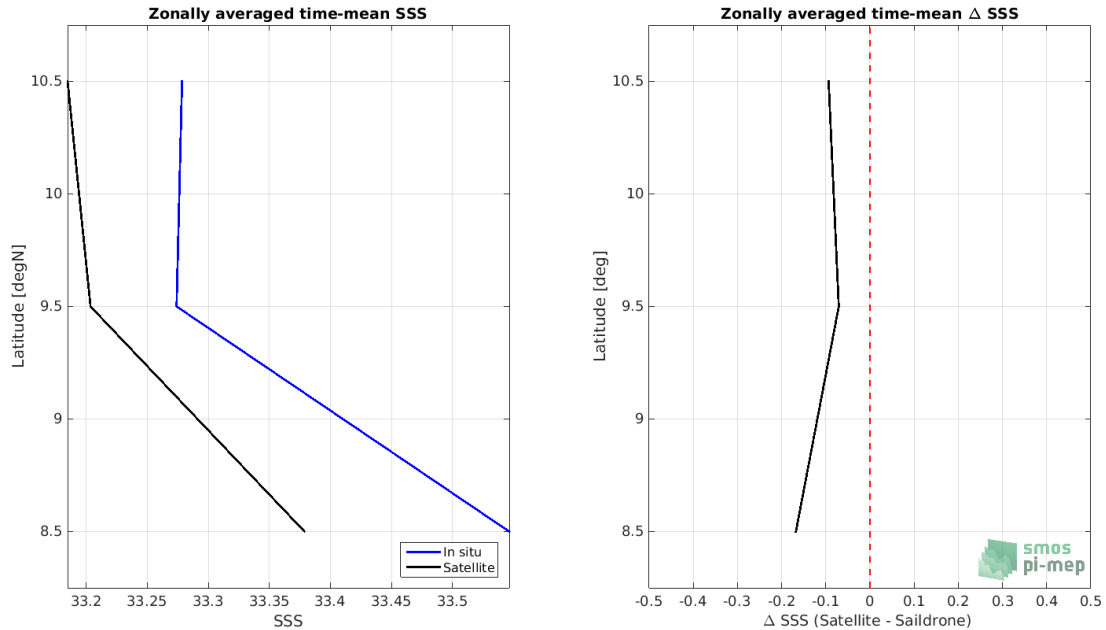
Figure 8: Left panel: Zonal mean SSS from SMAP SSS L3 v4 - Monthly (RSS) satellite product (black) and from Sairdrone (blue). Right panel: Zonal mean of \Delta SSS (Satellite - Sairdrone) for all the collected Pi-MEP match-up pairs estimated over the full satellite product period.
