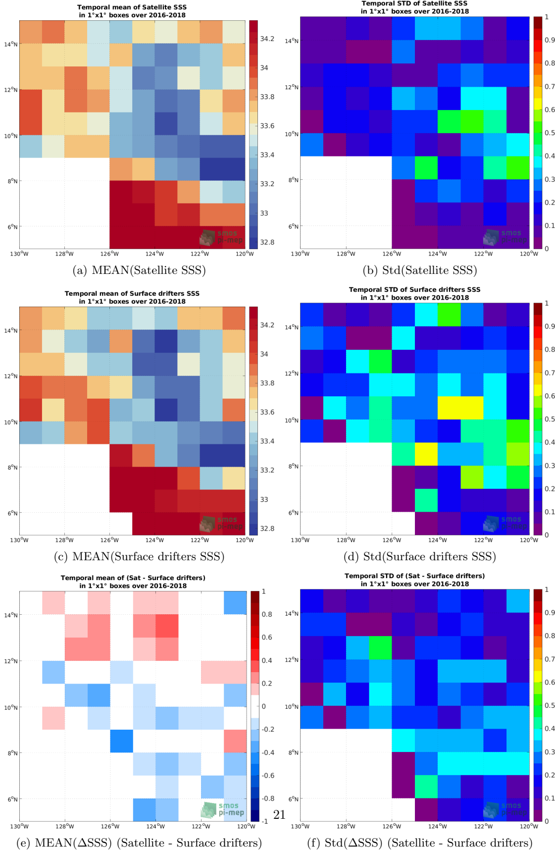
Figure 5: Temporal mean (left) and Std (right) of SSS from SMAP SSS L3 v4 - Monthly (RSS) (top), Surface drifters (middle), and of \Delta SSS (Satellite - Surface drifters). Only match-up pairs are used to generate these maps.
