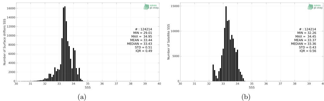
Figure 2: Histograms of SSS from Surface drifters (a) and SMAP SSS L3 v4 - Monthly (RSS) (b) considering all match-up pairs per bins of 0.1 over the SPURS 2 Pi-MEP region and for the full satellite product period.
