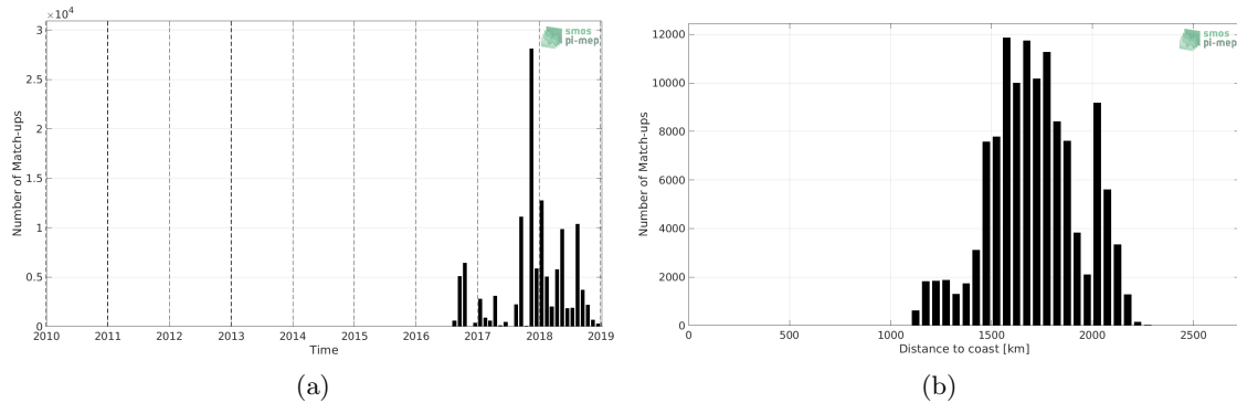
Figure 1: Number of match-ups between Surface drifters and SMAP SSS L3 v4 - Monthly (RSS) SSS as a function of time (a) and as function of the distance to coast (b) over the SPURS 2 Pi-MEP region and for the full satellite product period.
