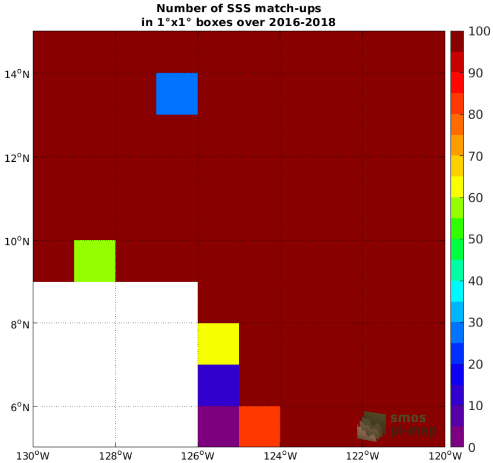
Figure 3: Number of SSS match-ups between Surface drifters SSS and the SMAP SSS L3 v4 - Monthly (RSS) SSS product for the SPURS 2 Pi-MEP region over 1°x1° boxes and for the full satellite product period.
