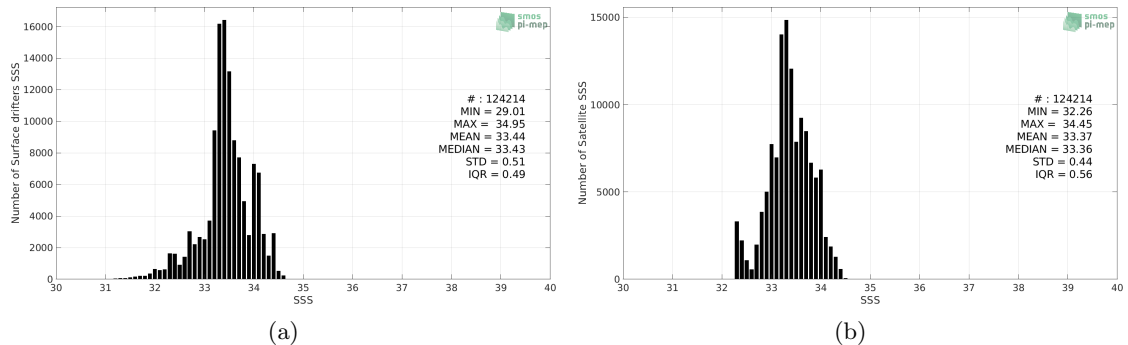
Figure 2: Histograms of SSS from Surface drifters (a) and SMAP SSS L3 v4 - Monthly (RSS) (b) considering all match-up pairs per bins of 0.1 over the SPURS 2 Pi-MEP region and for the full satellite product period.
