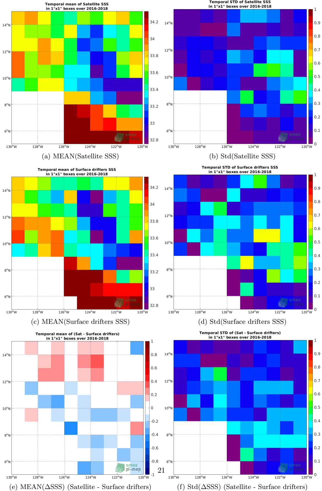
Figure 5: Temporal mean (left) and Std (right) of SSS from SMAP SSS L3 v4 - Monthly (RSS) (top), Surface drifters (middle), and of \Delta SSS (Satellite - Surface drifters). Only match-up pairs are used to generate these maps.
