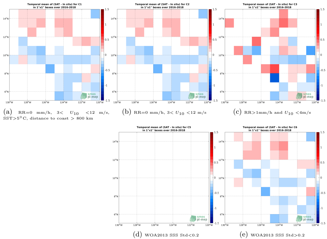
Figure 11: Temporal mean gridded over spatial boxes of size 1^\circ \times 1^\circ of \Delta SSS (SMAP SSS L3 v4 - Monthly (RSS) - Surface drifters) for 5 different subdatasets corresponding to:RR=0 mm/h, 3 < U_{10} < 12 m/s, SST >5^\circ C, distance to coast > 800 km (a), RR=0 mm/h, 3 < U_{10} < 12 m/s (b), RR >1 mm/h and U_{10} < 4 m/s (c), WOA2013 SSS Std <0.2 (d), WOA2013 SSS Std >0.2 (e).
