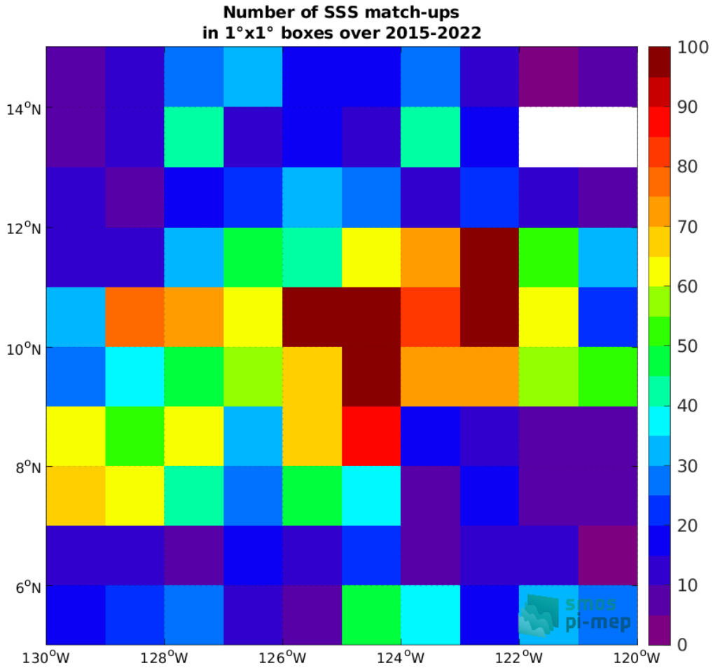
Figure 4: Number of SSS match-ups between Argo SSS and the SMAP SSS L3 v4 - Monthly (RSS) SSS product for the SPURS 2 Pi-MEP region over 1°x1° boxes and for the full satellite product period.
