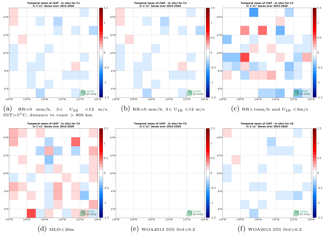
Figure 12: Temporal mean gridded over spatial boxes of size 1^\circ \times 1^\circ of \Delta SSS (SMAP SSS L3 v4 - Monthly (RSS) - Argo) for 6 different subdatasets corresponding to:RR=0 mm/h, 3 < U_{10} < 12 m/s, SST>5°C, distance to coast > 800 km (a), RR=0 mm/h, 3 < U_{10} < 12 m/s (b), RR>1mm/h and U_{10} < 4 m/s (c),MLD<20m (d),WOA2013 SSS Std<0.2 (e),WOA2013 SSS Std>0.2 (f).
