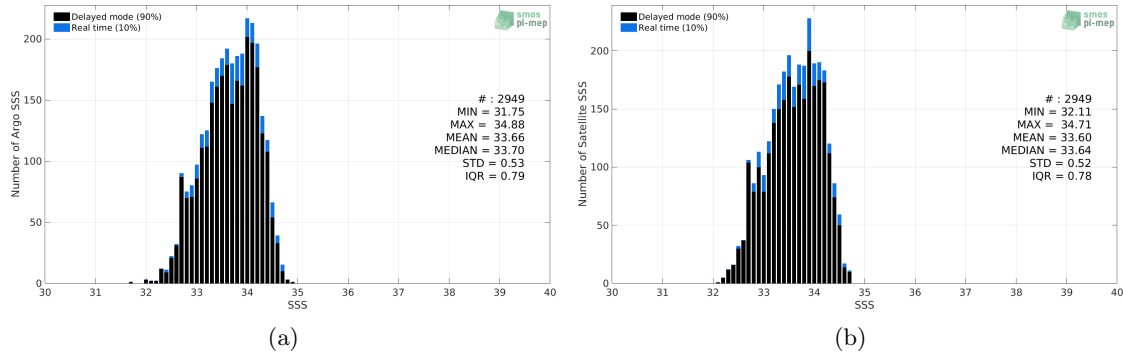
Figure 2: Histograms of SSS from Argo (a) and SMAP SSS L3 v4 - Monthly (RSS) (b) considering all match-up pairs per bins of 0.1 over the SPURS 2 Pi-MEP region and for the full satellite product period.
