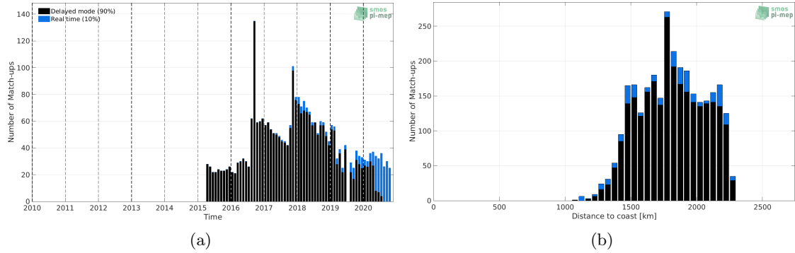
Figure 1: Number of match-ups between Argo and SMAP SSS L3 v4 - Monthly (RSS) SSS as a function of time (a) and as function of the distance to coast (b) over the SPURS 2 Pi-MEP region and for the full satellite product period.
