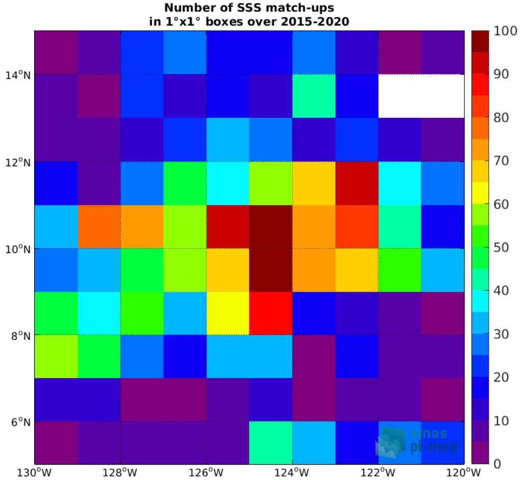
Figure 4: Number of SSS match-ups between Argo SSS and the SMAP SSS L3 v4 - Monthly (RSS) SSS product for the SPURS 2 Pi-MEP region over 1°x1° boxes and for the full satellite product period.
