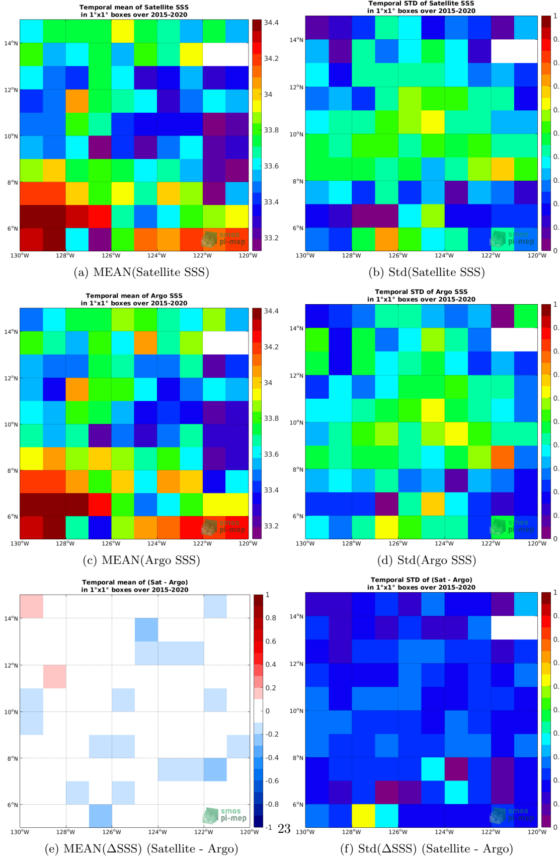
Figure 6: Temporal mean (left) and Std (right) of SSS from SMAP SSS L3 v4 - Monthly (RSS) (top), Argo (middle), and of \Delta SSS (Satellite - Argo). Only match-up pairs are used to generate these maps.
