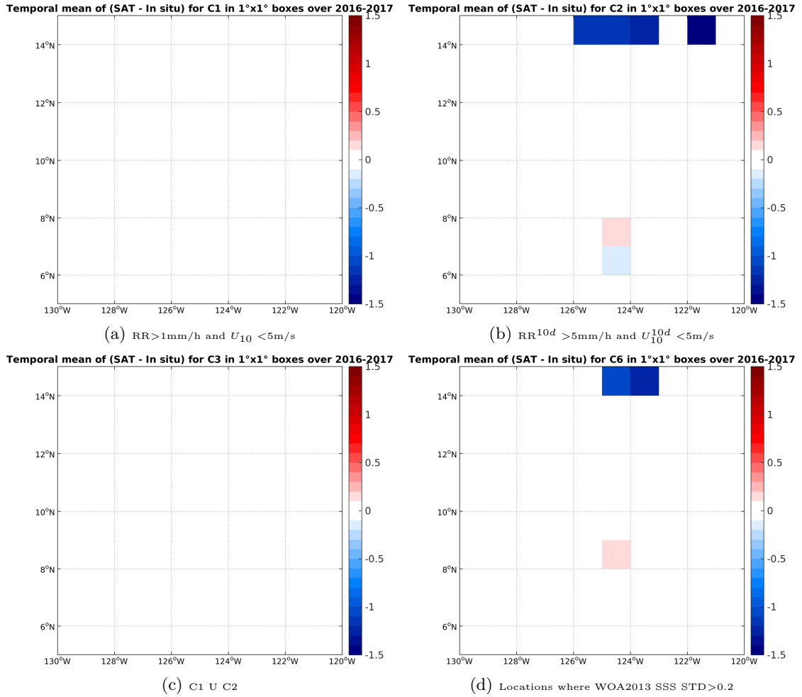
Figure 12: Temporal mean gridded over spatial boxes of size 1°x1° of \Delta SSS (SMAP-L3-RSS-V2-8DAY-RUNNING-40KM - TSG-SAMOS) for 4 different subdatasets corresponding to: RR > 1mm/h and U 10 < 5m/s (a), RR 10d > 5mm/h and U 10 10d < 5m/s (b), C1 U C2 (c), Locations where WOA2013 SSS STD > 0.2 (d).
