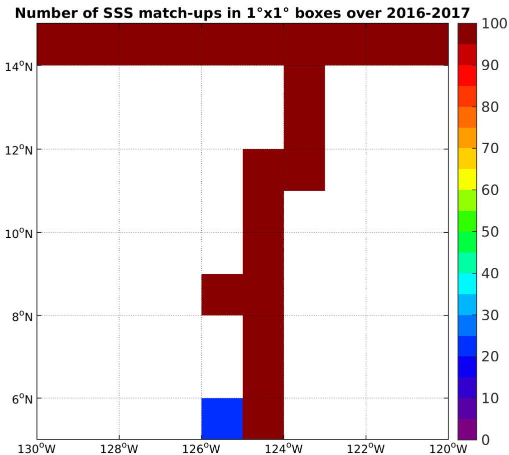
Figure 4: Number of SSS match-ups between TSG-SAMOS SSS and the SMAP-L3-RSS-V2-8DAY-RUNNING-40KM SSS product for the SPURS 2 Pi-MEP region over 1°x1° boxes and for the full satellite product period.
