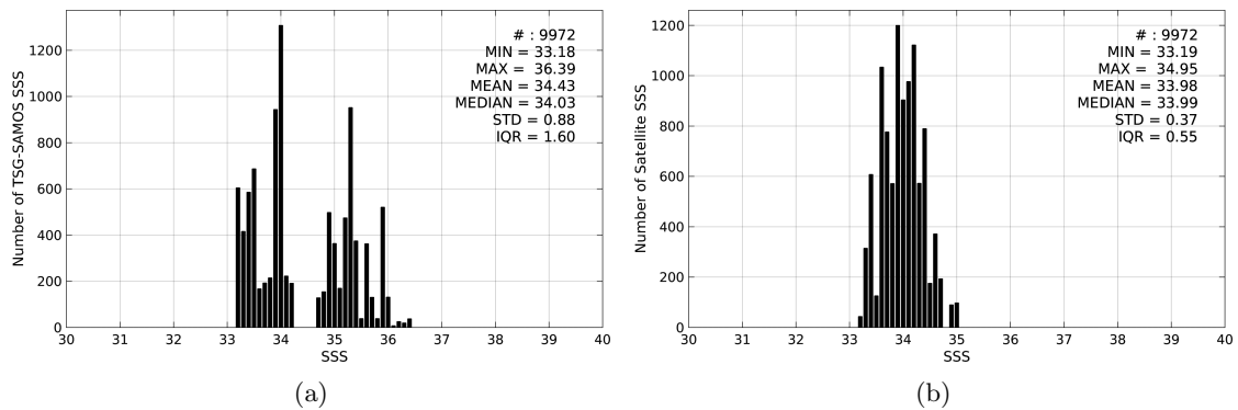
Figure 2: Histograms of SSS from TSG-SAMOS (a) and SMAP-L3-RSS-V2-8DAY-RUNNING-40KM (b) considering all match-up pairs per bins of 0.1 over the SPURS 2 Pi-MEP region and for the full satellite product period.
