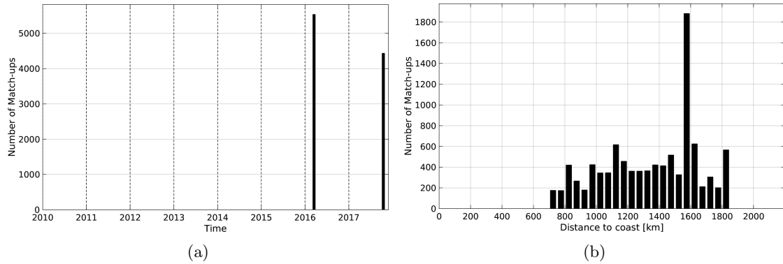
Figure 1: Number of match-ups between TSG-SAMOS and SMAP-L3-RSS-V2-8DAY-RUNNING-40KM SSS as a function of time (a) and as function of the distance to coast (b) over the SPURS 2 Pi-MEP region and for the full satellite product period.
