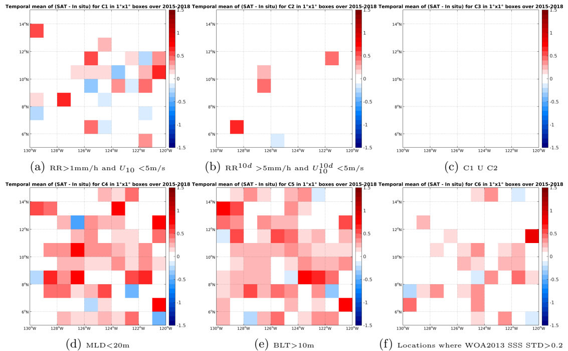
Figure 12: Temporal mean gridded over spatial boxes of size 1^\circ \times 1^\circ of \Delta SSS (SMAP-L3-RSS-V2-8DAY-RUNNING-40KM - Argo) for 6 different subdatasets corresponding to: RR > 1\text{mm/h} and U_{10} < 5\text{m/s} (a), RR^{10d} > 5\text{mm/h} and U_{10}^{10d} < 5\text{m/s} (b), C1 U C2 (c), MLD < 20\text{m} (d), BLT > 10\text{m} (e), Locations where WOA2013 SSS STD > 0.2 (f).
