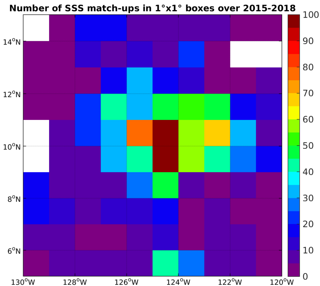
Figure 4: Number of SSS match-ups between Argo SSS and the SMAP-L3-RSS-V2-8DAY-RUNNING-40KM SSS product for the SPURS 2 Pi-MEP region over 1°x1° boxes and for the full satellite product period.
