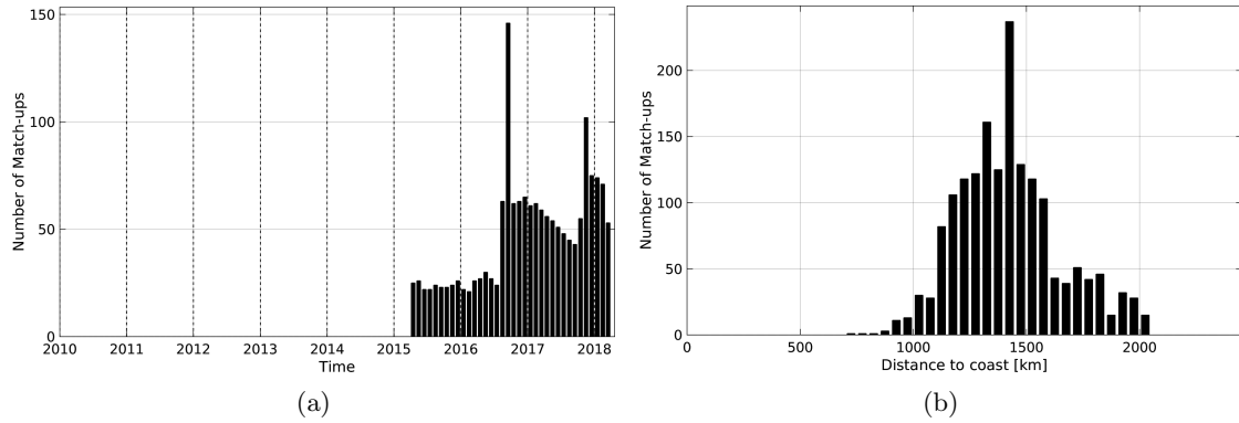
Figure 1: Number of match-ups between Argo and SMAP-L3-RSS-V2-8DAY-RUNNING-40KM SSS as a function of time (a) and as function of the distance to coast (b) over the SPURS 2 Pi-MEP region and for the full satellite product period.
