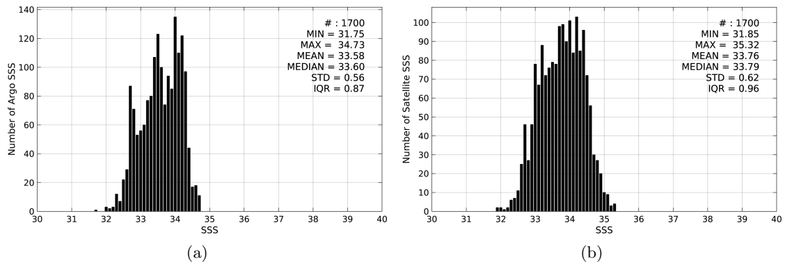
Figure 2: Histograms of SSS from Argo (a) and SMAP-L3-RSS-V2-8DAY-RUNNING-40KM (b) considering all match-up pairs per bins of 0.1 over the SPURS 2 Pi-MEP region and for the full satellite product period.
