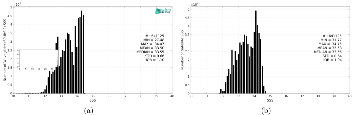
Figure 3: Histograms of SSS from Waveglider (SPURS 2) (a) and SMAP SSS L3 v5.0 - 8-Day running (JPL) (b) considering all match-up pairs per bins of 0.1 over the SPURS 2 Pi-MEP region and for the full satellite product period.
