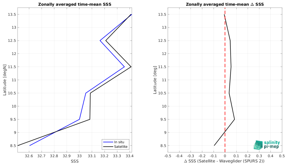
Figure 9: Left panel: Zonal mean SSS from SMAP SSS L3 v5.0 - 8-Day running (JPL) satellite product (black) and from Waveglider (SPURS 2) (blue). Right panel: Zonal mean of \Delta SSS (Satellite - Waveglider (SPURS 2)) for all the collected Pi-MEP match-up pairs estimated over the full satellite product period.
