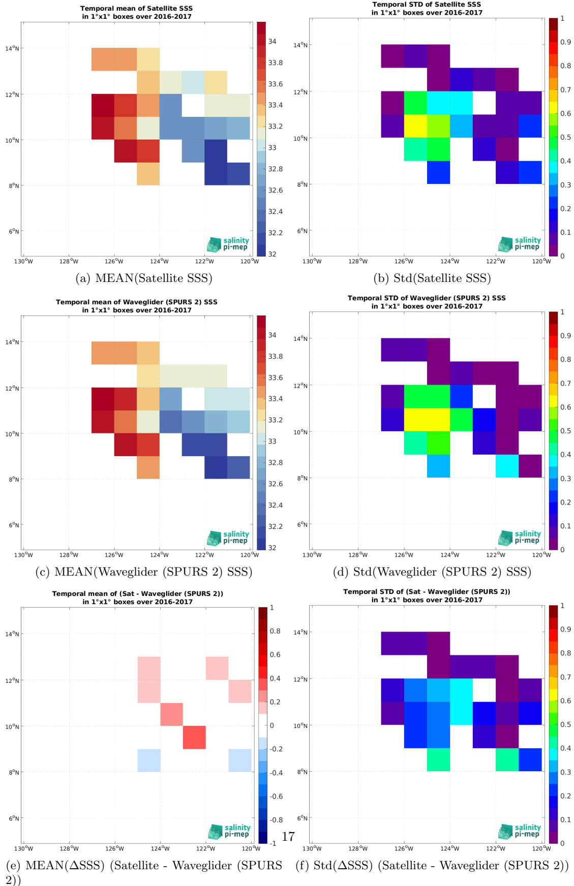
Figure 7: Temporal mean (left) and Std (right) of SSS from SMAP SSS L3 v5.0 - 8-Day running (JPL) (top), Waveglider (SPURS 2) (middle), and of \Delta SSS (Satellite - Waveglider (SPURS 2)). Only match-up pairs are used to generate these maps.
