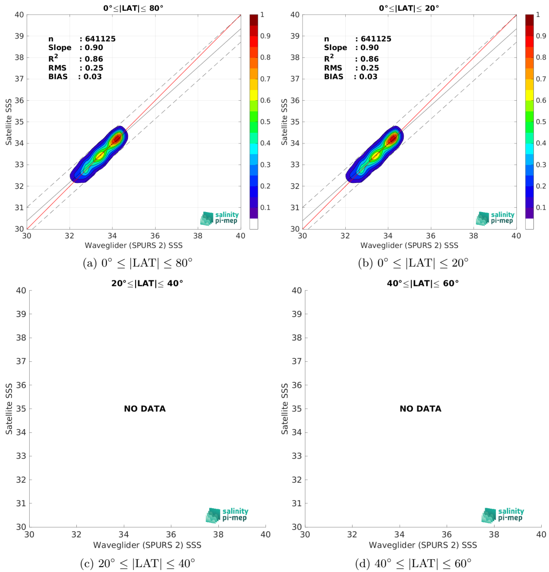
Figure 10: Contour maps of the concentration of SMAP SSS L3 v5.0 - 8-Day running (JPL) SSS (y-axis) versus Waveglider (SPURS 2) SSS (x-axis) at match-up pairs for different latitude bands. For each plot, the red line shows x=y . The black thin and dashed lines indicate a linear fit through the data cloud and the \pm 95\% confidence levels, respectively. The number match-up pairs n , the slope and R^2 coefficient of the linear fit, the root mean square (RMS) and the mean bias between satellite and in situ data are indicated for each latitude band in each plots.
