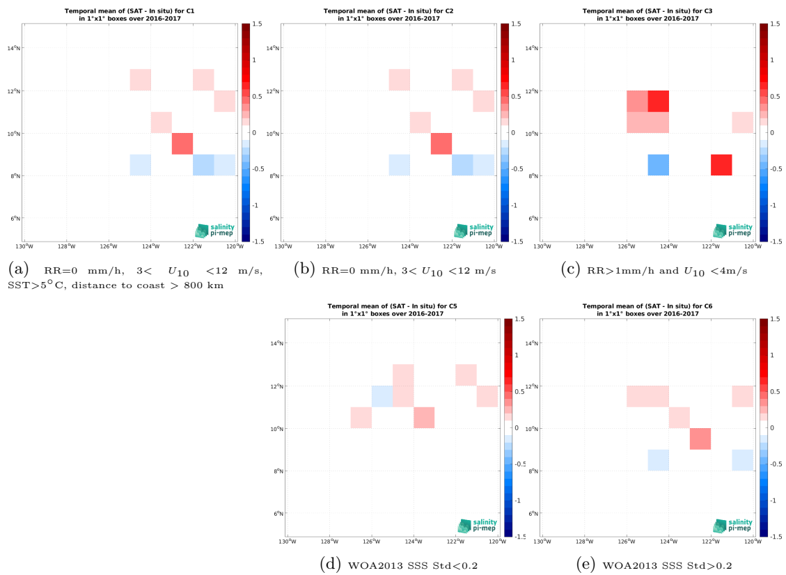
Figure 14: Temporal mean gridded over spatial boxes of size 1^\circ \times 1^\circ of \Delta SSS (SMAP SSS L3 v5.0 - 8-Day running (JPL) - Waveglider (SPURS 2)) for 5 different subdatasets corresponding to:RR=0 mm/h, 3 < U_{10} < 12 m/s, SST >5^\circ\text{C} , distance to coast > 800 km (a), RR=0 mm/h, 3 < U_{10} < 12 m/s (b), RR >1 mm/h and U_{10} < 4 m/s (c), WOA2013 SSS Std <0.2 (d), WOA2013 SSS Std >0.2 (e).
