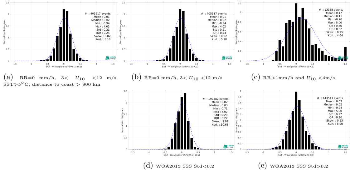
Figure 15: Normalized histogram of \Delta SSS (SMAP SSS L3 v5.0 - 8-Day running (JPL) - Waveglider (SPURS 2)) for 5 different subdatasets corresponding to: RR=0 mm/h, 3 < U_{10} < 12 m/s, SST>5°C, distance to coast > 800 km (a), RR=0 mm/h, 3 < U_{10} < 12 m/s (b), RR>1mm/h and U_{10} < 4 m/s (c), WOA2013 SSS Std<0.2 (d), WOA2013 SSS Std>0.2 (e).
