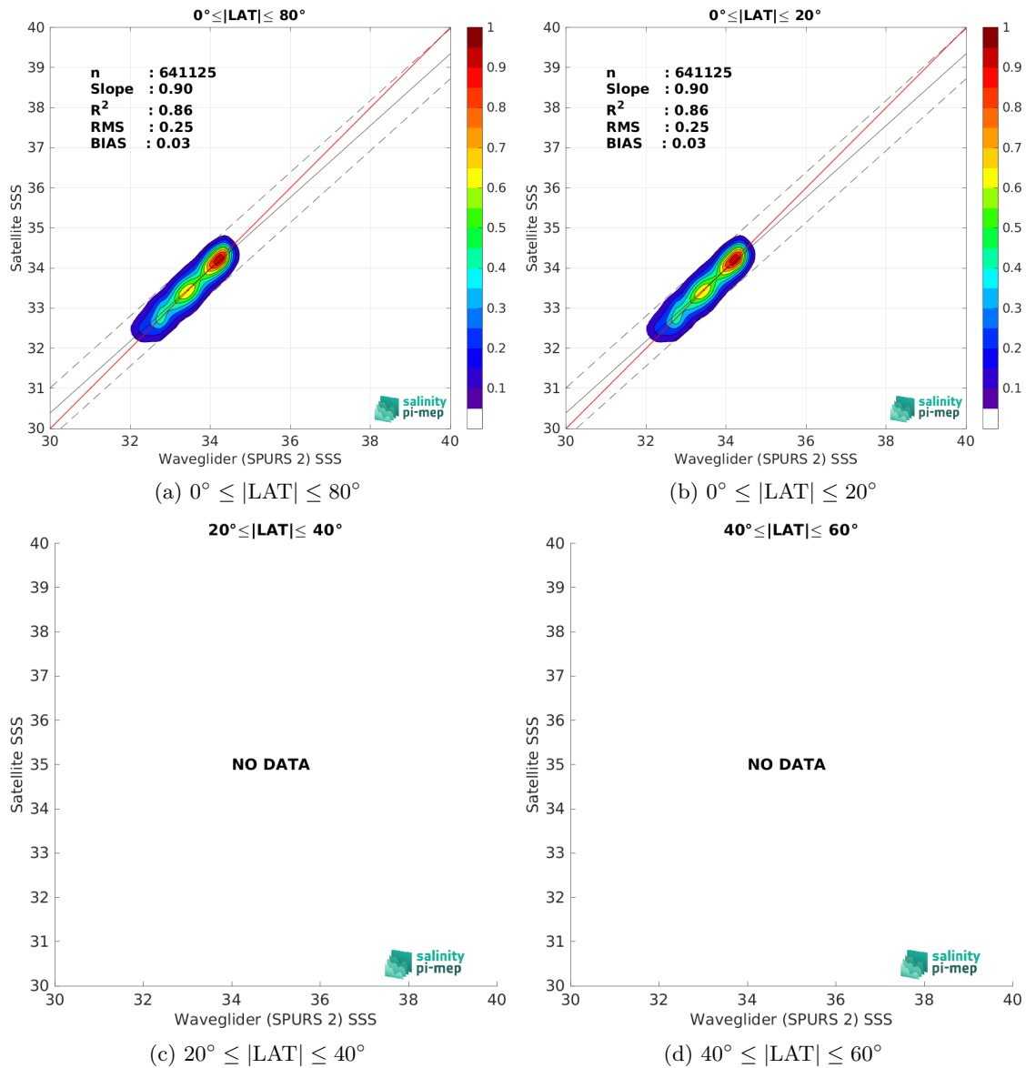
Figure 9: Contour maps of the concentration of SMAP SSS L3 v5.0 - 8-Day running (JPL) SSS (y-axis) versus Waveglider (SPURS 2) SSS (x-axis) at match-up pairs for different latitude bands. For each plot, the red line shows x=y . The black thin and dashed lines indicate a linear fit through the data cloud and the \pm 95\% confidence levels, respectively. The number match-up pairs n , the slope and R^2 coefficient of the linear fit, the root mean square (RMS) and the mean bias between satellite and in situ data are indicated for each latitude band in each plots.
