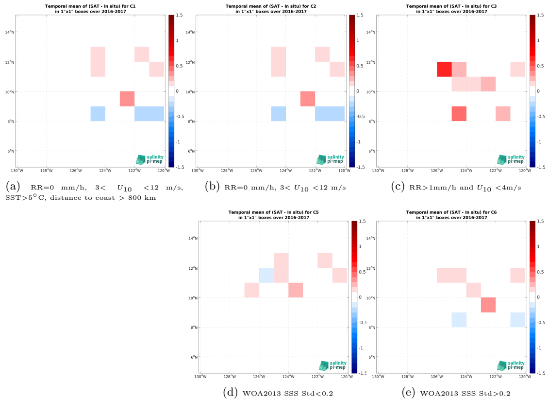
Figure 12: Temporal mean gridded over spatial boxes of size 1^\circ \times 1^\circ of \Delta SSS (SMAP SSS L3 v5.0 - 8-Day running (JPL) - Waveglider (SPURS 2)) for 5 different subdatasets corresponding to: RR=0 mm/h, 3 < U_{10} < 12 m/s, SST > 5^\circ\text{C} , distance to coast > 800 km (a), RR=0 mm/h, 3 < U_{10} < 12 m/s (b), RR > 1 mm/h and U_{10} < 4 m/s (c), WOA2013 SSS Std < 0.2 (d), WOA2013 SSS Std > 0.2 (e).
