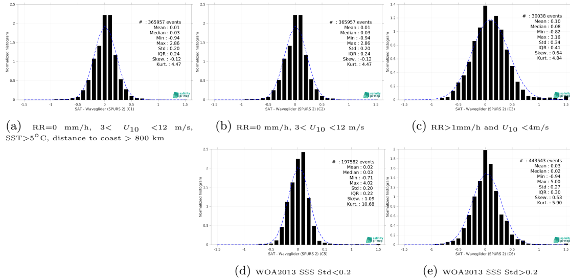
Figure 13: Normalized histogram of \Delta SSS (SMAP SSS L3 v5.0 - 8-Day running (JPL) - Waveglider (SPURS 2)) for 5 different subdatasets corresponding to: RR=0 mm/h, 3 < U_{10} < 12 m/s, SST>5°C, distance to coast > 800 km (a), RR=0 mm/h, 3 < U_{10} < 12 m/s (b), RR>1mm/h and U_{10} < 4 m/s (c), WOA2013 SSS Std<0.2 (d), WOA2013 SSS Std>0.2 (e).
