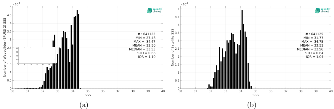
Figure 2: Histograms of SSS from Waveglider (SPURS 2) (a) and SMAP SSS L3 v5.0 - 8-Day running (JPL) (b) considering all match-up pairs per bins of 0.1 over the SPURS 2 Pi-MEP region and for the full satellite product period.
