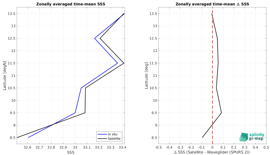
Figure 8: Left panel: Zonal mean SSS from SMAP SSS L3 v5.0 - 8-Day running (JPL) satellite product (black) and from Waveglider (SPURS 2) (blue). Right panel: Zonal mean of \Delta SSS (Satellite - Waveglider (SPURS 2)) for all the collected Pi-MEP match-up pairs estimated over the full satellite product period.
