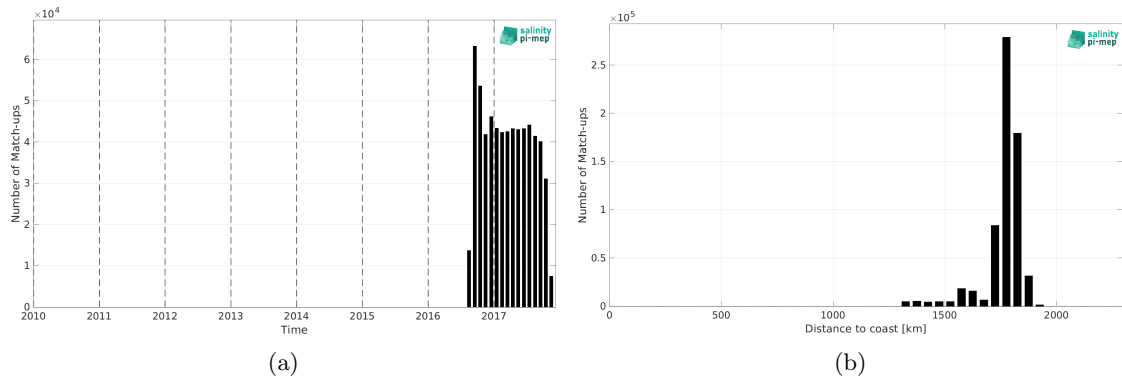
Figure 1: Number of match-ups between Waveglider (SPURS 2) and SMAP SSS L3 v5.0 - 8-Day running (JPL) SSS as a function of time (a) and as function of the distance to coast (b) over the SPURS 2 Pi-MEP region and for the full satellite product period.
