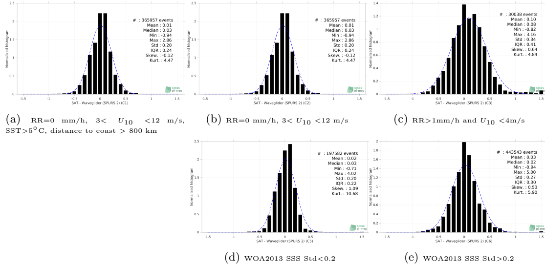
Figure 13: Normalized histogram of \Delta SSS (SMAP SSS L3 v5.0 - 8-Day running (JPL) - Waveglider (SPURS 2)) for 5 different subdatasets corresponding to: RR=0 mm/h, 3 < U_{10} < 12 m/s, SST > 5°C, distance to coast > 800 km (a), RR=0 mm/h, 3 < U_{10} < 12 m/s (b), RR > 1mm/h and U_{10} < 4 m/s (c), WOA2013 SSS Std < 0.2 (d), WOA2013 SSS Std > 0.2 (e).
