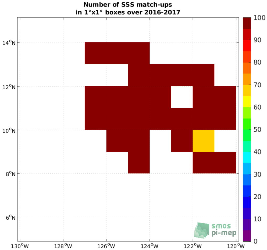
Figure 4: Number of SSS match-ups between Waveglider (SPURS 2) SSS and the SMAP SSS L3 v5.0 - 8-Day running (JPL) SSS product for the SPURS 2 Pi-MEP region over 1^\circ \times 1^\circ boxes and for the full satellite product period.
