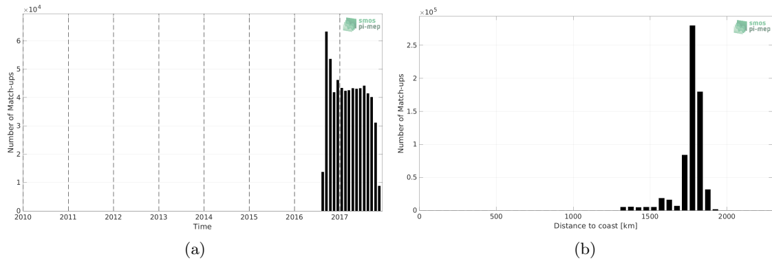
Figure 1: Number of match-ups between Waveglider and SMAP SSS L3 v5.0 - 8-Day running (JPL) SSS as a function of time (a) and as function of the distance to coast (b) over the SPURS 2 Pi-MEP region and for the full satellite product period.
