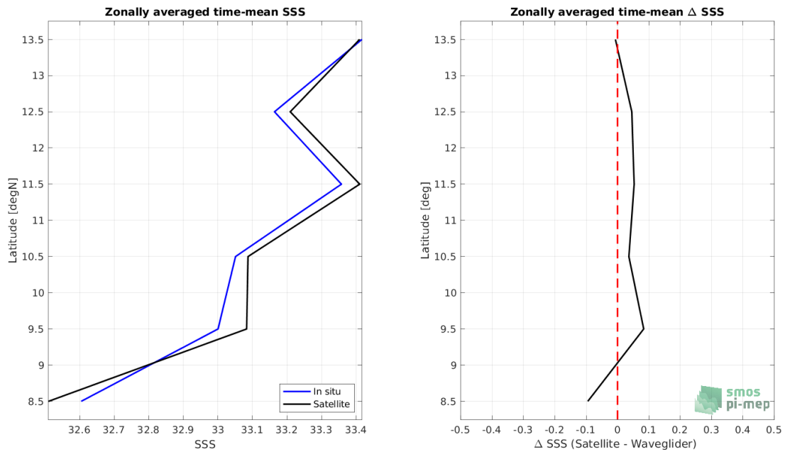
Figure 8: Left panel: Zonal mean SSS from SMAP SSS L3 v5.0 - 8-Day running (JPL) satellite product (black) and from Waveglider (blue). Right panel: Zonal mean of \Delta SSS (Satellite - Waveglider) for all the collected Pi-MEP match-up pairs estimated over the full satellite product period.
