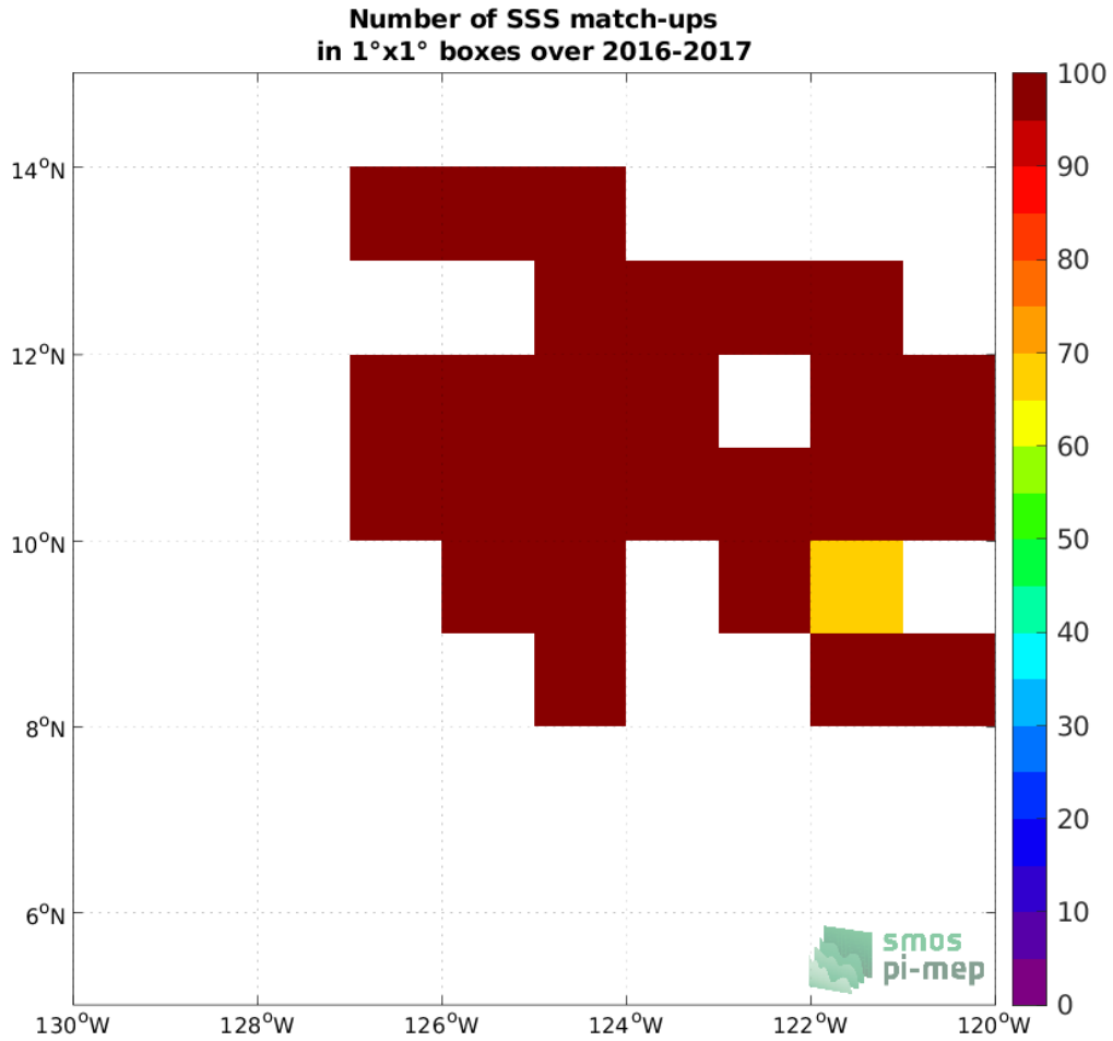
Figure 4: Number of SSS match-ups between Waveglider SSS and the SMAP SSS L3 v5.0 - 8-Day running (JPL) SSS product for the SPURS 2 Pi-MEP region over 1°x1° boxes and for the full satellite product period.
