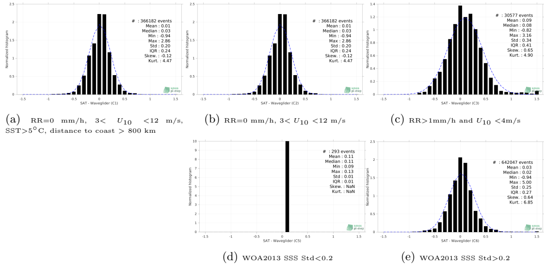
Figure 13: Normalized histogram of \Delta SSS (SMAP SSS L3 v5.0 - 8-Day running (JPL) - Waveglider) for 5 different subdatasets corresponding to: RR=0 mm/h, 3 < U_{10} < 12 m/s, SST > 5°C, distance to coast > 800 km (a), RR=0 mm/h, 3 < U_{10} < 12 m/s (b), RR > 1mm/h and U_{10} < 4 m/s (c), WOA2013 SSS Std < 0.2 (d), WOA2013 SSS Std > 0.2 (e).
