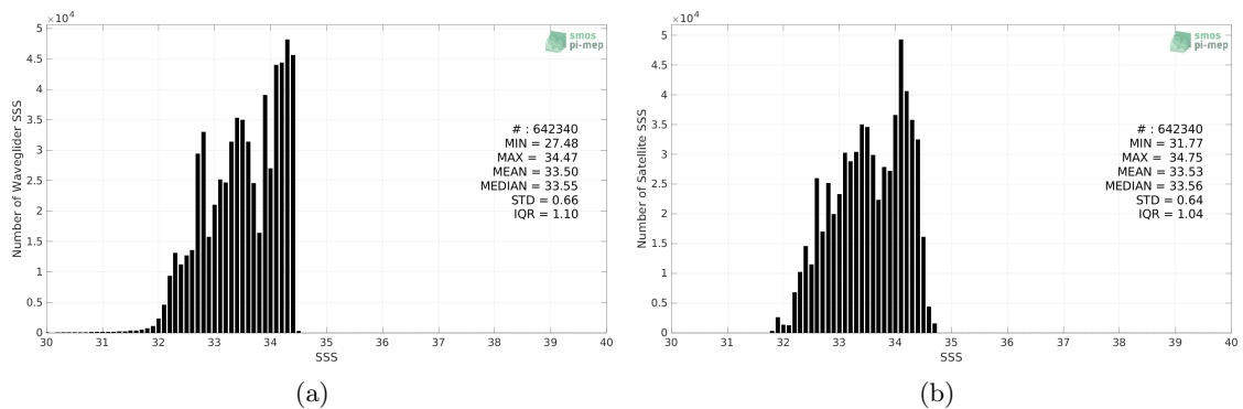
Figure 2: Histograms of SSS from Waveglider (a) and SMAP SSS L3 v5.0 - 8-Day running (JPL) (b) considering all match-up pairs per bins of 0.1 over the SPURS 2 Pi-MEP region and for the full satellite product period.
