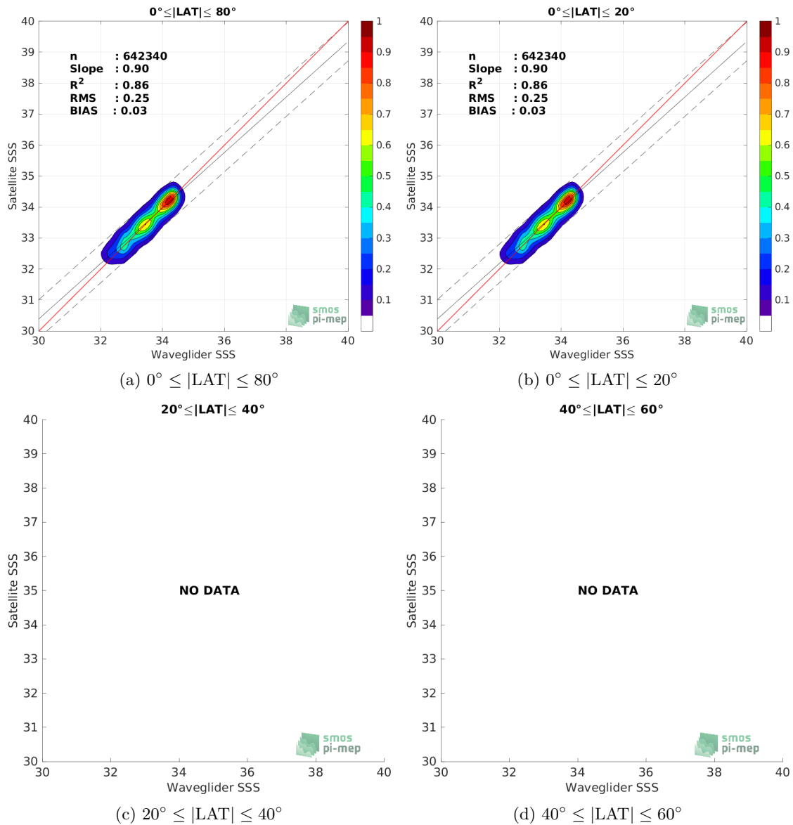
Figure 9: Contour maps of the concentration of SMAP SSS L3 v5.0 - 8-Day running (JPL) SSS (y-axis) versus Waveglider SSS (x-axis) at match-up pairs for different latitude bands. For each plot, the red line shows x=y . The black thin and dashed lines indicate a linear fit through the data cloud and the \pm 95\% confidence levels, respectively. The number match-up pairs n , the slope and R^2 coefficient of the linear fit, the root mean square (RMS) and the mean bias between satellite and in situ data are indicated for each latitude band in each plots.
