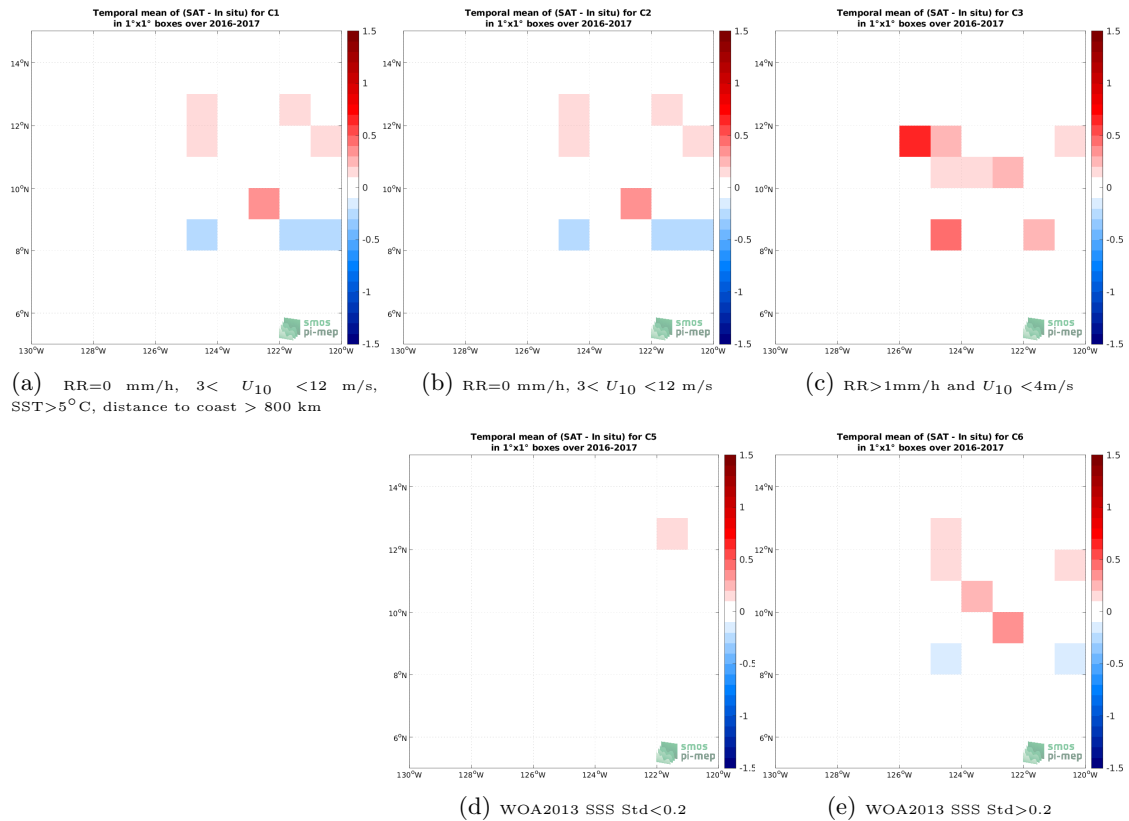
Figure 12: Temporal mean gridded over spatial boxes of size 1^\circ \times 1^\circ of \Delta SSS (SMAP SSS L3 v5.0 - 8-Day running (JPL) - Waveglider) for 5 different subdatasets corresponding to:RR=0 mm/h, 3 < U_{10} < 12 m/s, SST > 5^\circ\text{C} , distance to coast > 800 km (a), RR=0 mm/h, 3 < U_{10} < 12 m/s (b), RR > 1 mm/h and U_{10} < 4 m/s (c), WOA2013 SSS Std < 0.2 (d), WOA2013 SSS Std > 0.2 (e).
