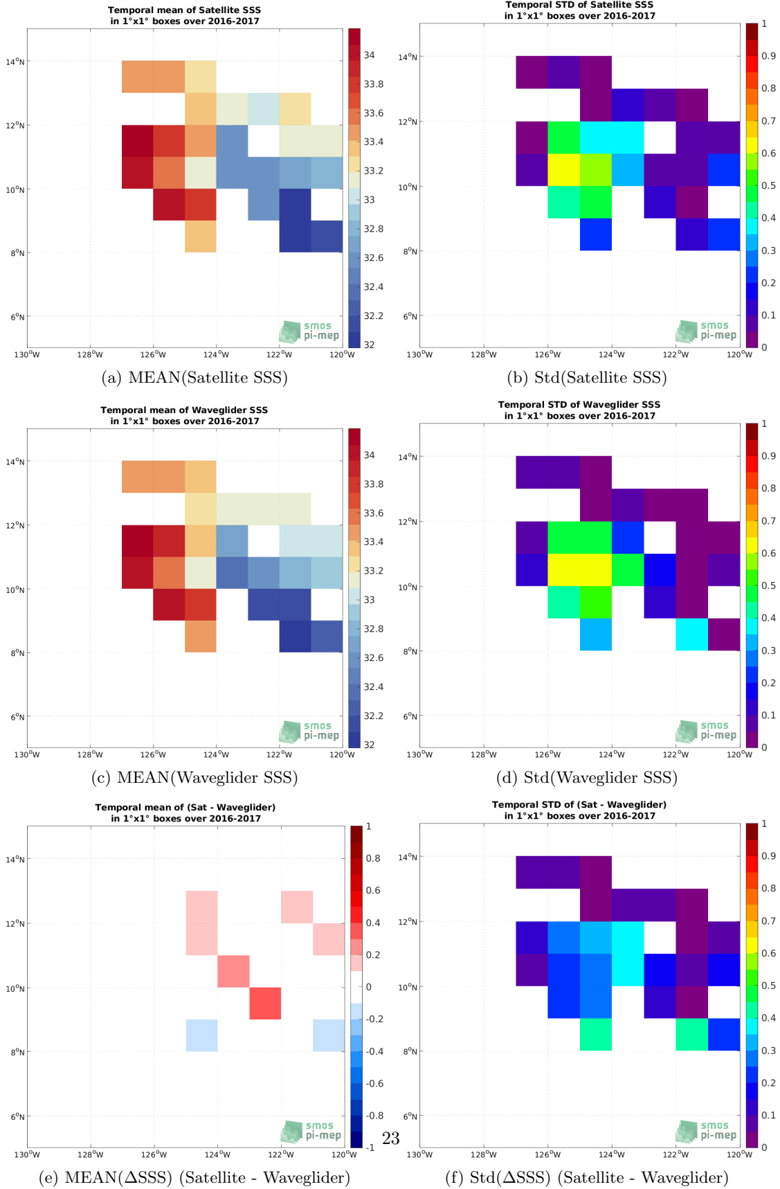
Figure 6: Temporal mean (left) and Std (right) of SSS from SMAP SSS L3 v5.0 - 8-Day running (JPL) (top), Waveglider (middle), and of \Delta SSS (Satellite - Waveglider). Only match-up pairs are used to generate these maps.
