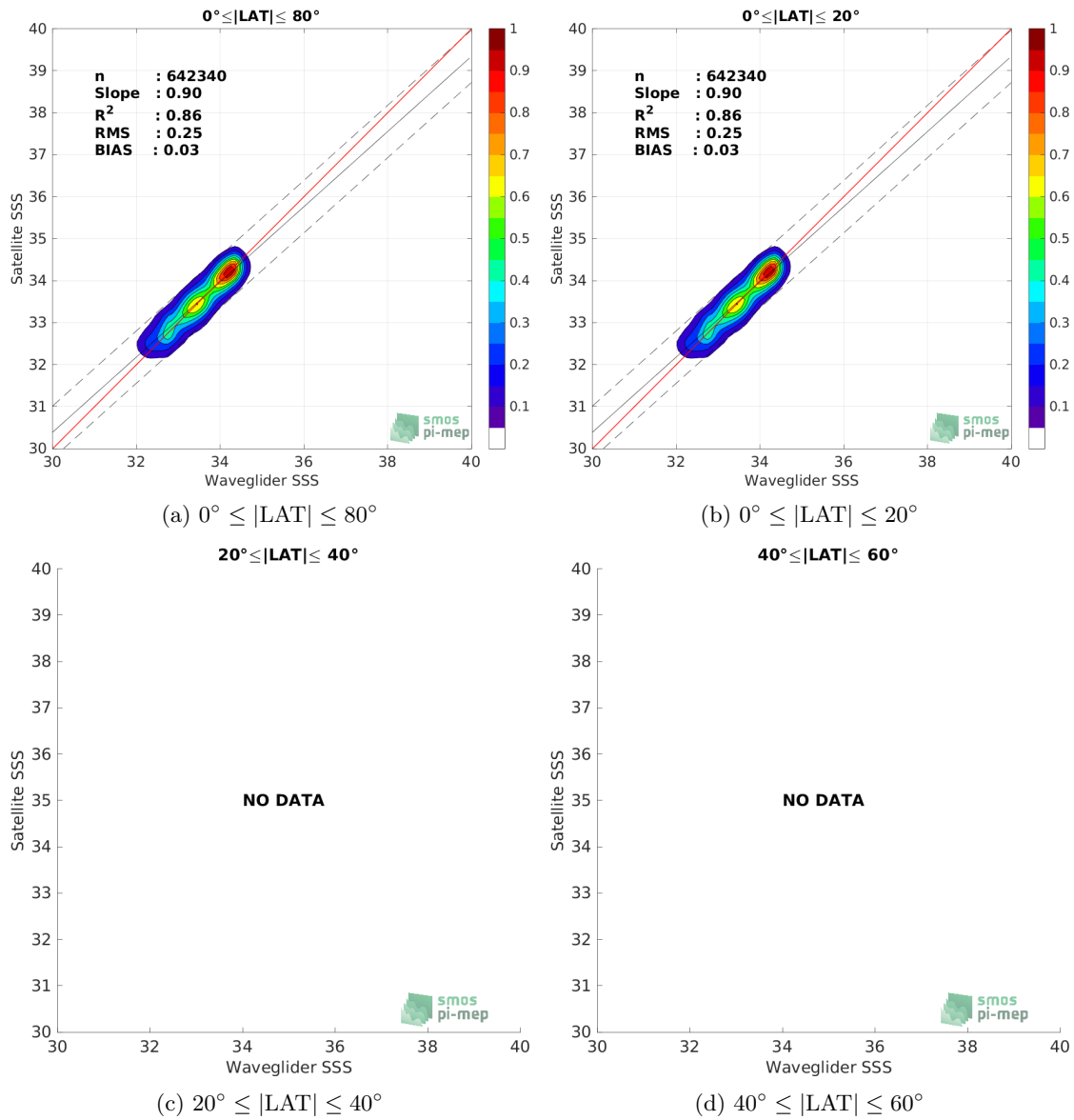
Figure 8: Contour maps of the concentration of SMAP SSS L3 v5.0 - 8-Day running (JPL) SSS (y-axis) versus Waveglider SSS (x-axis) at match-up pairs for different latitude bands. For each plot, the red line shows x=y . The black thin and dashed lines indicate a linear fit through the data cloud and the \pm 95\% confidence levels, respectively. The number match-up pairs n , the slope and R^2 coefficient of the linear fit, the root mean square (RMS) and the mean bias between satellite and in situ data are indicated for each latitude band in each plots.
