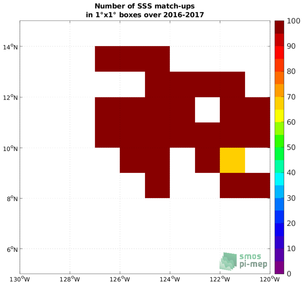
Figure 3: Number of SSS match-ups between Waveglider SSS and the SMAP SSS L3 v5.0 - 8-Day running (JPL) SSS product for the SPURS 2 Pi-MEP region over 1°x1° boxes and for the full satellite product period.
