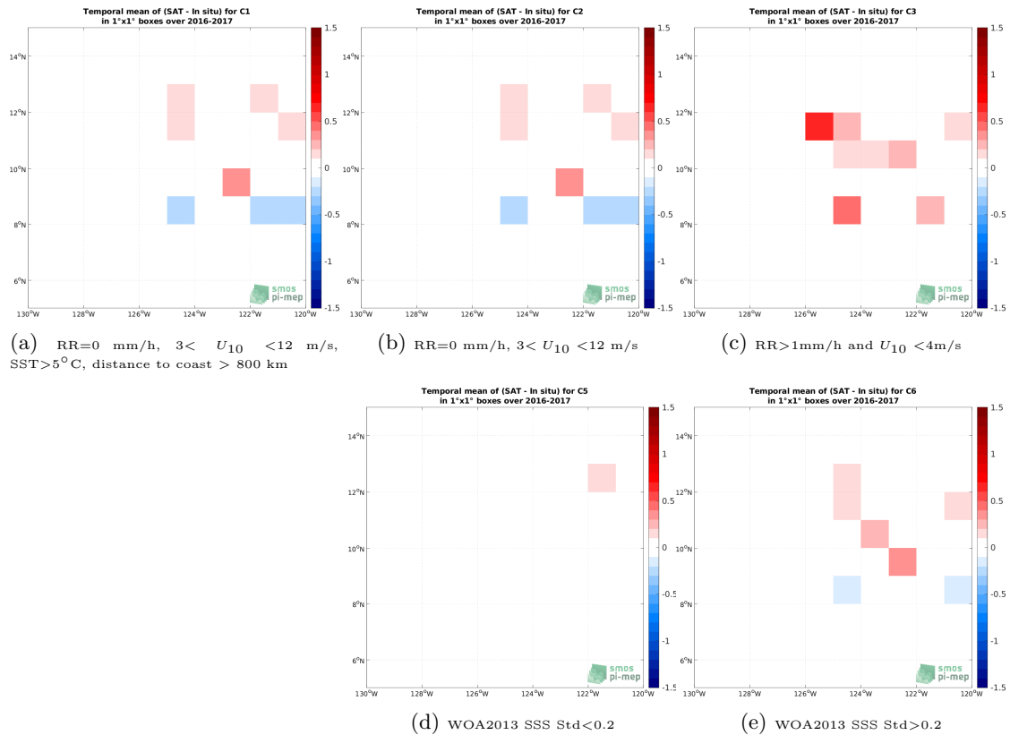
Figure 11: Temporal mean gridded over spatial boxes of size 1^\circ \times 1^\circ of \Delta SSS (SMAP SSS L3 v5.0 - 8-Day running (JPL) - Waveglider) for 5 different subdatasets corresponding to:RR=0 mm/h, 3 < U_{10} < 12 m/s, SST >5^\circ C, distance to coast > 800 km (a), RR=0 mm/h, 3 < U_{10} < 12 m/s (b), RR >1 mm/h and U_{10} < 4 m/s (c), WOA2013 SSS Std <0.2 (d), WOA2013 SSS Std >0.2 (e).
