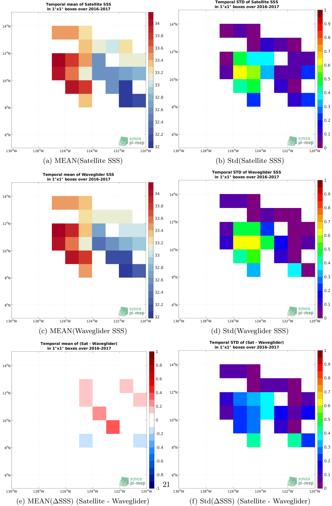
Figure 5: Temporal mean (left) and Std (right) of SSS from SMAP SSS L3 v5.0 - 8-Day running (JPL) (top), Waveglider (middle), and of \Delta SSS (Satellite - Waveglider). Only match-up pairs are used to generate these maps.
