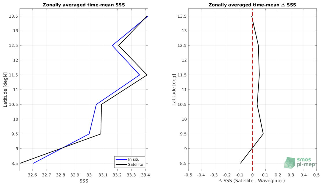
Figure 7: Left panel: Zonal mean SSS from SMAP SSS L3 v5.0 - 8-Day running (JPL) satellite product (black) and from Waveglider (blue). Right panel: Zonal mean of \Delta SSS (Satellite - Waveglider) for all the collected Pi-MEP match-up pairs estimated over the full satellite product period.
