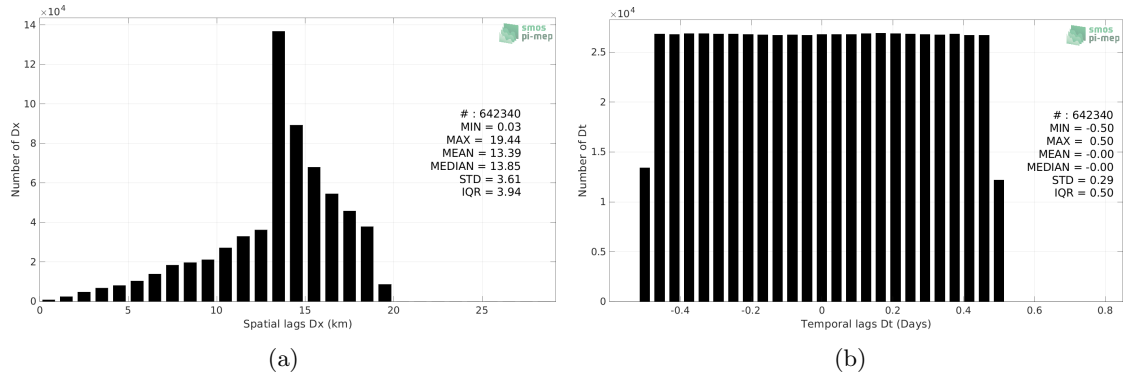
Figure 4: Histograms of the spatial (a) and temporal (b) lags between the location/time of the Waveglider measurement and the date of the corresponding SMAP SSS L3 v5.0 - 8-Day running (JPL) SSS pixel.
