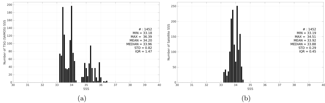
Figure 3: Histograms of SSS from TSG (SAMOS) (a) and SMAP SSS L3 v5.0 - 8-Day running (JPL) (b) considering all match-up pairs per bins of 0.1 over the SPURS 2 Pi-MEP region and for the full satellite product period.
