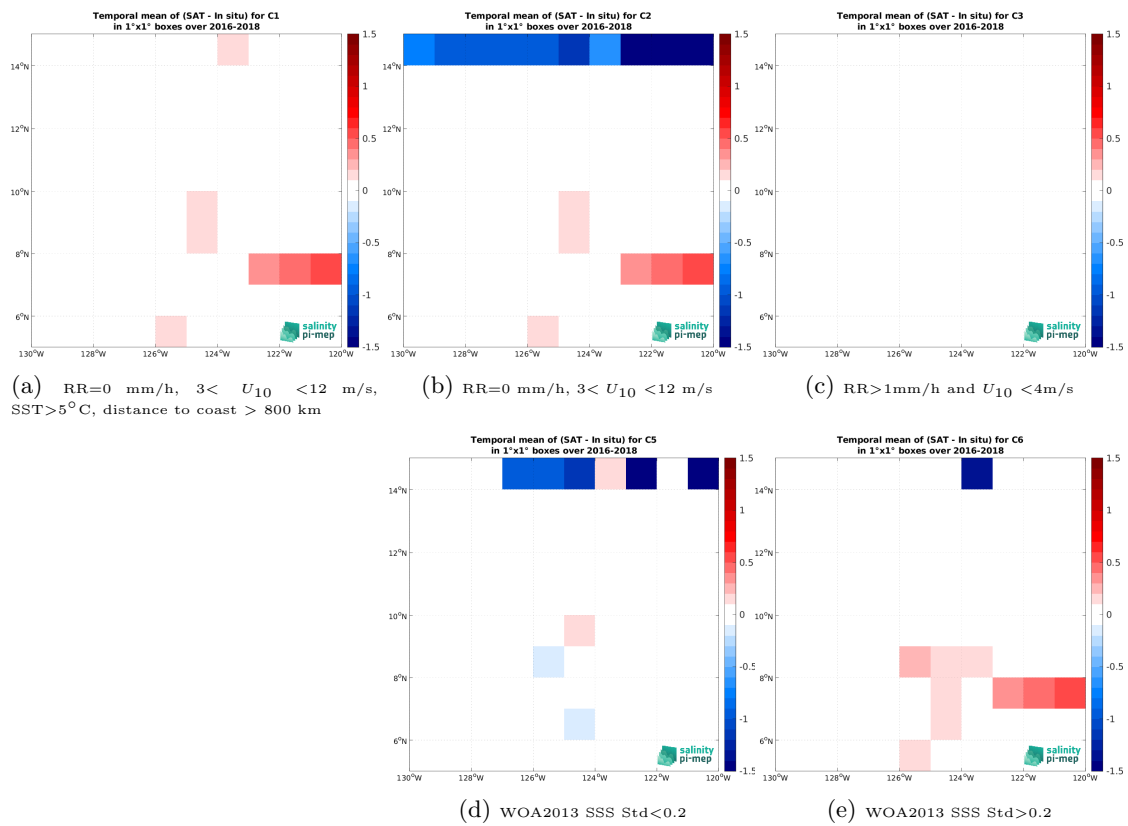
Figure 14: Temporal mean gridded over spatial boxes of size 1^\circ \times 1^\circ of \Delta SSS (SMAP SSS L3 v5.0 - 8-Day running (JPL) - TSG (SAMOS)) for 5 different subdatasets corresponding to:RR=0 mm/h, 3 < U_{10} < 12 m/s, SST > 5^\circ\text{C} , distance to coast > 800 km (a), RR=0 mm/h, 3 < U_{10} < 12 m/s (b), RR > 1 mm/h and U_{10} < 4 m/s (c), WOA2013 SSS Std < 0.2 (d), WOA2013 SSS Std > 0.2 (e).
