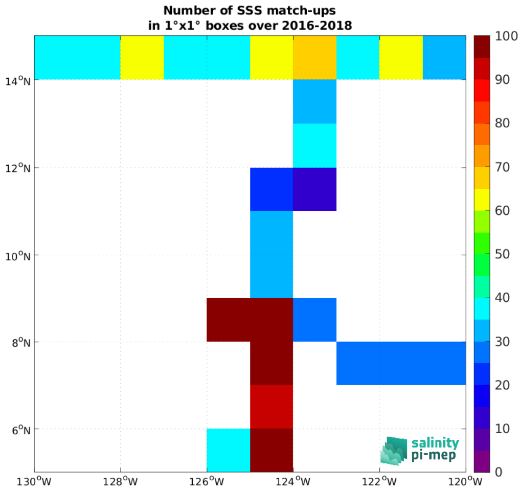
Figure 5: Number of SSS match-ups between TSG (SAMOS) SSS and the SMAP SSS L3 v5.0 - 8-Day running (JPL) SSS product for the SPURS 2 Pi-MEP region over 1^\circ \times 1^\circ boxes and for the full satellite product period.
