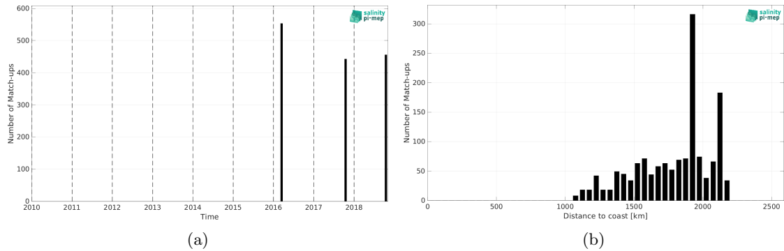
Figure 2: Number of match-ups between TSG (SAMOS) and SMAP SSS L3 v5.0 - 8-Day running (JPL) SSS as a function of time (a) and as function of the distance to coast (b) over the SPURS 2 Pi-MEP region and for the full satellite product period.
