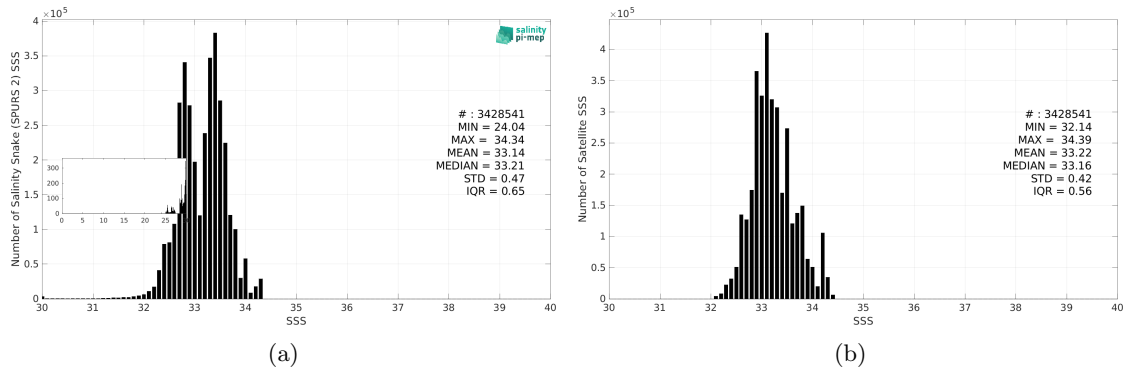
Figure 3: Histograms of SSS from Salinity Snake (SPURS 2) (a) and SMAP SSS L3 v5.0 - 8-Day running (JPL) (b) considering all match-up pairs per bins of 0.1 over the SPURS 2 Pi-MEP region and for the full satellite product period.
