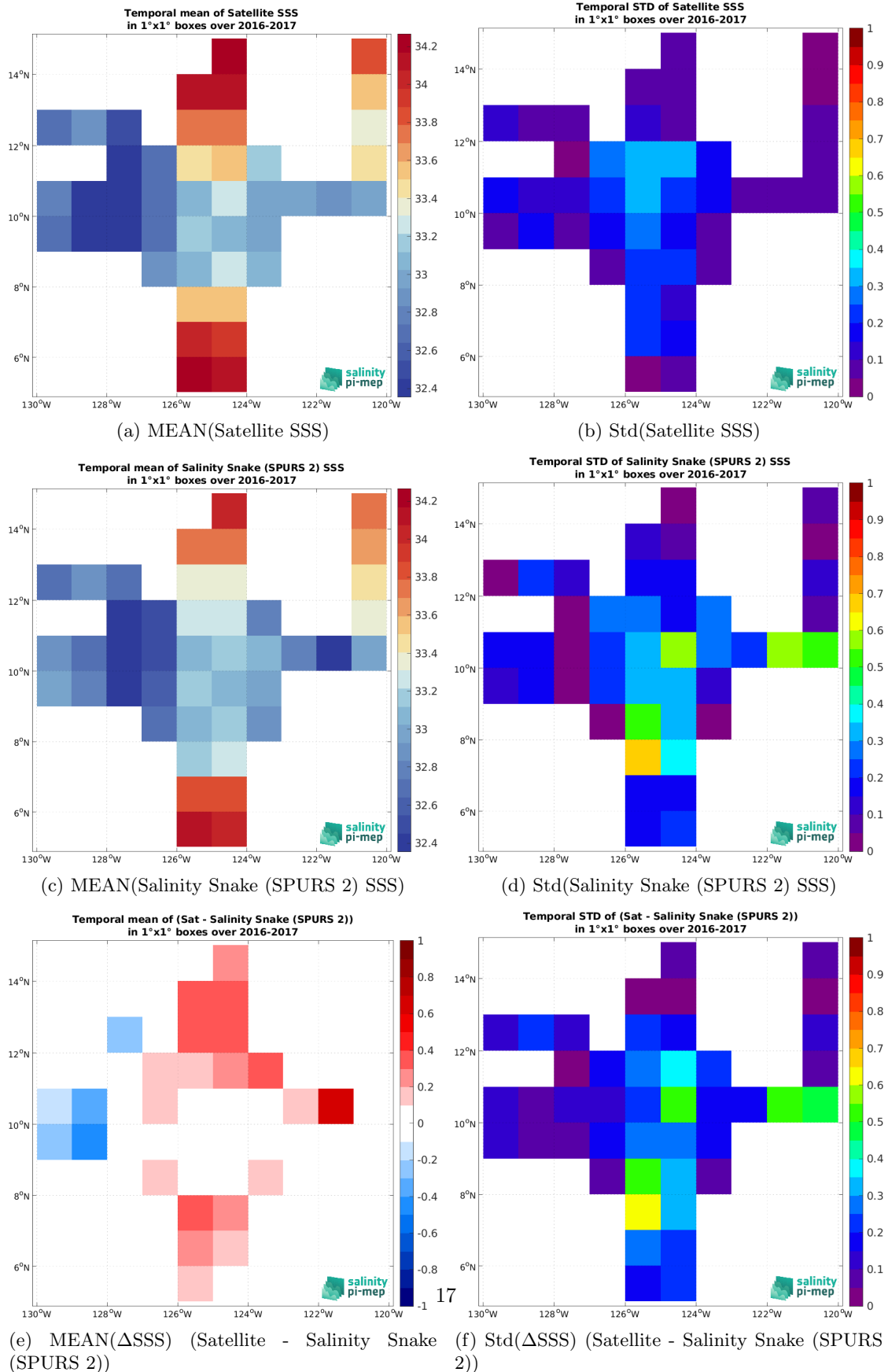
Figure 7: Temporal mean (left) and Std (right) of SSS from SMAP SSS L3 v5.0 - 8-Day running (JPL) (top), Salinity Snake (SPURS 2) (middle), and of \Delta SSS (Satellite - Salinity Snake (SPURS 2)). Only match-up pairs are used to generate these maps.
