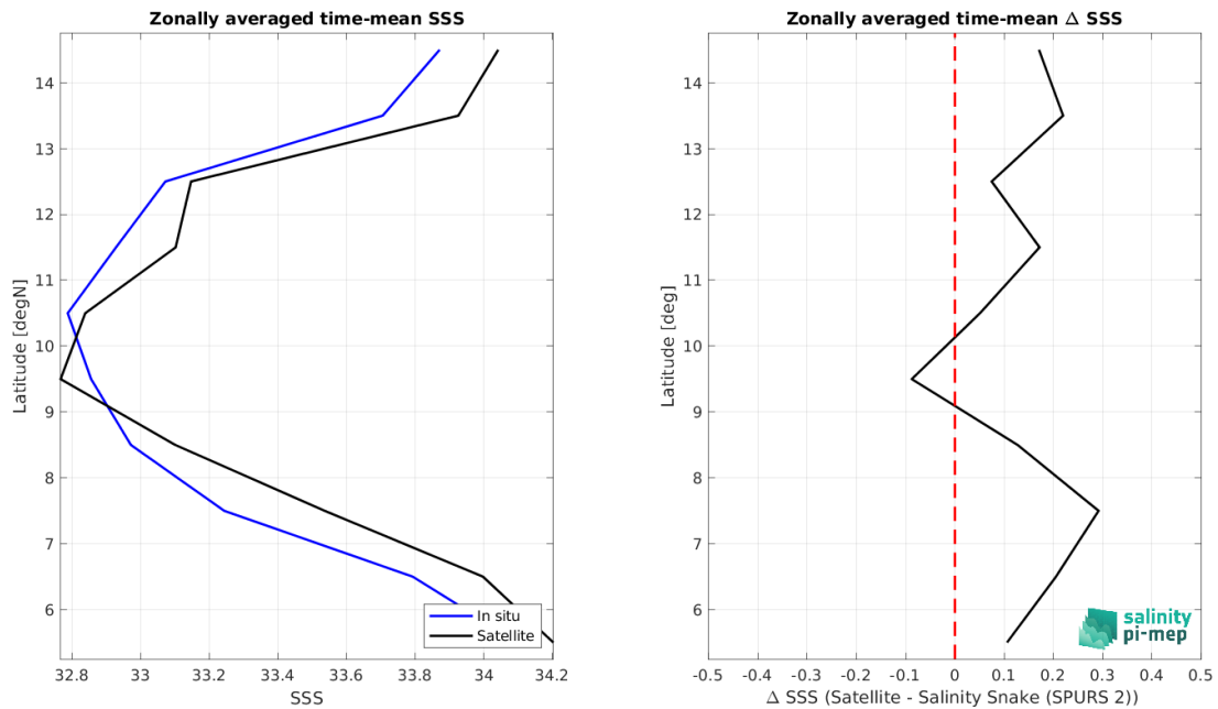
Figure 9: Left panel: Zonal mean SSS from SMAP SSS L3 v5.0 - 8-Day running (JPL) satellite product (black) and from Salinity Snake (SPURS 2) (blue). Right panel: Zonal mean of \Delta SSS (Satellite - Salinity Snake (SPURS 2)) for all the collected Pi-MEP match-up pairs estimated over the full satellite product period.
