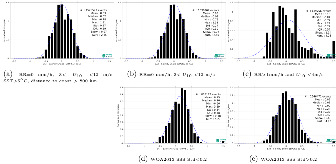
Figure 15: Normalized histogram of \Delta SSS (SMAP SSS L3 v5.0 - 8-Day running (JPL) - Salinity Snake (SPURS 2)) for 5 different subdatasets corresponding to: RR=0 mm/h, 3 < U_{10} < 12 m/s, SST>5°C, distance to coast > 800 km (a), RR=0 mm/h, 3 < U_{10} < 12 m/s (b), RR>1mm/h and U_{10} < 4 m/s (c), WOA2013 SSS Std<0.2 (d), WOA2013 SSS Std>0.2 (e).
