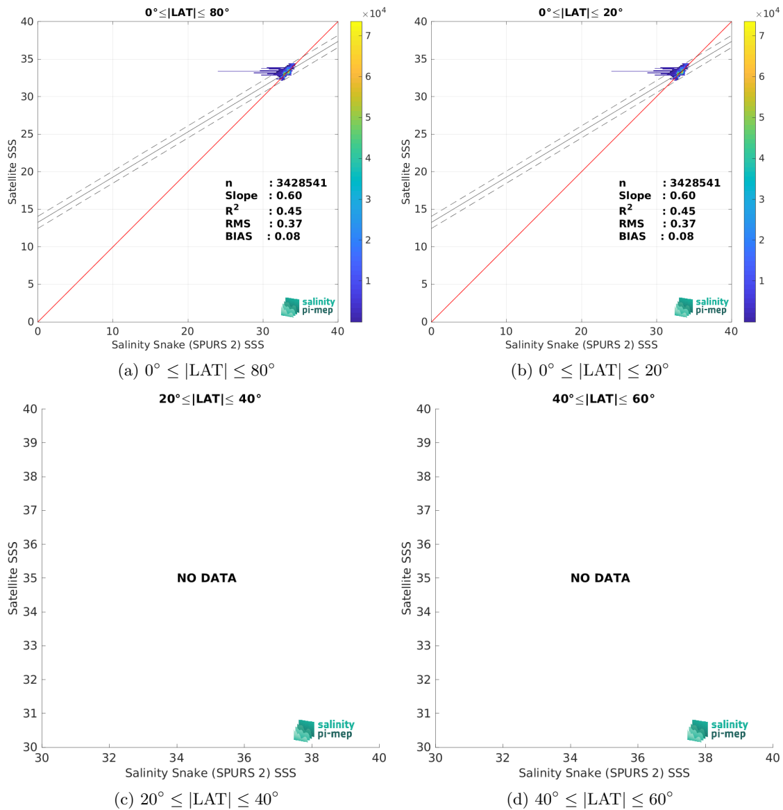
Figure 10: Contour maps of the concentration of SMAP SSS L3 v5.0 - 8-Day running (JPL) SSS (y-axis) versus Salinity Snake (SPURS 2) SSS (x-axis) at match-up pairs for different latitude bands. For each plot, the red line shows x=y . The black thin and dashed lines indicate a linear fit through the data cloud and the \pm 95\% confidence levels, respectively. The number match-up pairs n , the slope and R^2 coefficient of the linear fit, the root mean square (RMS) and the mean bias between satellite and in situ data are indicated for each latitude band in each plots.
