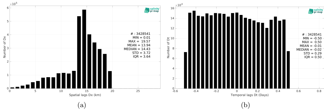
Figure 6: Histograms of the spatial (a) and temporal (b) lags between the location/time of the Salinity Snake (SPURS 2) measurement and the date of the corresponding SMAP SSS L3 v5.0 - 8-Day running (JPL) SSS pixel.
