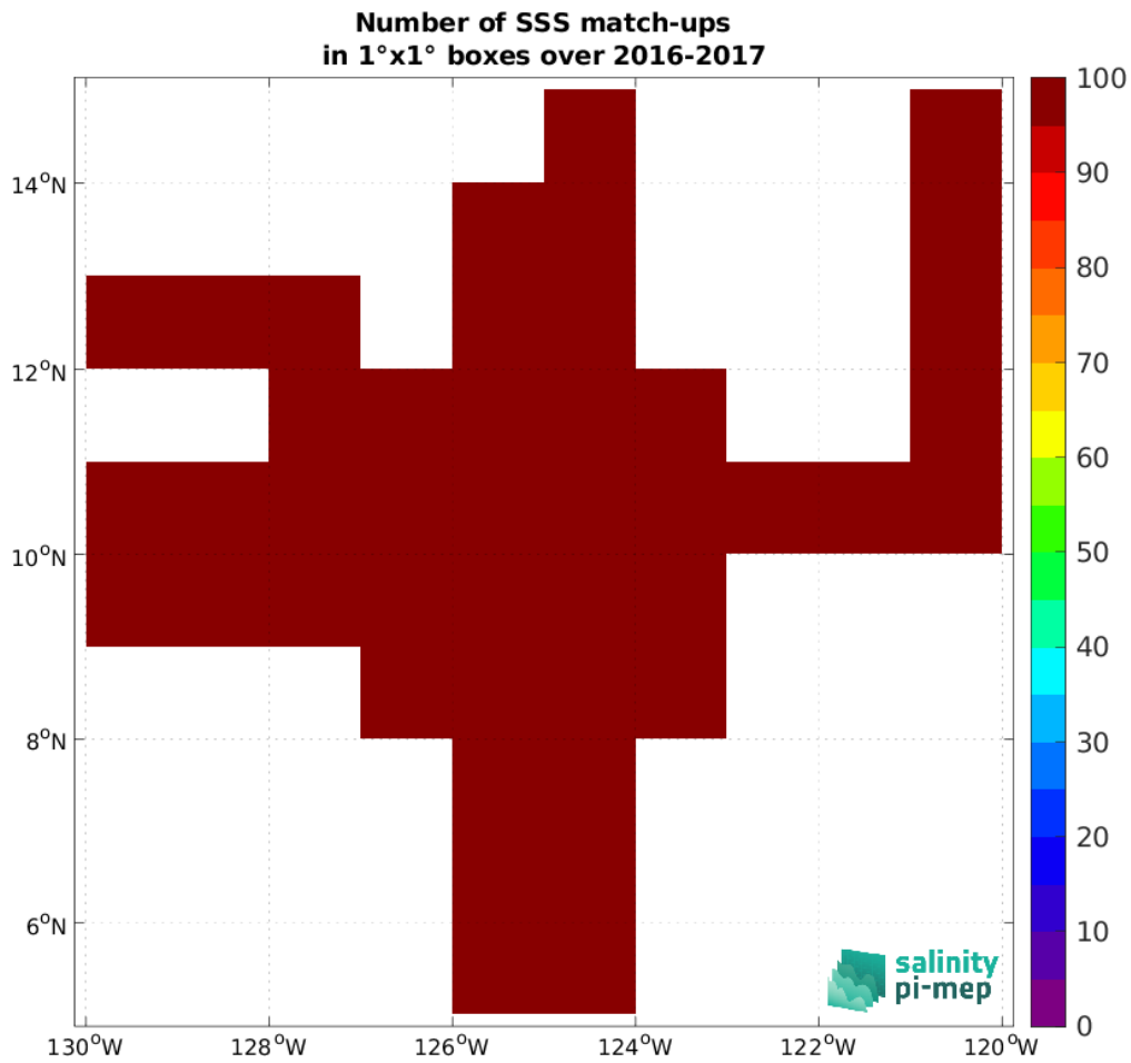
Figure 5: Number of SSS match-ups between Salinity Snake (SPURS 2) SSS and the SMAP SSS L3 v5.0 - 8-Day running (JPL) SSS product for the SPURS 2 Pi-MEP region over 1°x1° boxes and for the full satellite product period.
