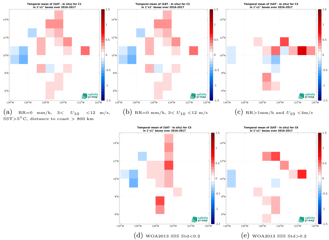
Figure 14: Temporal mean gridded over spatial boxes of size 1^\circ \times 1^\circ of \Delta\text{SSS} (SMAP SSS L3 v5.0 - 8-Day running (JPL) - Salinity Snake (SPURS 2)) for 5 different subdatasets corresponding to:RR=0 mm/h, 3 < U_{10} < 12 m/s, SST>5°C, distance to coast > 800 km (a), RR=0 mm/h, 3 < U_{10} < 12 m/s (b), RR>1mm/h and U_{10} < 4 m/s (c), WOA2013 SSS Std<0.2 (d), WOA2013 SSS Std>0.2 (e).
