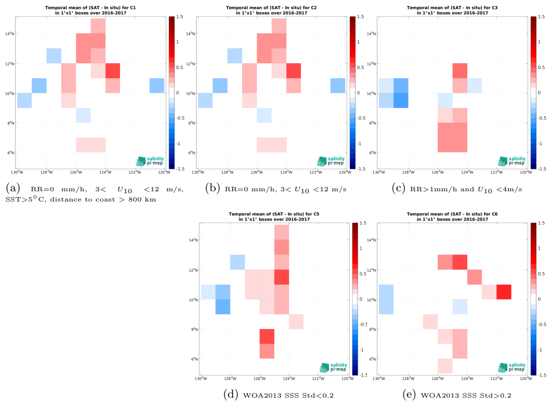
Figure 12: Temporal mean gridded over spatial boxes of size 1^\circ \times 1^\circ of \Delta\text{SSS} (SMAP SSS L3 v5.0 - 8-Day running (JPL) - Salinity Snake (SPURS 2)) for 5 different subdatasets corresponding to:RR=0 mm/h, 3 < U_{10} < 12 m/s, SST>5°C, distance to coast > 800 km (a), RR=0 mm/h, 3 < U_{10} < 12 m/s (b), RR>1mm/h and U_{10} < 4 m/s (c), WOA2013 SSS Std<0.2 (d), WOA2013 SSS Std>0.2 (e).
