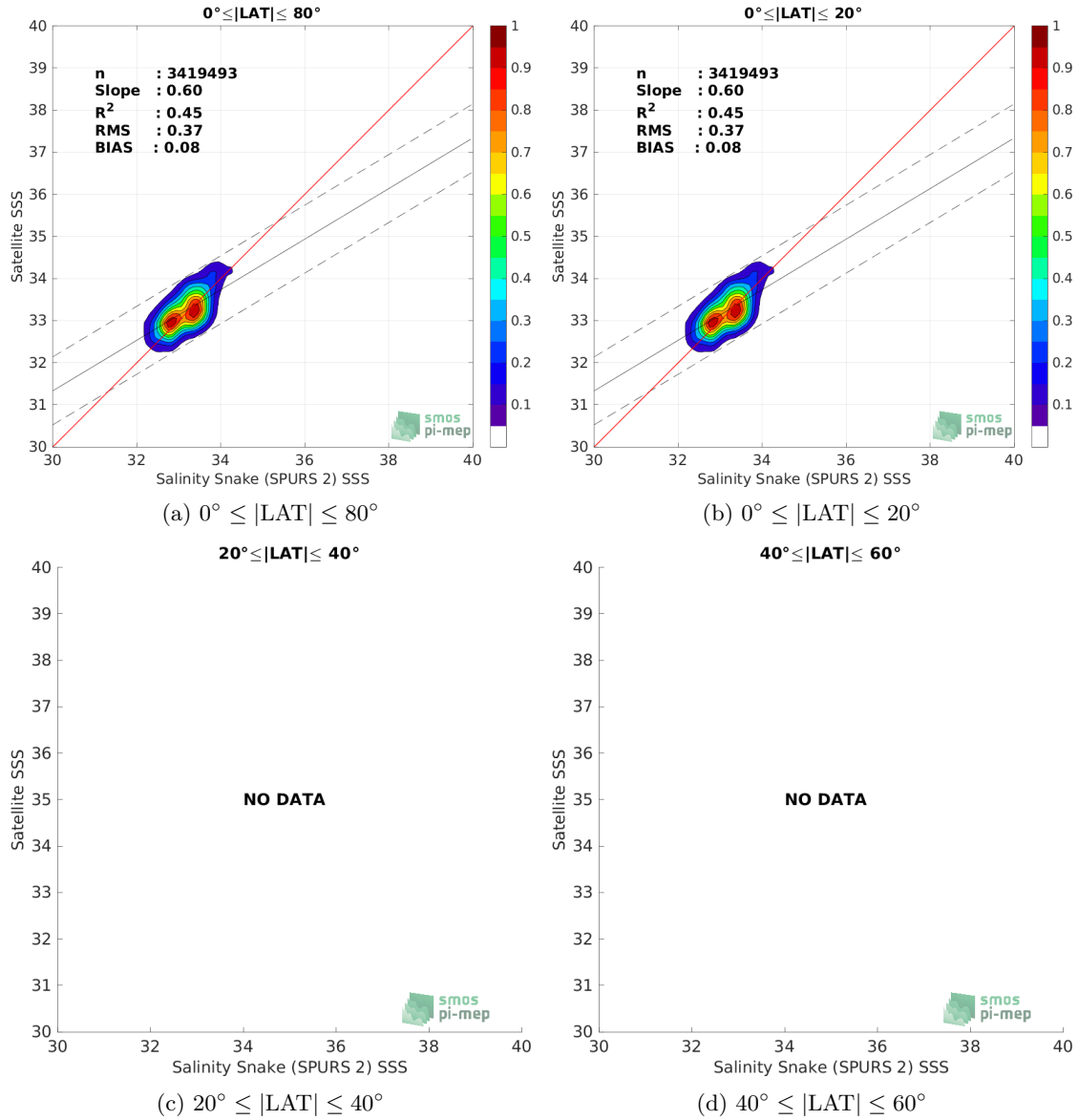
Figure 9: Contour maps of the concentration of SMAP SSS L3 v5.0 - 8-Day running (JPL) SSS (y-axis) versus Salinity Snake (SPURS 2) SSS (x-axis) at match-up pairs for different latitude bands. For each plot, the red line shows x=y . The black thin and dashed lines indicate a linear fit through the data cloud and the \pm 95\% confidence levels, respectively. The number match-up pairs n , the slope and R^2 coefficient of the linear fit, the root mean square (RMS) and the mean bias between satellite and in situ data are indicated for each latitude band in each plots.
