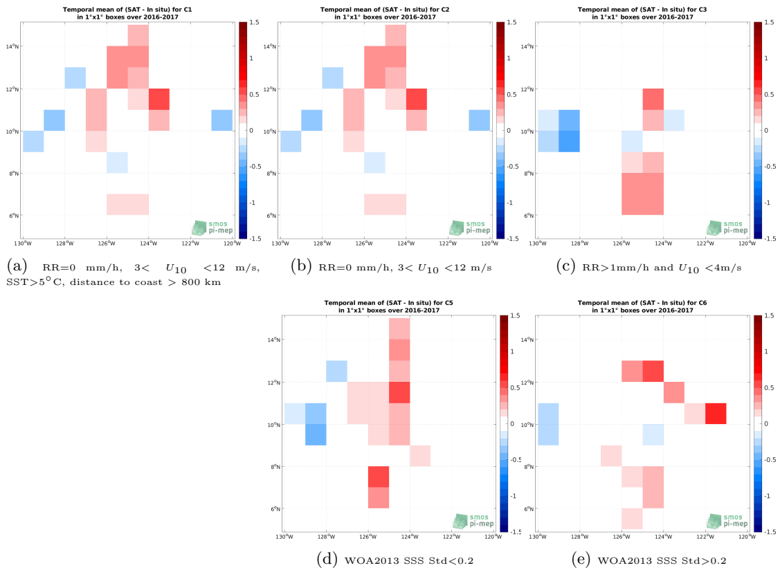
Figure 12: Temporal mean gridded over spatial boxes of size 1^\circ \times 1^\circ of \Delta SSS (SMAP SSS L3 v5.0 - 8-Day running (JPL) - Salinity Snake (SPURS 2)) for 5 different subdatasets corresponding to:RR=0 mm/h, 3 < U_{10} < 12 m/s, SST>5°C, distance to coast > 800 km (a), RR=0 mm/h, 3 < U_{10} < 12 m/s (b), RR>1mm/h and U_{10} < 4 m/s (c), WOA2013 SSS Std<0.2 (d), WOA2013 SSS Std>0.2 (e).
