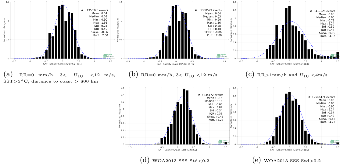
Figure 13: Normalized histogram of \Delta SSS (SMAP SSS L3 v5.0 - 8-Day running (JPL) - Salinity Snake (SPURS 2)) for 5 different subdatasets corresponding to: RR=0 mm/h, 3 < U_{10} < 12 m/s, SST>5°C, distance to coast > 800 km (a), RR=0 mm/h, 3 < U_{10} < 12 m/s (b), RR>1mm/h and U_{10} < 4 m/s (c), WOA2013 SSS Std<0.2 (d), WOA2013 SSS Std>0.2 (e).
