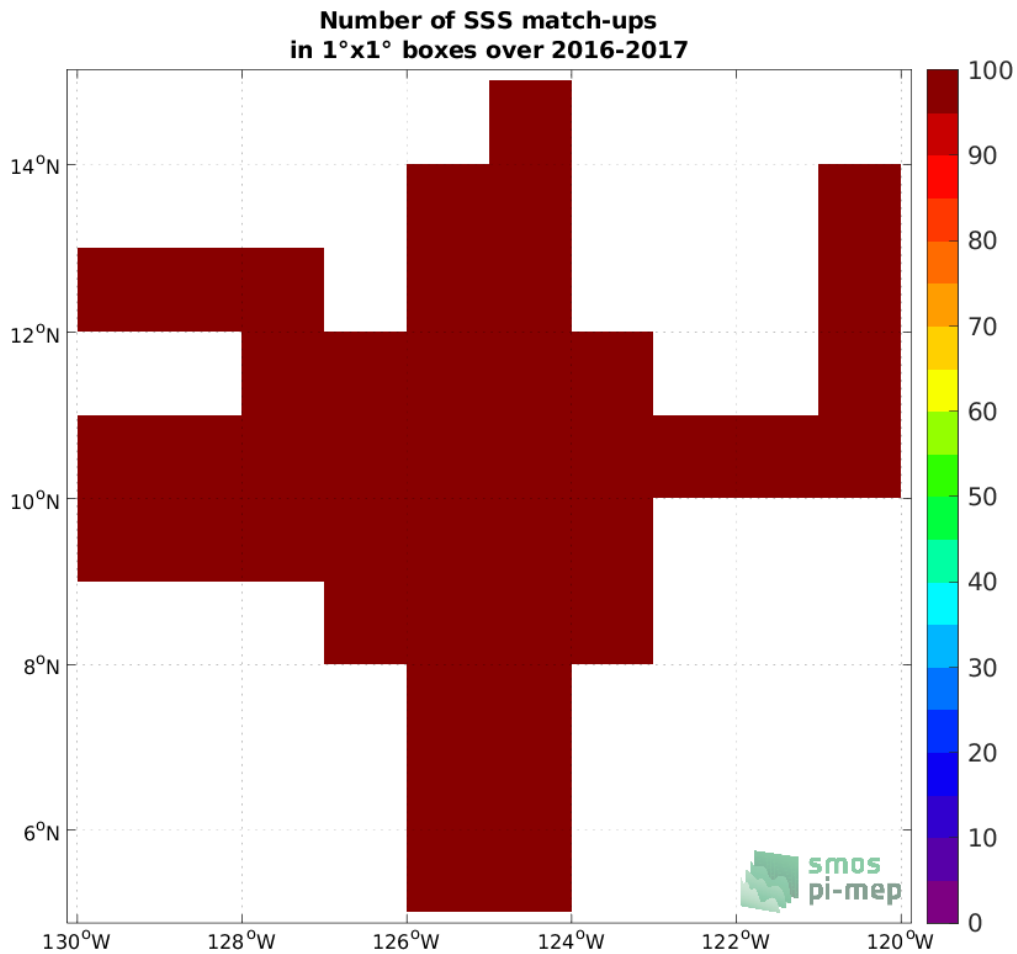
Figure 4: Number of SSS match-ups between Salinity Snake (SPURS 2) SSS and the SMAP SSS L3 v5.0 - 8-Day running (JPL) SSS product for the SPURS 2 Pi-MEP region over 1°x1° boxes and for the full satellite product period.
