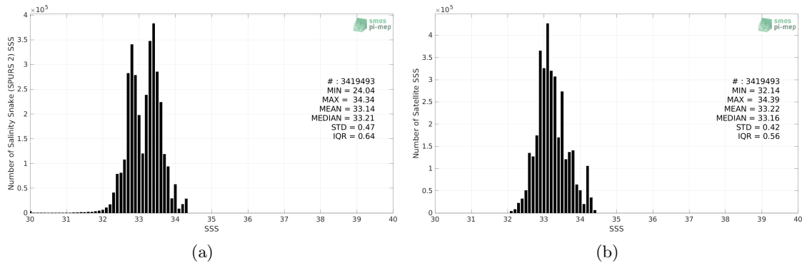
Figure 2: Histograms of SSS from Salinity Snake (SPURS 2) (a) and SMAP SSS L3 v5.0 - 8-Day running (JPL) (b) considering all match-up pairs per bins of 0.1 over the SPURS 2 Pi-MEP region and for the full satellite product period.
