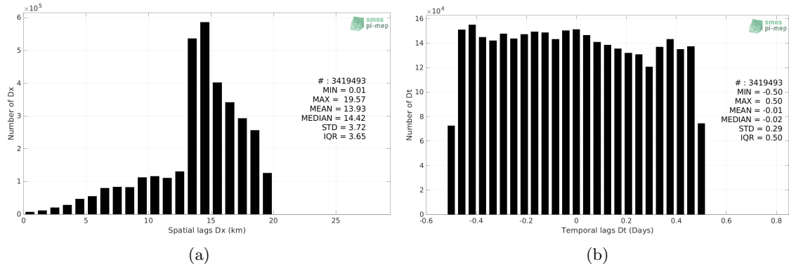
Figure 5: Histograms of the spatial (a) and temporal (b) lags between the location/time of the Salinity Snake (SPURS 2) measurement and the date of the corresponding SMAP SSS L3 v5.0 - 8-Day running (JPL) SSS pixel.
