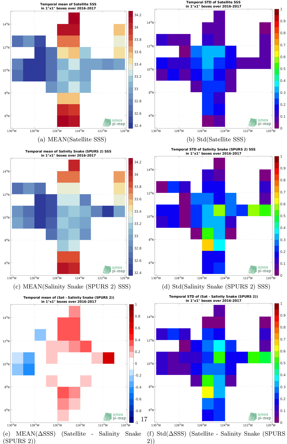
Figure 6: Temporal mean (left) and Std (right) of SSS from SMAP SSS L3 v5.0 - 8-Day running (JPL) (top), Salinity Snake (SPURS 2) (middle), and of \Delta SSS (Satellite - Salinity Snake (SPURS 2)). Only match-up pairs are used to generate these maps.
