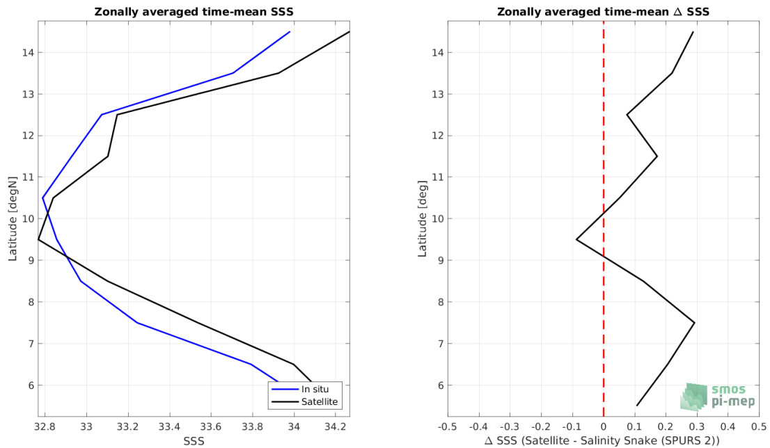
Figure 8: Left panel: Zonal mean SSS from SMAP SSS L3 v5.0 - 8-Day running (JPL) satellite product (black) and from Salinity Snake (SPURS 2) (blue). Right panel: Zonal mean of \Delta SSS (Satellite - Salinity Snake (SPURS 2)) for all the collected Pi-MEP match-up pairs estimated over the full satellite product period.
