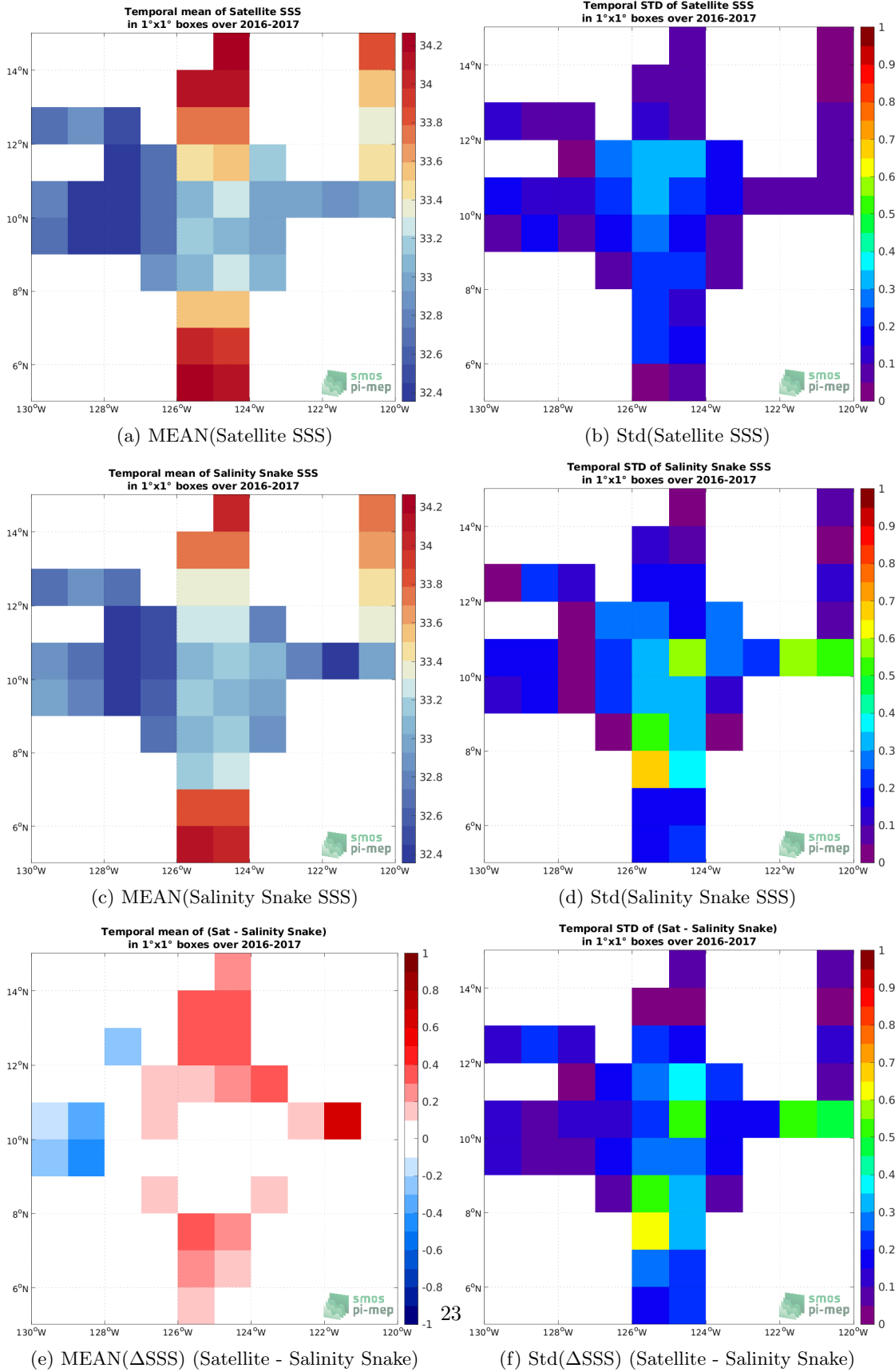
Figure 6: Temporal mean (left) and Std (right) of SSS from SMAP SSS L3 v5.0 - 8-Day running (JPL) (top), Salinity Snake (middle), and of \Delta SSS (Satellite - Salinity Snake). Only match-up pairs are used to generate these maps.
