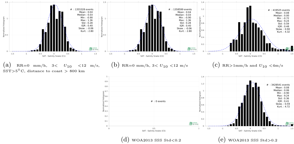
Figure 13: Normalized histogram of \Delta SSS (SMAP SSS L3 v5.0 - 8-Day running (JPL) - Salinity Snake) for 5 different subdatasets corresponding to: RR=0 mm/h, 3 < U_{10} < 12 m/s, SST > 5°C, distance to coast > 800 km (a), RR=0 mm/h, 3 < U_{10} < 12 m/s (b), RR > 1mm/h and U_{10} < 4 m/s (c), WOA2013 SSS Std < 0.2 (d), WOA2013 SSS Std > 0.2 (e).
