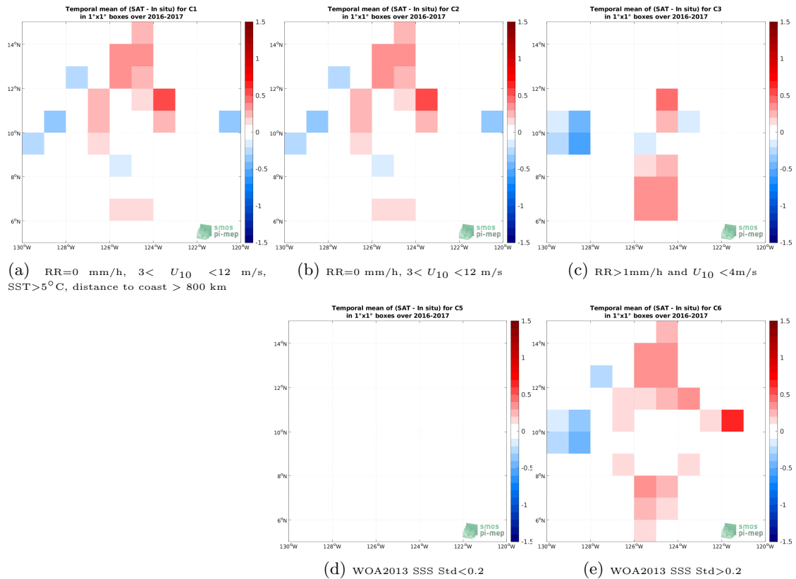
Figure 12: Temporal mean gridded over spatial boxes of size 1^\circ \times 1^\circ of \Delta SSS (SMAP SSS L3 v5.0 - 8-Day running (JPL) - Salinity Snake) for 5 different subdatasets corresponding to:RR=0 mm/h, 3 < U_{10} < 12 m/s, SST > 5^\circ\text{C} , distance to coast > 800 km (a), RR=0 mm/h, 3 < U_{10} < 12 m/s (b), RR > 1 mm/h and U_{10} < 4 m/s (c), WOA2013 SSS Std < 0.2 (d), WOA2013 SSS Std > 0.2 (e).
