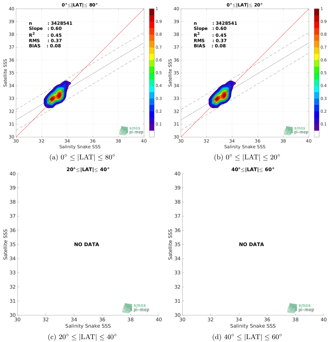
Figure 9: Contour maps of the concentration of SMAP SSS L3 v5.0 - 8-Day running (JPL) SSS (y-axis) versus Salinity Snake SSS (x-axis) at match-up pairs for different latitude bands. For each plot, the red line shows x=y . The black thin and dashed lines indicate a linear fit through the data cloud and the \pm 95\% confidence levels, respectively. The number match-up pairs n , the slope and R^2 coefficient of the linear fit, the root mean square (RMS) and the mean bias between satellite and in situ data are indicated for each latitude band in each plots.
