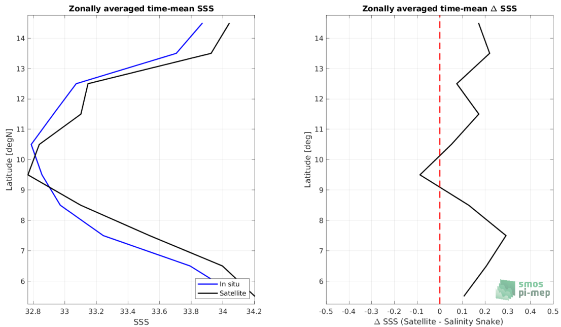
Figure 8: Left panel: Zonal mean SSS from SMAP SSS L3 v5.0 - 8-Day running (JPL) satellite product (black) and from Salinity Snake (blue). Right panel: Zonal mean of \Delta SSS (Satellite - Salinity Snake) for all the collected Pi-MEP match-up pairs estimated over the full satellite product period.
