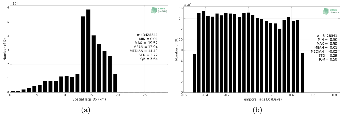
Figure 5: Histograms of the spatial (a) and temporal (b) lags between the location/time of the Salinity Snake measurement and the date of the corresponding SMAP SSS L3 v5.0 - 8-Day running (JPL) SSS pixel.
