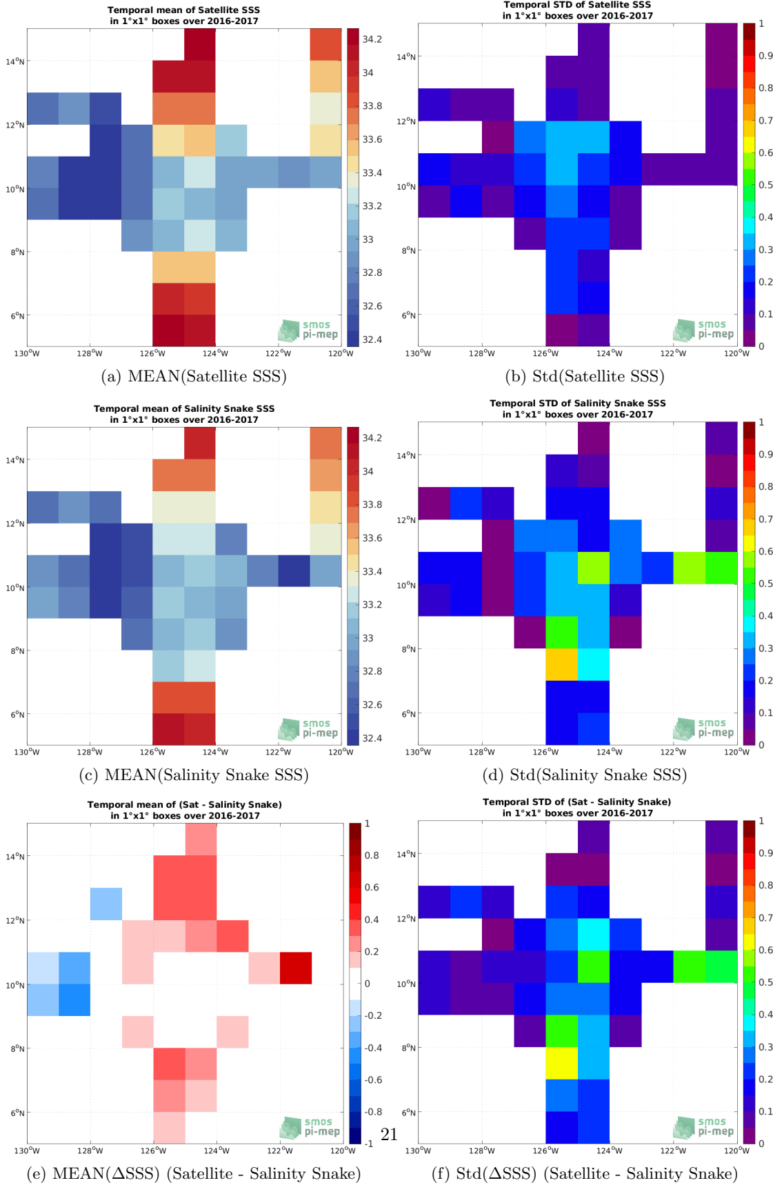
Figure 5: Temporal mean (left) and Std (right) of SSS from SMAP SSS L3 v5.0 - 8-Day running (JPL) (top), Salinity Snake (middle), and of \Delta SSS (Satellite - Salinity Snake). Only match-up pairs are used to generate these maps.
