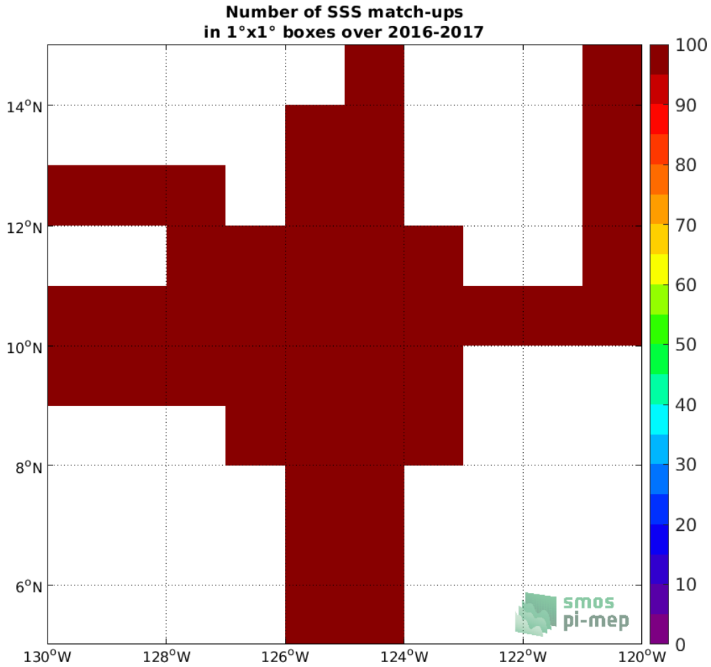
Figure 3: Number of SSS match-ups between Salinity Snake SSS and the SMAP SSS L3 v5.0 - 8-Day running (JPL) SSS product for the SPURS 2 Pi-MEP region over 1^\circ \times 1^\circ boxes and for the full satellite product period.
