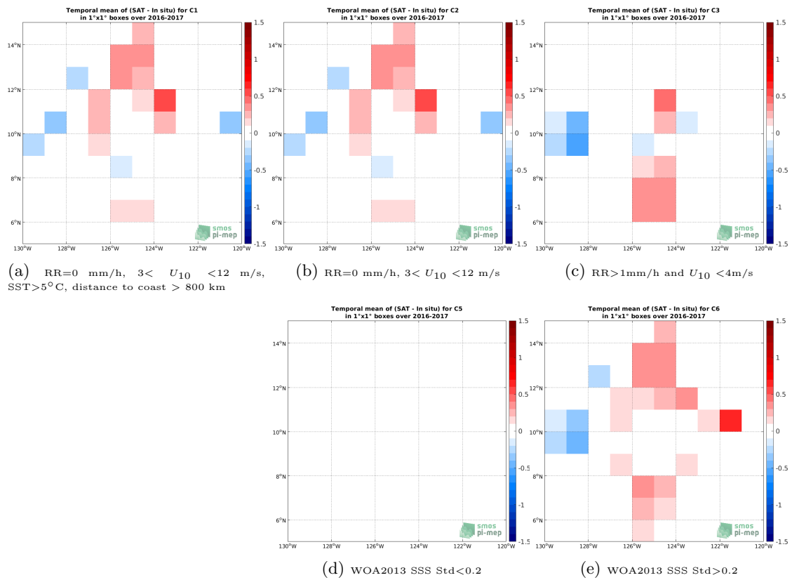
Figure 11: Temporal mean gridded over spatial boxes of size 1^\circ \times 1^\circ of \Delta SSS (SMAP SSS L3 v5.0 - 8-Day running (JPL) - Salinity Snake) for 5 different subdatasets corresponding to:RR=0 mm/h, 3 < U_{10} < 12 m/s, SST >5^\circ\text{C} , distance to coast > 800 km (a), RR=0 mm/h, 3 < U_{10} < 12 m/s (b), RR >1 mm/h and U_{10} < 4 m/s (c), WOA2013 SSS Std <0.2 (d), WOA2013 SSS Std >0.2 (e).
