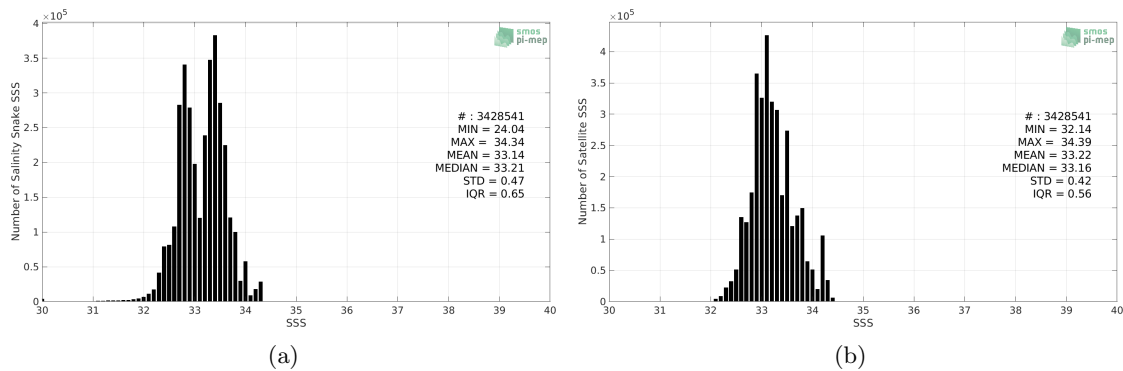
Figure 2: Histograms of SSS from Salinity Snake (a) and SMAP SSS L3 v5.0 - 8-Day running (JPL) (b) considering all match-up pairs per bins of 0.1 over the SPURS 2 Pi-MEP region and for the full satellite product period.
