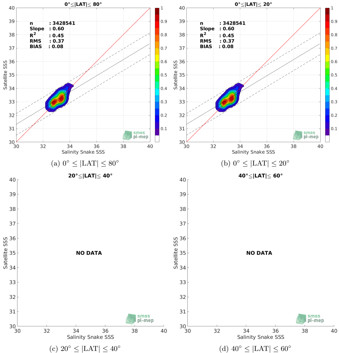
Figure 8: Contour maps of the concentration of SMAP SSS L3 v5.0 - 8-Day running (JPL) SSS (y-axis) versus Salinity Snake SSS (x-axis) at match-up pairs for different latitude bands. For each plot, the red line shows x=y . The black thin and dashed lines indicate a linear fit through the data cloud and the \pm 95\% confidence levels, respectively. The number match-up pairs n , the slope and R^2 coefficient of the linear fit, the root mean square (RMS) and the mean bias between satellite and in situ data are indicated for each latitude band in each plots.
