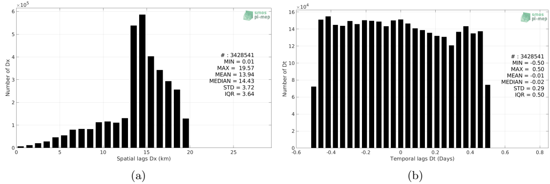
Figure 4: Histograms of the spatial (a) and temporal (b) lags between the location/time of the Salinity Snake measurement and the date of the corresponding SMAP SSS L3 v5.0 - 8-Day running (JPL) SSS pixel.
