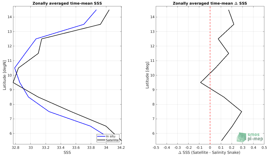
Figure 7: Left panel: Zonal mean SSS from SMAP SSS L3 v5.0 - 8-Day running (JPL) satellite product (black) and from Salinity Snake (blue). Right panel: Zonal mean of \Delta SSS (Satellite - Salinity Snake) for all the collected Pi-MEP match-up pairs estimated over the full satellite product period.
