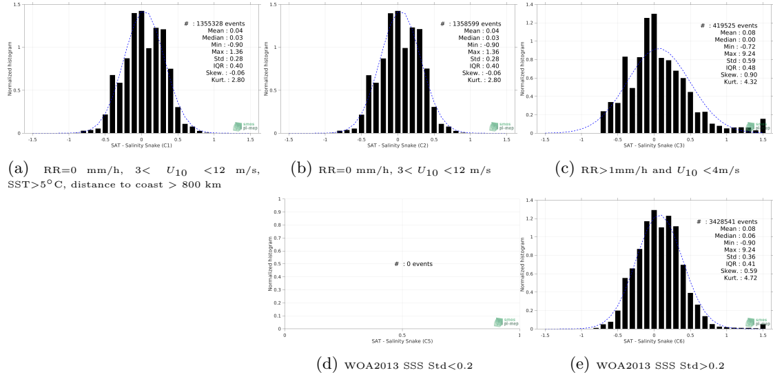
Figure 12: Normalized histogram of \Delta SSS (SMAP SSS L3 v5.0 - 8-Day running (JPL) - Salinity Snake) for 5 different subdatasets corresponding to: RR=0 mm/h, 3 < U_{10} < 12 m/s, SST > 5°C, distance to coast > 800 km (a), RR=0 mm/h, 3 < U_{10} < 12 m/s (b), RR > 1mm/h and U_{10} < 4 m/s (c), WOA2013 SSS Std < 0.2 (d), WOA2013 SSS Std > 0.2 (e).
