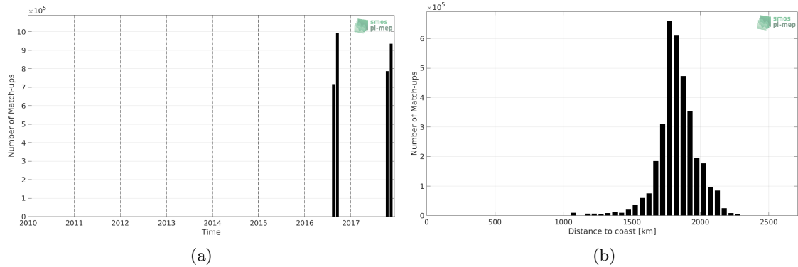
Figure 1: Number of match-ups between Salinity Snake and SMAP SSS L3 v5.0 - 8-Day running (JPL) SSS as a function of time (a) and as function of the distance to coast (b) over the SPURS 2 Pi-MEP region and for the full satellite product period.
