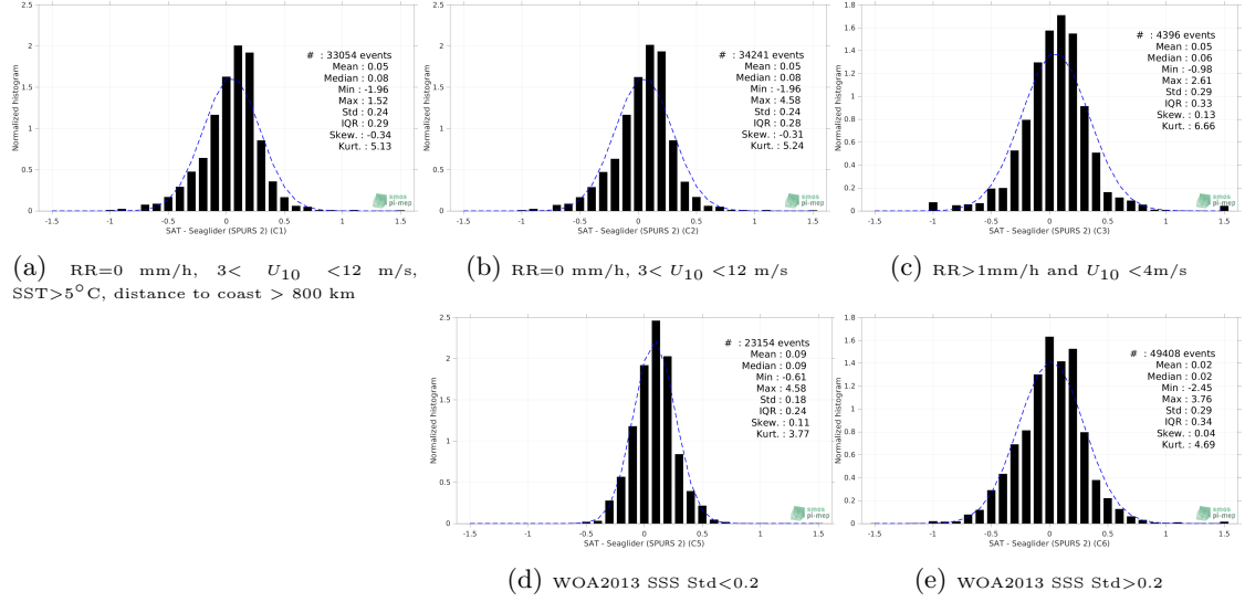
Figure 13: Normalized histogram of \Delta SSS (SMAP SSS L3 v5.0 - 8-Day running (JPL) - Seaglider (SPURS 2)) for 5 different subdatasets corresponding to: RR=0 mm/h, 3 < U_{10} < 12 m/s, SST>5°C, distance to coast > 800 km (a), RR=0 mm/h, 3 < U_{10} < 12 m/s (b), RR>1mm/h and U_{10} < 4 m/s (c), WOA2013 SSS Std<0.2 (d), WOA2013 SSS Std>0.2 (e).
