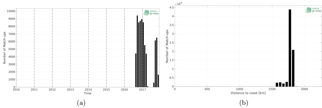
Figure 1: Number of match-ups between Seaglider (SPURS 2) and SMAP SSS L3 v5.0 - 8-Day running (JPL) SSS as a function of time (a) and as function of the distance to coast (b) over the SPURS 2 Pi-MEP region and for the full satellite product period.
