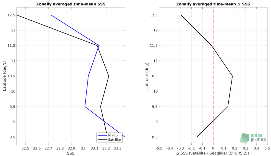
Figure 8: Left panel: Zonal mean SSS from SMAP SSS L3 v5.0 - 8-Day running (JPL) satellite product (black) and from Seaglider (SPURS 2) (blue). Right panel: Zonal mean of \Delta SSS (Satellite - Seaglider (SPURS 2)) for all the collected Pi-MEP match-up pairs estimated over the full satellite product period.
