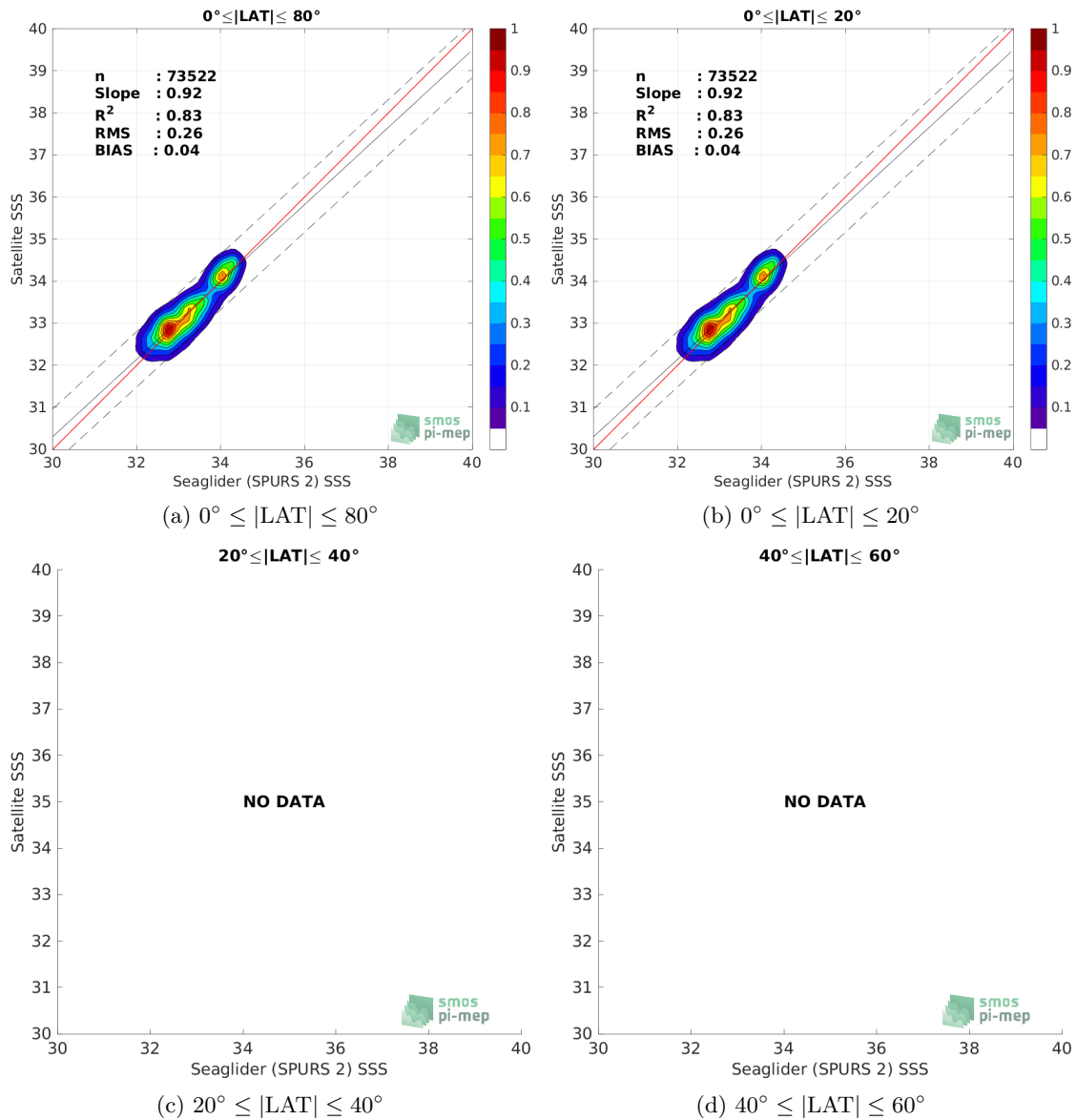
Figure 9: Contour maps of the concentration of SMAP SSS L3 v5.0 - 8-Day running (JPL) SSS (y-axis) versus Seaglider (SPURS 2) SSS (x-axis) at match-up pairs for different latitude bands. For each plot, the red line shows x=y . The black thin and dashed lines indicate a linear fit through the data cloud and the \pm 95\% confidence levels, respectively. The number match-up pairs n , the slope and R^2 coefficient of the linear fit, the root mean square (RMS) and the mean bias between satellite and in situ data are indicated for each latitude band in each plots.
