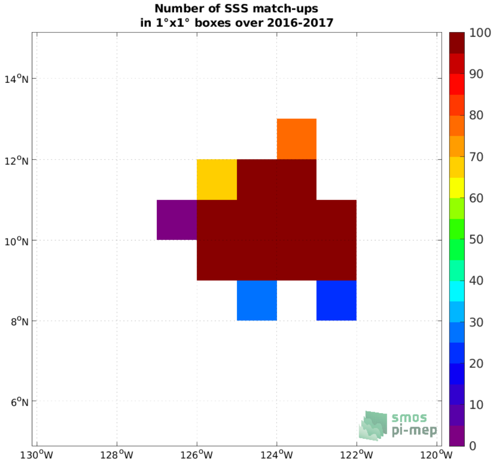
Figure 4: Number of SSS match-ups between Seaglider (SPURS 2) SSS and the SMAP SSS L3 v5.0 - 8-Day running (JPL) SSS product for the SPURS 2 Pi-MEP region over 1°x1° boxes and for the full satellite product period.
