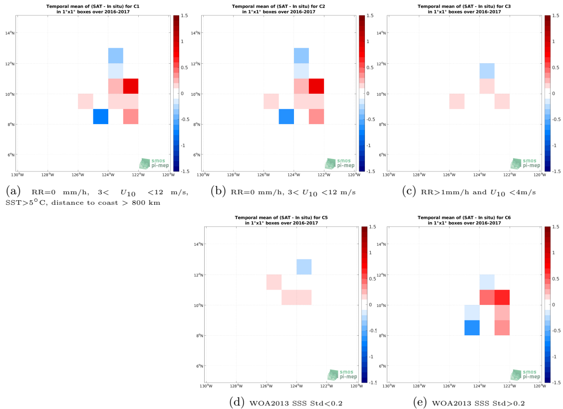
Figure 12: Temporal mean gridded over spatial boxes of size 1^\circ \times 1^\circ of \Delta SSS (SMAP SSS L3 v5.0 - 8-Day running (JPL) - Seaglider (SPURS 2)) for 5 different subdatasets corresponding to:RR=0 mm/h, 3 < U_{10} < 12 m/s, SST >5^\circ C, distance to coast > 800 km (a), RR=0 mm/h, 3 < U_{10} < 12 m/s (b), RR >1 mm/h and U_{10} < 4 m/s (c), WOA2013 SSS Std <0.2 (d), WOA2013 SSS Std >0.2 (e).
