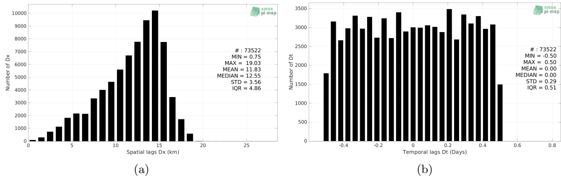
Figure 5: Histograms of the spatial (a) and temporal (b) lags between the location/time of the Seaglider (SPURS 2) measurement and the date of the corresponding SMAP SSS L3 v5.0 - 8-Day running (JPL) SSS pixel.
