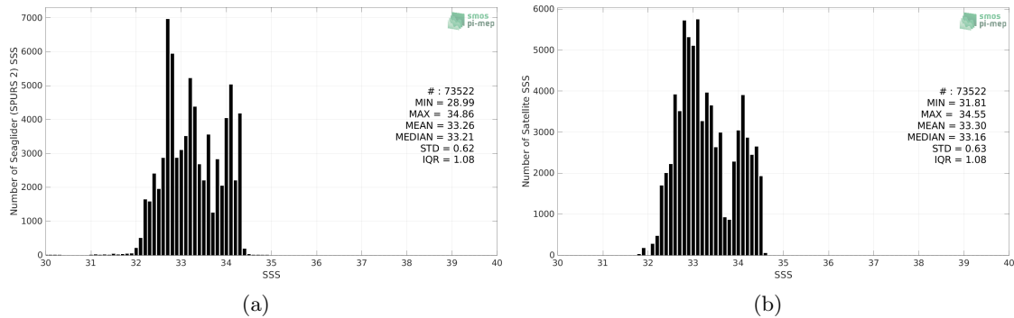
Figure 2: Histograms of SSS from Seaglider (SPURS 2) (a) and SMAP SSS L3 v5.0 - 8-Day running (JPL) (b) considering all match-up pairs per bins of 0.1 over the SPURS 2 Pi-MEP region and for the full satellite product period.
