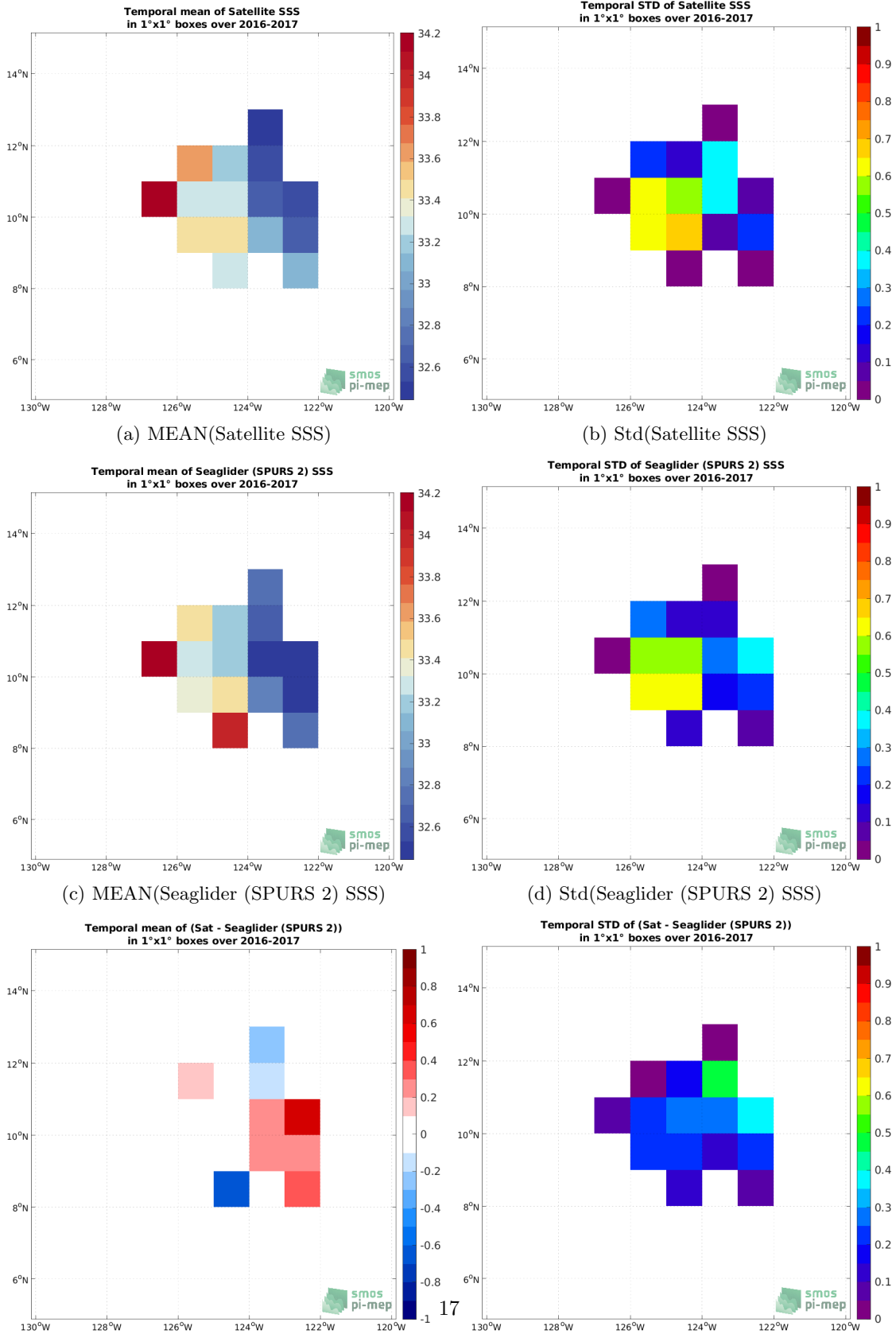
Figure 6: Temporal mean (left) and Std (right) of SSS from SMAP SSS L3 v5.0 - 8-Day running (JPL) (top), Seaglider (SPURS 2) (middle), and of \Delta SSS (Satellite - Seaglider (SPURS 2)). Only match-up pairs are used to generate these maps.
