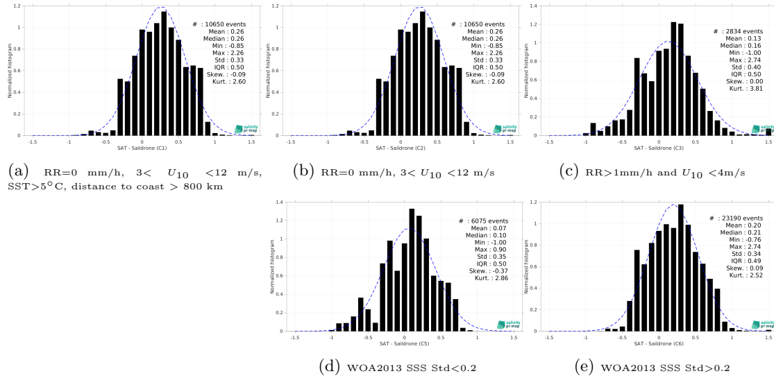
Figure 13: Normalized histogram of \Delta\text{SSS} (SMAP SSS L3 v5.0 - 8-Day running (JPL) - Saildrone) for 5 different subdatasets corresponding to: RR=0 mm/h, 3 < U_{10} < 12 m/s, SST>5°C, distance to coast > 800 km (a), RR=0 mm/h, 3 < U_{10} < 12 m/s (b), RR>1mm/h and U_{10} < 4 m/s (c), WOA2013 SSS Std<0.2 (d), WOA2013 SSS Std>0.2 (e).
