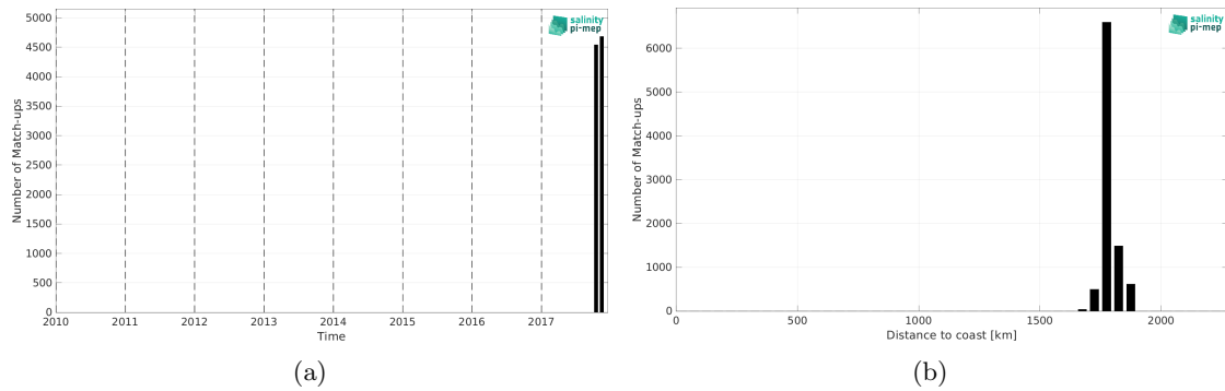
Figure 2: Number of match-ups between Saildrone (SPURS 2) and SMAP SSS L3 v5.0 - 8-Day running (JPL) SSS as a function of time (a) and as function of the distance to coast (b) over the SPURS 2 Pi-MEP region and for the full satellite product period.
