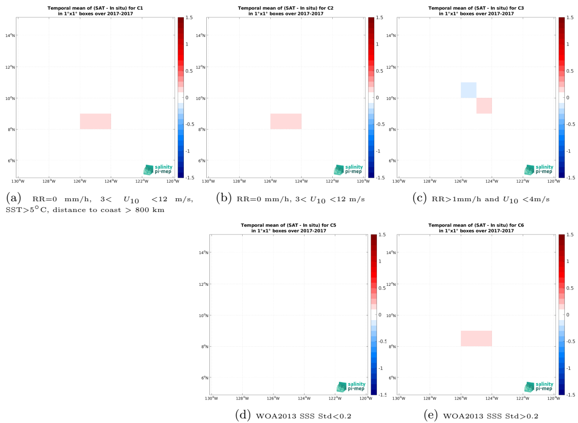
Figure 14: Temporal mean gridded over spatial boxes of size 1^\circ \times 1^\circ of \Delta SSS (SMAP SSS L3 v5.0 - 8-Day running (JPL) - Sairdron (SPURS 2)) for 5 different subdatasets corresponding to:RR=0 mm/h, 3 < U_{10} < 12 m/s, SST>5°C, distance to coast > 800 km (a), RR=0 mm/h, 3 < U_{10} < 12 m/s (b), RR>1mm/h and U_{10} < 4 m/s (c), WOA2013 SSS Std<0.2 (d), WOA2013 SSS Std>0.2 (e).
