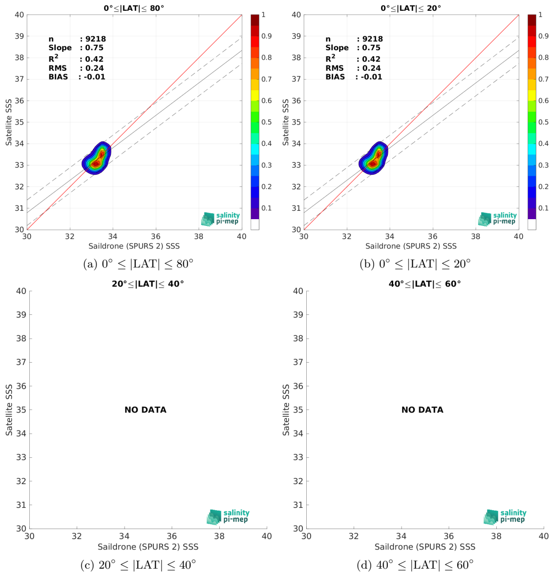
Figure 10: Contour maps of the concentration of SMAP SSS L3 v5.0 - 8-Day running (JPL) SSS (y-axis) versus Saildrone (SPURS 2) SSS (x-axis) at match-up pairs for different latitude bands. For each plot, the red line shows x=y . The black thin and dashed lines indicate a linear fit through the data cloud and the \pm 95\% confidence levels, respectively. The number match-up pairs n , the slope and R^2 coefficient of the linear fit, the root mean square (RMS) and the mean bias between satellite and in situ data are indicated for each latitude band in each plots.
