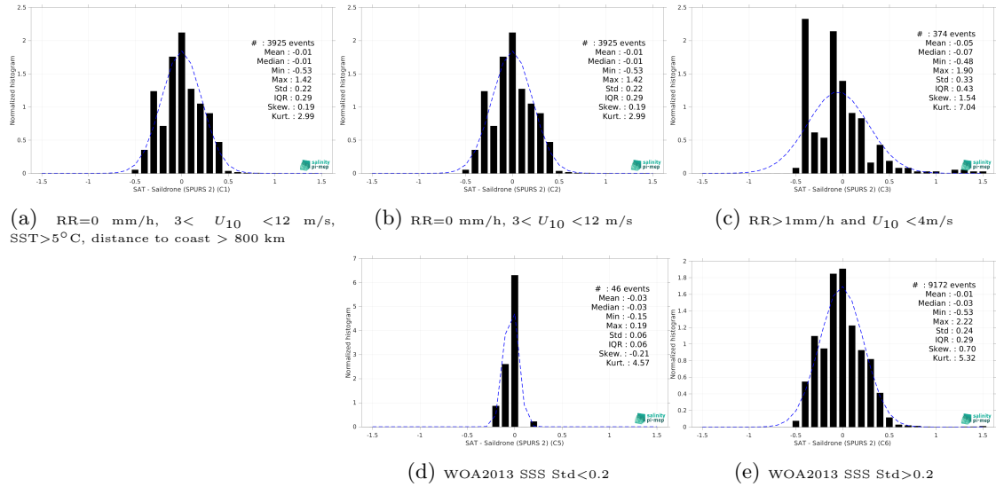
Figure 15: Normalized histogram of \Delta SSS (SMAP SSS L3 v5.0 - 8-Day running (JPL) - Saldrone (SPURS 2)) for 5 different subdatasets corresponding to: RR=0 mm/h, 3 < U_{10} < 12 m/s, SST > 5°C, distance to coast > 800 km (a), RR=0 mm/h, 3 < U_{10} < 12 m/s (b), RR > 1mm/h and U_{10} < 4 m/s (c), WOA2013 SSS Std < 0.2 (d), WOA2013 SSS Std > 0.2 (e).
