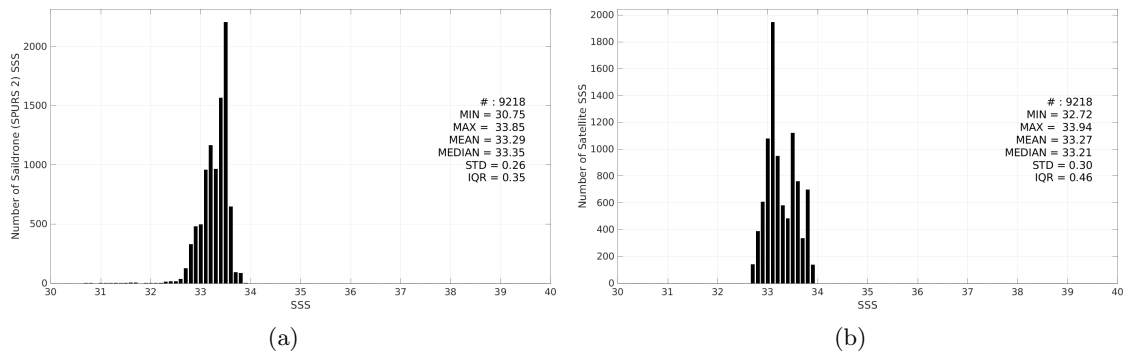
Figure 3: Histograms of SSS from Saildrone (SPURS 2) (a) and SMAP SSS L3 v5.0 - 8-Day running (JPL) (b) considering all match-up pairs per bins of 0.1 over the SPURS 2 Pi-MEP region and for the full satellite product period.
