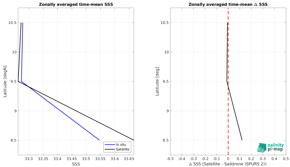
Figure 9: Left panel: Zonal mean SSS from SMAP SSS L3 v5.0 - 8-Day running (JPL) satellite product (black) and from Sairdron (SPURS 2) (blue). Right panel: Zonal mean of \Delta SSS (Satellite - Sairdron (SPURS 2)) for all the collected Pi-MEP match-up pairs estimated over the full satellite product period.
