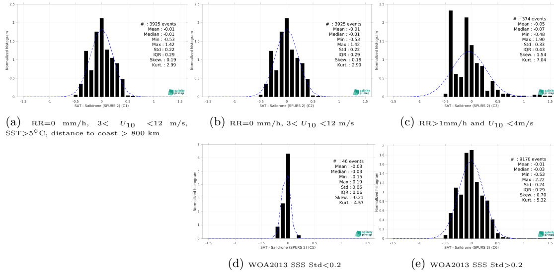
Figure 15: Normalized histogram of \Delta SSS (SMAP SSS L3 v5.0 - 8-Day running (JPL) - Saldrone (SPURS 2)) for 5 different subdatasets corresponding to: RR=0 mm/h, 3 < U_{10} < 12 m/s, SST>5°C, distance to coast > 800 km (a), RR=0 mm/h, 3 < U_{10} < 12 m/s (b), RR>1mm/h and U_{10} < 4 m/s (c), WOA2013 SSS Std<0.2 (d), WOA2013 SSS Std>0.2 (e).
