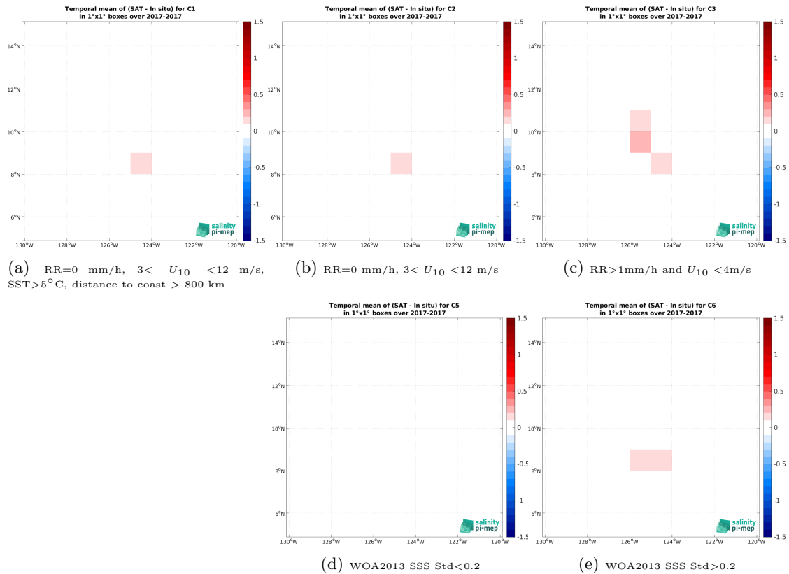
Figure 12: Temporal mean gridded over spatial boxes of size 1^\circ \times 1^\circ of \Delta SSS (SMAP SSS L3 v5.0 - 8-Day running (JPL) - Sailerone (SPURS 2)) for 5 different subdatasets corresponding to:RR=0 mm/h, 3 < U_{10} < 12 m/s, SST >5^\circ C, distance to coast > 800 km (a), RR=0 mm/h, 3 < U_{10} < 12 m/s (b), RR >1 mm/h and U_{10} < 4 m/s (c), WOA2013 SSS Std <0.2 (d), WOA2013 SSS Std >0.2 (e).
