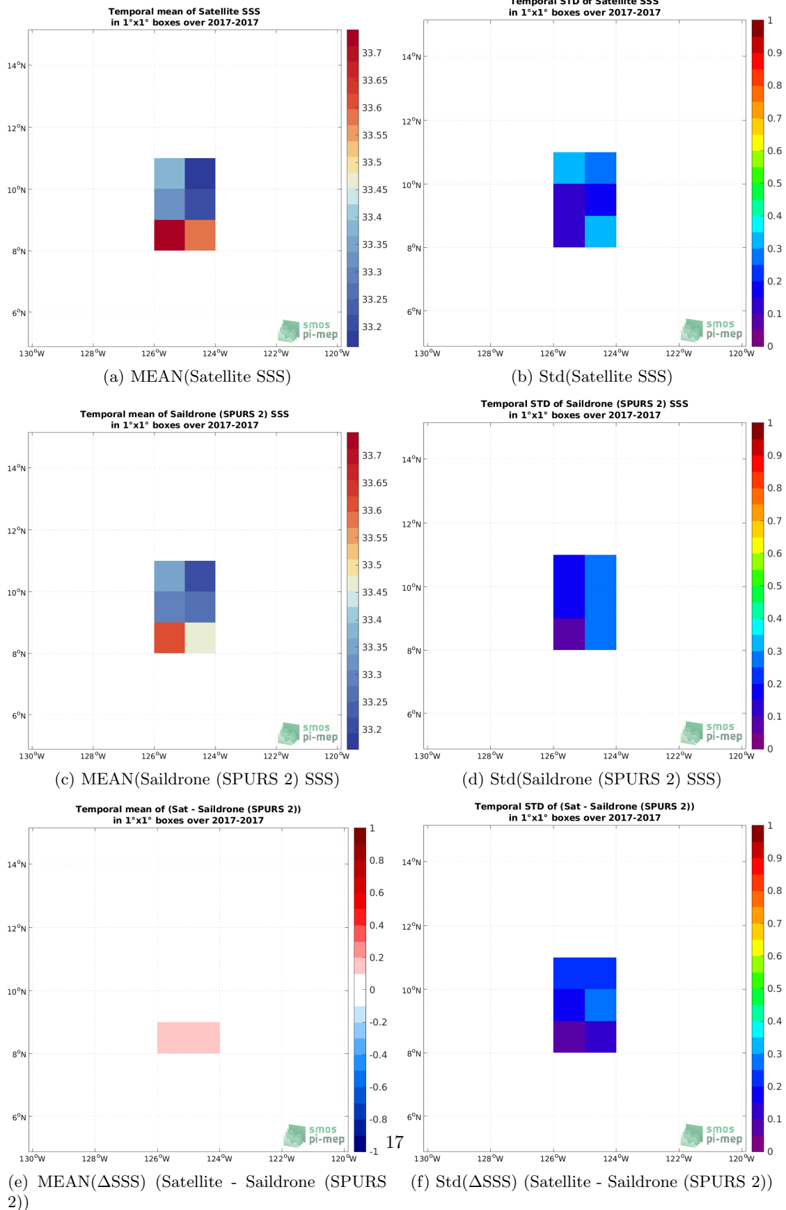
Figure 6: Temporal mean (left) and Std (right) of SSS from SMAP SSS L3 v5.0 - 8-Day running (JPL) (top), Saildrone (SPURS 2) (middle), and of \Delta SSS (Satellite - Saildrone (SPURS 2)). Only match-up pairs are used to generate these maps.
