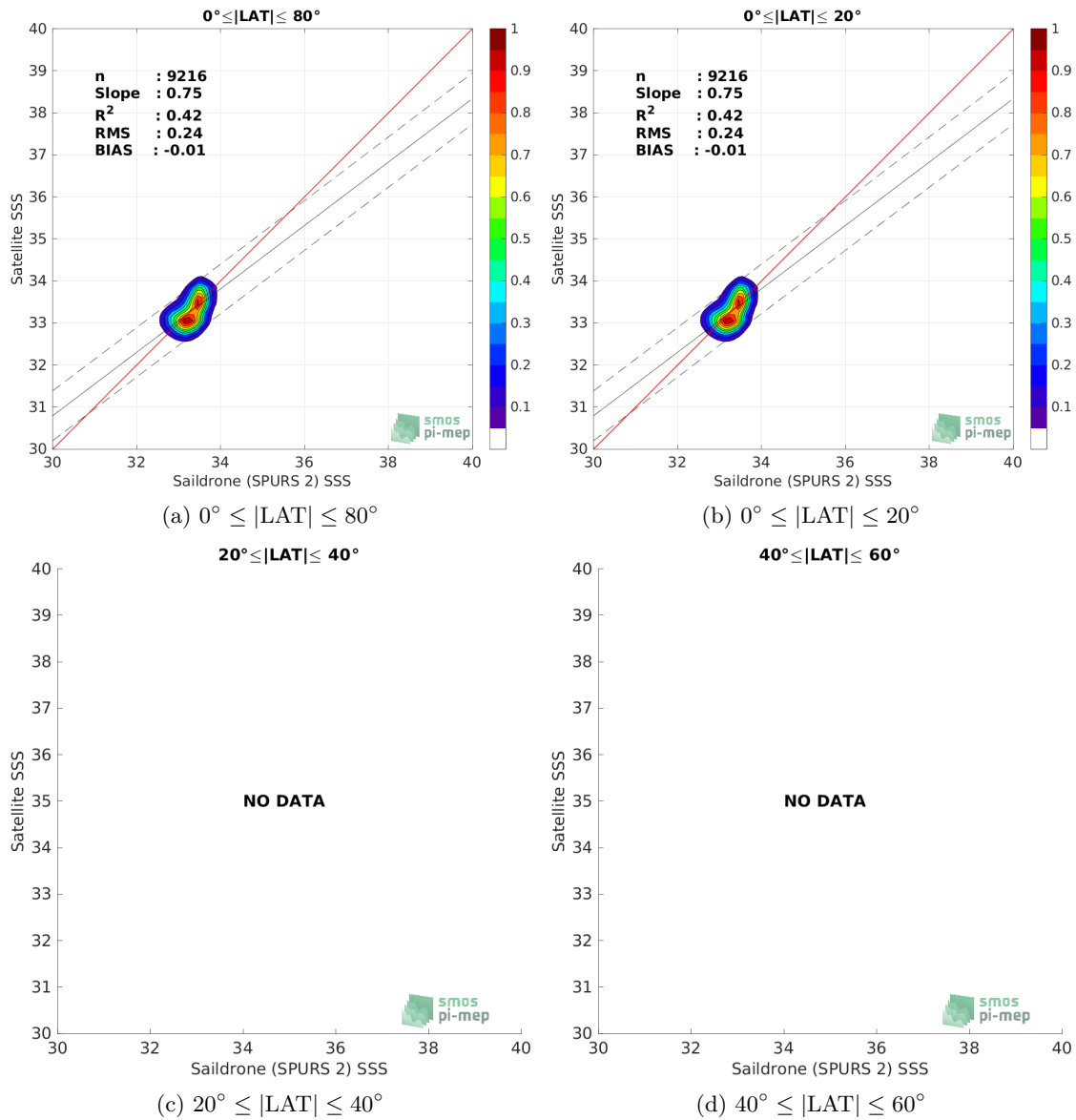
Figure 9: Contour maps of the concentration of SMAP SSS L3 v5.0 - 8-Day running (JPL) SSS (y-axis) versus Saildrone (SPURS 2) SSS (x-axis) at match-up pairs for different latitude bands. For each plot, the red line shows x=y . The black thin and dashed lines indicate a linear fit through the data cloud and the \pm 95\% confidence levels, respectively. The number match-up pairs n , the slope and R^2 coefficient of the linear fit, the root mean square (RMS) and the mean bias between satellite and in situ data are indicated for each latitude band in each plots.
