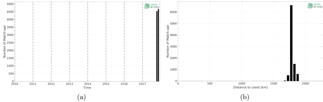
Figure 1: Number of match-ups between Saildrone (SPURS 2) and SMAP SSS L3 v5.0 - 8-Day running (JPL) SSS as a function of time (a) and as function of the distance to coast (b) over the SPURS 2 Pi-MEP region and for the full satellite product period.
