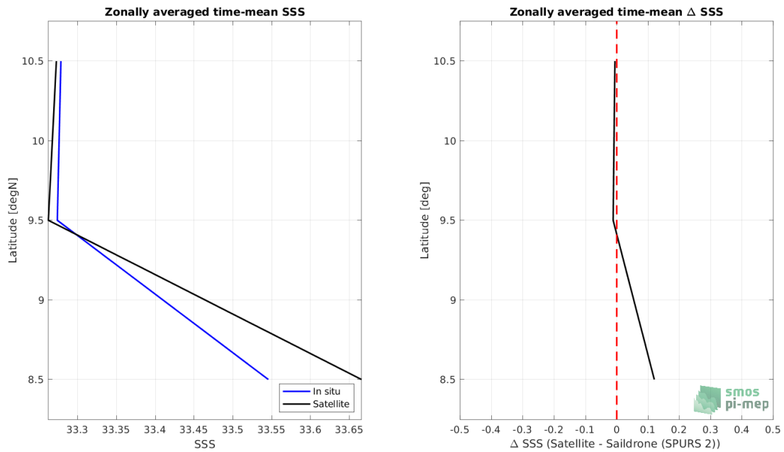
Figure 8: Left panel: Zonal mean SSS from SMAP SSS L3 v5.0 - 8-Day running (JPL) satellite product (black) and from Sairdron (SPURS 2) (blue). Right panel: Zonal mean of \Delta SSS (Satellite - Sairdron (SPURS 2)) for all the collected Pi-MEP match-up pairs estimated over the full satellite product period.
