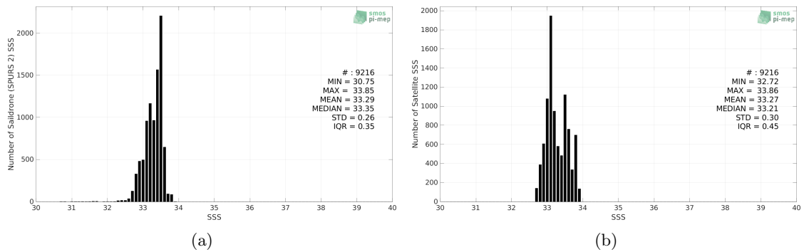
Figure 2: Histograms of SSS from Saildrone (SPURS 2) (a) and SMAP SSS L3 v5.0 - 8-Day running (JPL) (b) considering all match-up pairs per bins of 0.1 over the SPURS 2 Pi-MEP region and for the full satellite product period.
