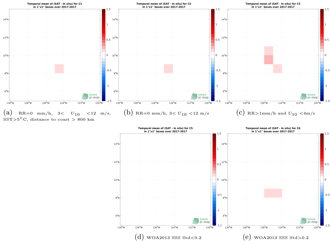
Figure 12: Temporal mean gridded over spatial boxes of size 1^\circ \times 1^\circ of \Delta SSS (SMAP SSS L3 v5.0 - 8-Day running (JPL) - Sairdron (SPURS 2)) for 5 different subdatasets corresponding to:RR=0 mm/h, 3 < U_{10} < 12 m/s, SST >5^\circ C, distance to coast > 800 km (a), RR=0 mm/h, 3 < U_{10} < 12 m/s (b), RR >1 mm/h and U_{10} < 4 m/s (c), WOA2013 SSS Std <0.2 (d), WOA2013 SSS Std >0.2 (e).
