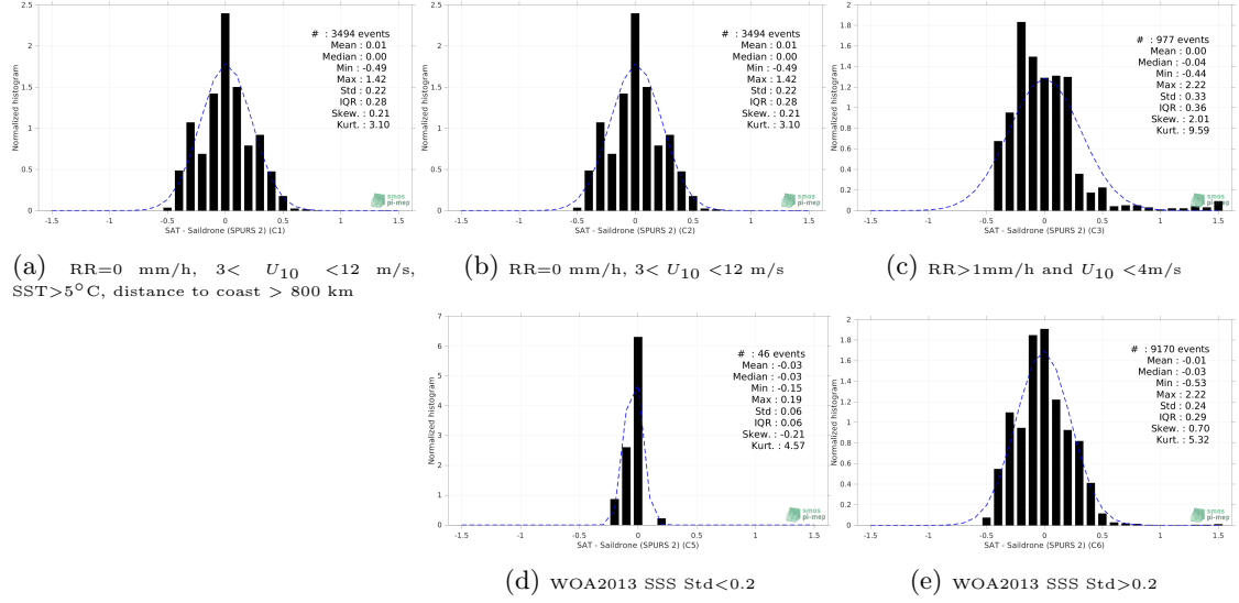
Figure 13: Normalized histogram of \Delta SSS (SMAP SSS L3 v5.0 - 8-Day running (JPL) - Saldrone (SPURS 2)) for 5 different subdatasets corresponding to: RR=0 mm/h, 3 < U_{10} < 12 m/s, SST>5°C, distance to coast > 800 km (a), RR=0 mm/h, 3 < U_{10} < 12 m/s (b), RR>1mm/h and U_{10} < 4 m/s (c), WOA2013 SSS Std<0.2 (d), WOA2013 SSS Std>0.2 (e).
