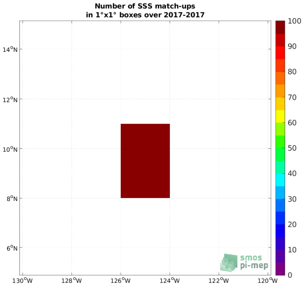
Figure 4: Number of SSS match-ups between Saifdrone (SPURS 2) SSS and the SMAP SSS L3 v5.0 - 8-Day running (JPL) SSS product for the SPURS 2 Pi-MEP region over 1°x1° boxes and for the full satellite product period.
