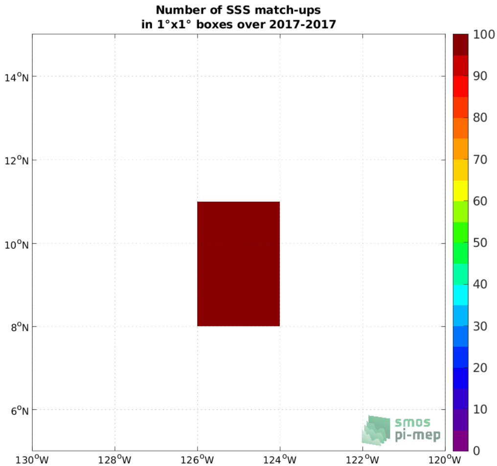
Figure 4: Number of SSS match-ups between Saildrone SSS and the SMAP SSS L3 v5.0 - 8-Day running (JPL) SSS product for the SPURS 2 Pi-MEP region over 1°x1° boxes and for the full satellite product period.
