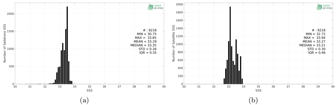
Figure 2: Histograms of SSS from Saildrone (a) and SMAP SSS L3 v5.0 - 8-Day running (JPL) (b) considering all match-up pairs per bins of 0.1 over the SPURS 2 Pi-MEP region and for the full satellite product period.
