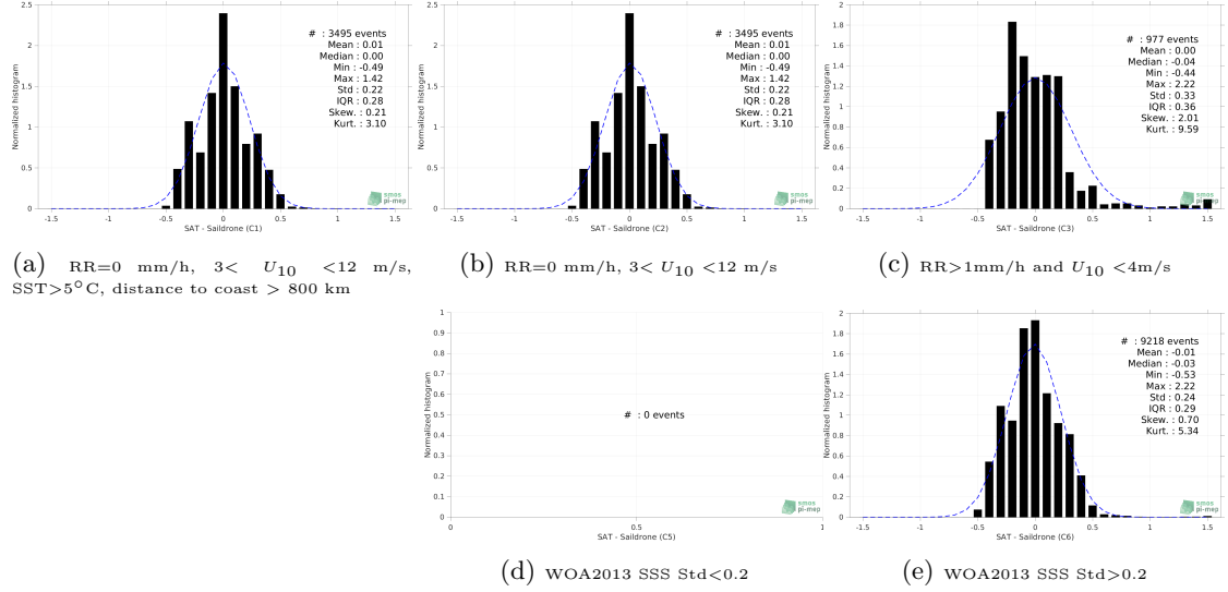
Figure 12: Normalized histogram of \Delta SSS (SMAP SSS L3 v5.0 - 8-Day running (JPL) - Saildrone) for 5 different subdatasets corresponding to: RR=0 mm/h, 3 < U_{10} < 12 m/s, SST > 5°C, distance to coast > 800 km (a), RR=0 mm/h, 3 < U_{10} < 12 m/s (b), RR > 1mm/h and U_{10} < 4 m/s (c), WOA2013 SSS Std < 0.2 (d), WOA2013 SSS Std > 0.2 (e).
