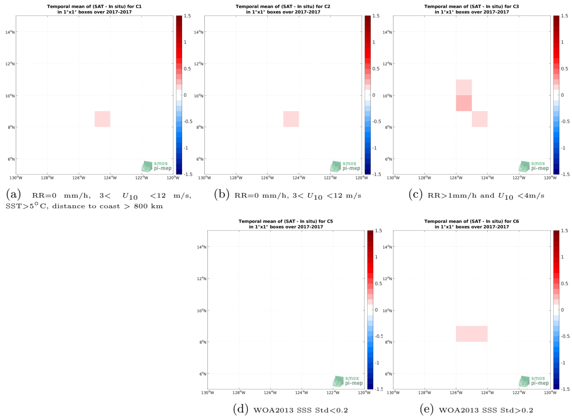
Figure 11: Temporal mean gridded over spatial boxes of size 1^\circ \times 1^\circ of \Delta SSS (SMAP SSS L3 v5.0 - 8-Day running (JPL) - Saifdrone) for 5 different subdatasets corresponding to:RR=0 mm/h, 3 < U_{10} < 12 m/s, SST > 5^\circ\text{C} , distance to coast > 800 km (a), RR=0 mm/h, 3 < U_{10} < 12 m/s (b), RR > 1 mm/h and U_{10} < 4 m/s (c), WOA2013 SSS Std < 0.2 (d), WOA2013 SSS Std > 0.2 (e).
