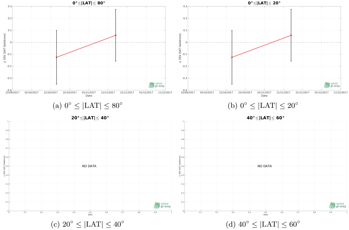
Figure 9: Monthly median (red curves) of \Delta SSS (Satellite - Sailability) and \pm 1 Std (black vertical thick bars) as function of time for all the collected Pi-MEP match-up pairs estimated over the SPURS 2 Pi-MEP region and for the full satellite product period are shown for different latitude bands: (a) 80°S-80°N, (b) 20°S-20°N, (c) 40°S-20°S and 20°N-40°N and (d) 60°S-40°S and 40°N-60°N.
