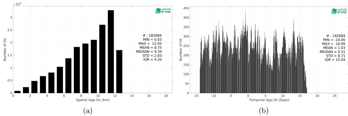
Figure 6: Histograms of the spatial (a) and temporal (b) lags between the location/time of the Waveglider (SPURS 2) measurement and the date of the corresponding SMAP SSS L3 v5.0 - Monthly (JPL) SSS pixel.
