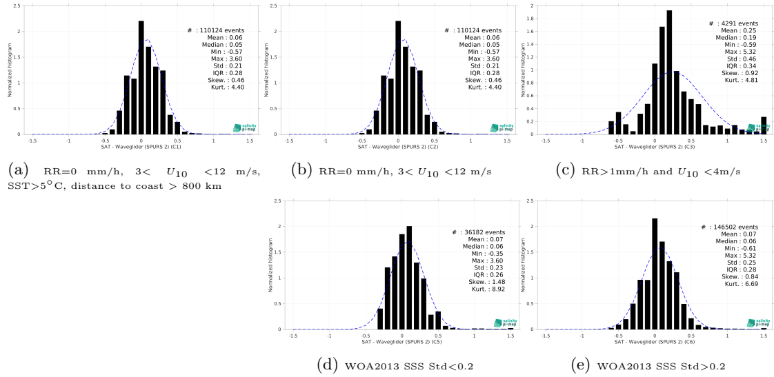
Figure 15: Normalized histogram of \Delta SSS (SMAP SSS L3 v5.0 - Monthly (JPL) - Waveglider (SPURS 2)) for 5 different subdatasets corresponding to: RR=0 mm/h, 3 < U_{10} < 12 m/s, SST>5°C, distance to coast > 800 km (a), RR=0 mm/h, 3 < U_{10} < 12 m/s (b), RR>1mm/h and U_{10} < 4 m/s (c), WOA2013 SSS Std<0.2 (d), WOA2013 SSS Std>0.2 (e).
