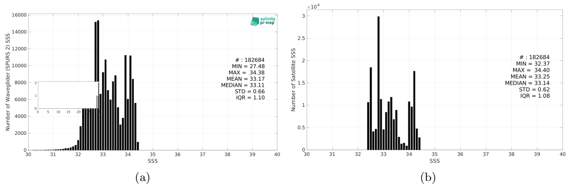
Figure 3: Histograms of SSS from Waveglider (SPURS 2) (a) and SMAP SSS L3 v5.0 - Monthly (JPL) (b) considering all match-up pairs per bins of 0.1 over the SPURS 2 Pi-MEP region and for the full satellite product period.
