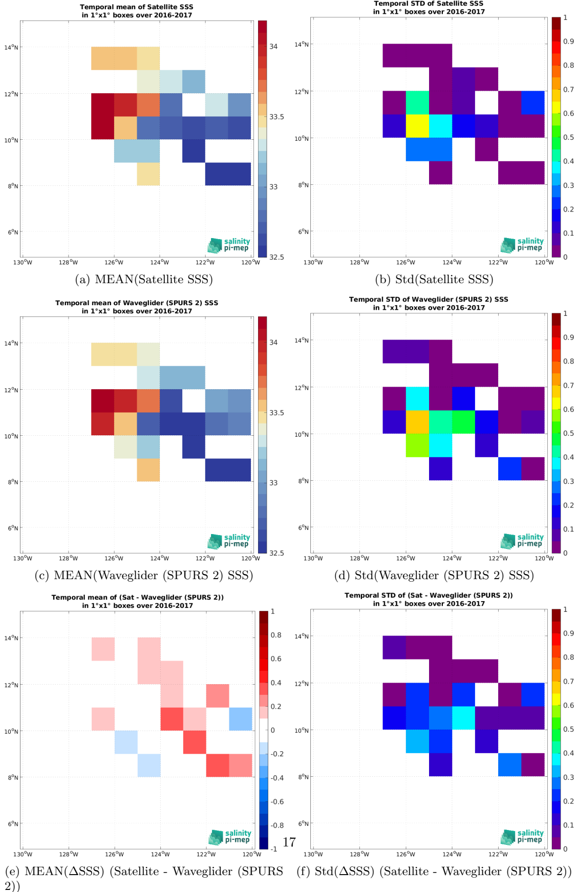
Figure 7: Temporal mean (left) and Std (right) of SSS from SMAP SSS L3 v5.0 - Monthly (JPL) (top), Waveglider (SPURS 2) (middle), and of \Delta SSS (Satellite - Waveglider (SPURS 2)). Only match-up pairs are used to generate these maps.
