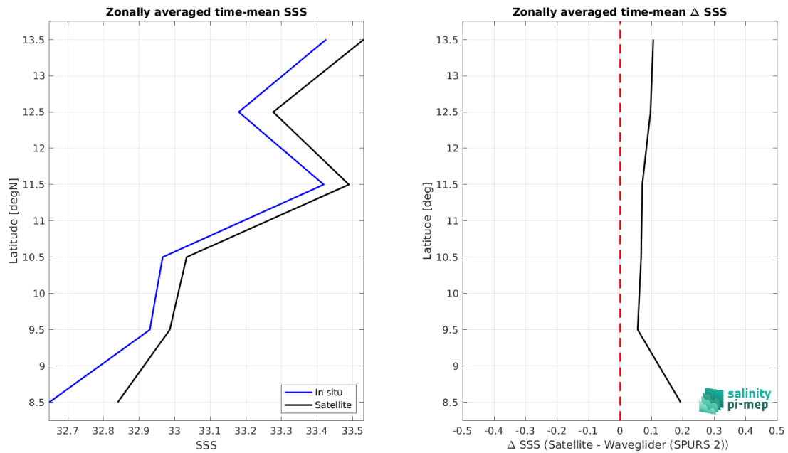
Figure 9: Left panel: Zonal mean SSS from SMAP SSS L3 v5.0 - Monthly (JPL) satellite product (black) and from Waveglider (SPURS 2) (blue). Right panel: Zonal mean of \Delta SSS (Satellite - Waveglider (SPURS 2)) for all the collected Pi-MEP match-up pairs estimated over the full satellite product period.
