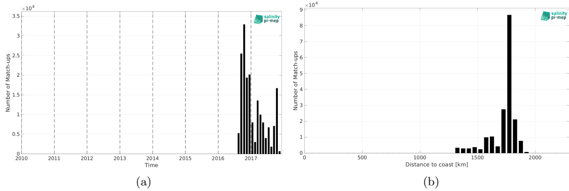
Figure 2: Number of match-ups between Waveglider (SPURS 2) and SMAP SSS L3 v5.0 - Monthly (JPL) SSS as a function of time (a) and as function of the distance to coast (b) over the SPURS 2 Pi-MEP region and for the full satellite product period.
