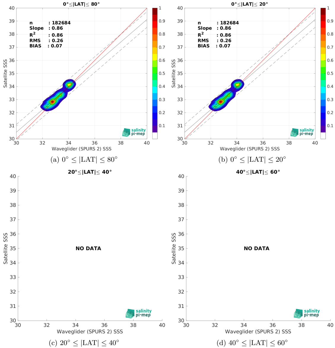
Figure 10: Contour maps of the concentration of SMAP SSS L3 v5.0 - Monthly (JPL) SSS (y-axis) versus Waveglider (SPURS 2) SSS (x-axis) at match-up pairs for different latitude bands. For each plot, the red line shows x=y . The black thin and dashed lines indicate a linear fit through the data cloud and the \pm 95\% confidence levels, respectively. The number match-up pairs n , the slope and R^2 coefficient of the linear fit, the root mean square (RMS) and the mean bias between satellite and in situ data are indicated for each latitude band in each plots.
