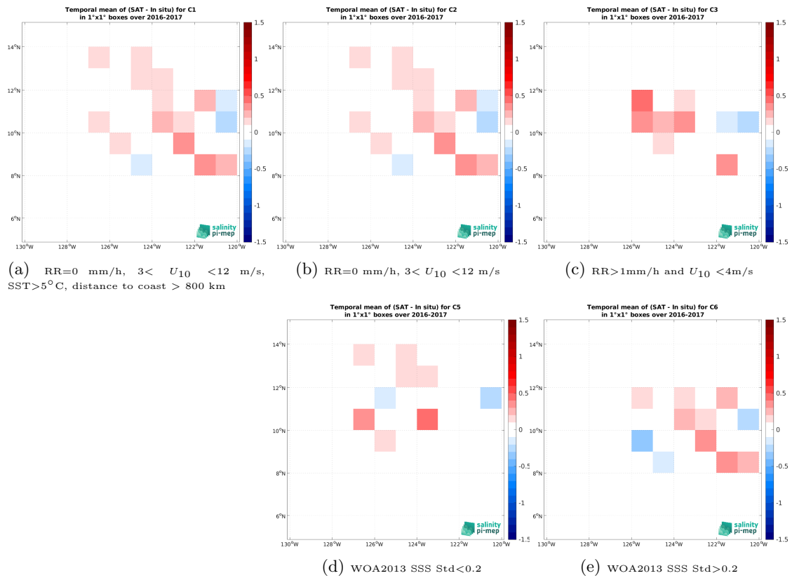
Figure 14: Temporal mean gridded over spatial boxes of size 1^\circ \times 1^\circ of \Delta\text{SSS} (SMAP SSS L3 v5.0 - Monthly (JPL) - Waveglider (SPURS 2)) for 5 different subdatasets corresponding to:RR=0 mm/h, 3 < U_{10} < 12 m/s, SST > 5°C, distance to coast > 800 km (a), RR=0 mm/h, 3 < U_{10} < 12 m/s (b), RR > 1mm/h and U_{10} < 4 m/s (c), WOA2013 SSS Std < 0.2 (d), WOA2013 SSS Std > 0.2 (e).
