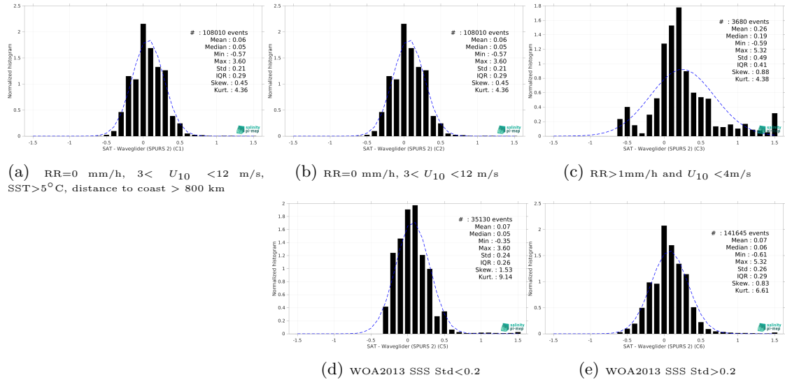
Figure 15: Normalized histogram of \Delta SSS (SMAP SSS L3 v5.0 - Monthly (JPL) - Waveglider (SPURS 2)) for 5 different subdatasets corresponding to: RR=0 mm/h, 3 < U_{10} < 12 m/s, SST > 5°C, distance to coast > 800 km (a), RR=0 mm/h, 3 < U_{10} < 12 m/s (b), RR > 1mm/h and U_{10} < 4 m/s (c), WOA2013 SSS Std < 0.2 (d), WOA2013 SSS Std > 0.2 (e).
