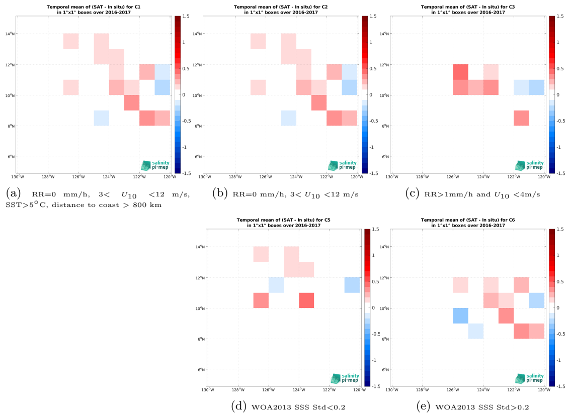
Figure 14: Temporal mean gridded over spatial boxes of size 1^\circ \times 1^\circ of \Delta SSS (SMAP SSS L3 v5.0 - Monthly (JPL) - Waveglider (SPURS 2)) for 5 different subdatasets corresponding to:RR=0 mm/h, 3 < U_{10} < 12 m/s, SST >5^\circ C, distance to coast > 800 km (a), RR=0 mm/h, 3 < U_{10} < 12 m/s (b), RR >1 mm/h and U_{10} < 4 m/s (c), WOA2013 SSS Std <0.2 (d), WOA2013 SSS Std >0.2 (e).
