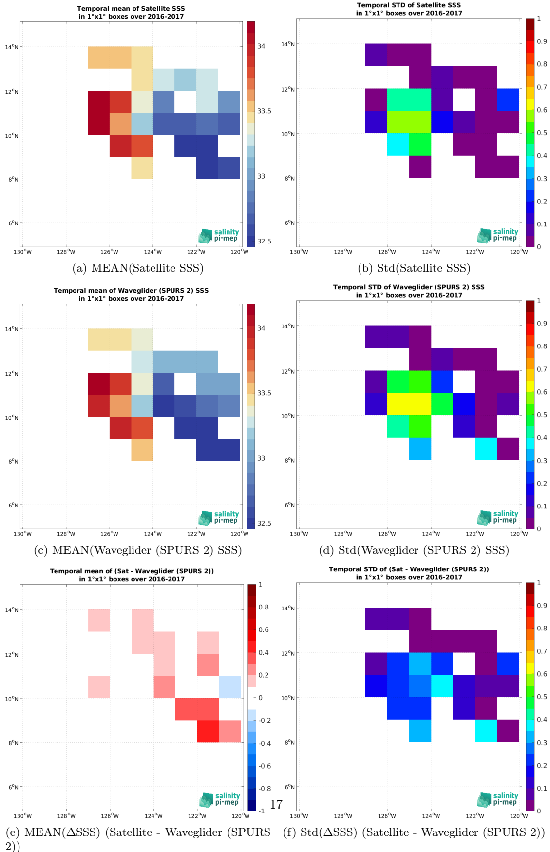
Figure 6: Temporal mean (left) and Std (right) of SSS from SMAP SSS L3 v5.0 - Monthly (JPL) (top), Waveglider (SPURS 2) (middle), and of \Delta SSS (Satellite - Waveglider (SPURS 2)). Only match-up pairs are used to generate these maps.
