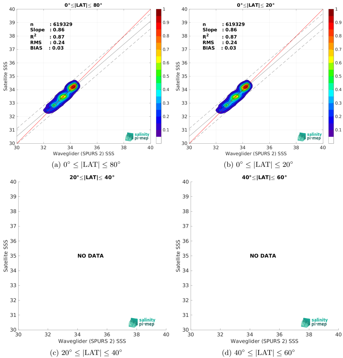
Figure 9: Contour maps of the concentration of SMAP SSS L3 v5.0 - Monthly (JPL) SSS (y-axis) versus Waveglider (SPURS 2) SSS (x-axis) at match-up pairs for different latitude bands. For each plot, the red line shows x=y . The black thin and dashed lines indicate a linear fit through the data cloud and the \pm 95\% confidence levels, respectively. The number match-up pairs n , the slope and R^2 coefficient of the linear fit, the root mean square (RMS) and the mean bias between satellite and in situ data are indicated for each latitude band in each plots.
