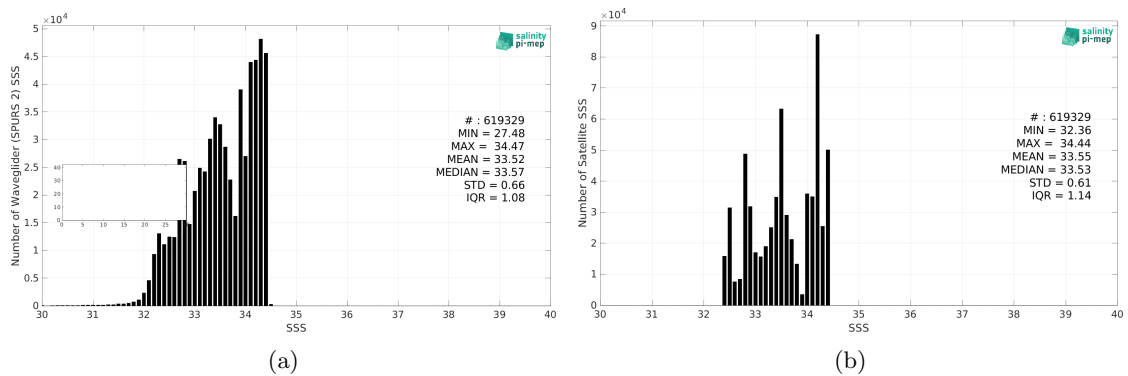
Figure 2: Histograms of SSS from Waveglider (SPURS 2) (a) and SMAP SSS L3 v5.0 - Monthly (JPL) (b) considering all match-up pairs per bins of 0.1 over the SPURS 2 Pi-MEP region and for the full satellite product period.
