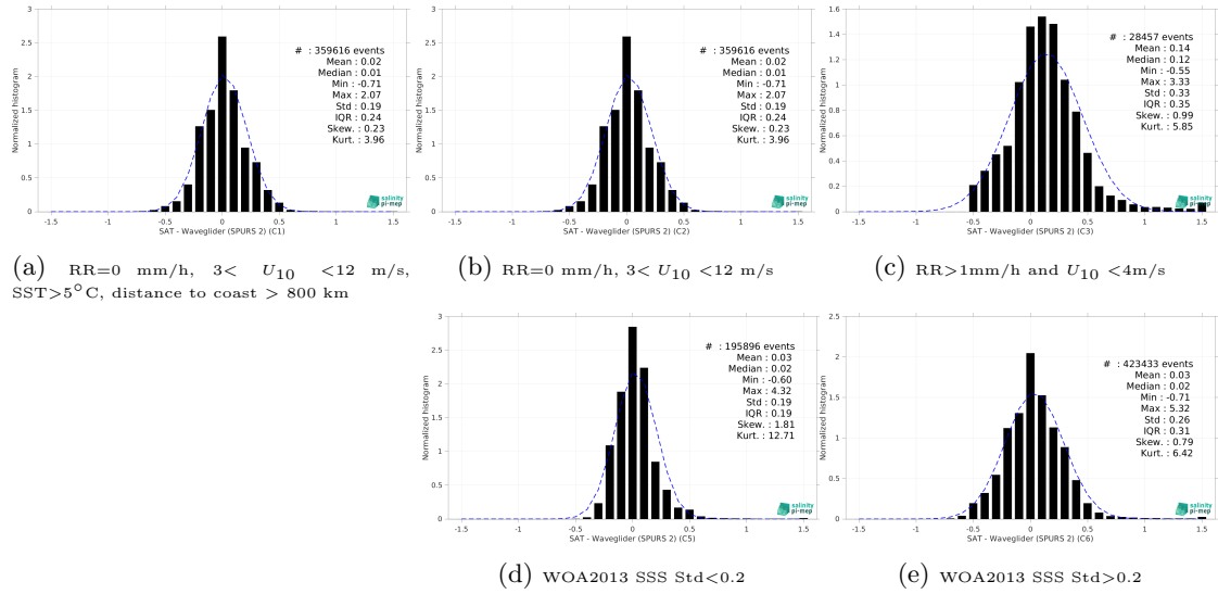
Figure 13: Normalized histogram of \Delta SSS (SMAP SSS L3 v5.0 - Monthly (JPL) - Waveglider (SPURS 2)) for 5 different subdatasets corresponding to: RR=0 mm/h, 3 < U_{10} < 12 m/s, SST > 5°C, distance to coast > 800 km (a), RR=0 mm/h, 3 < U_{10} < 12 m/s (b), RR > 1mm/h and U_{10} < 4 m/s (c), WOA2013 SSS Std < 0.2 (d), WOA2013 SSS Std > 0.2 (e).
