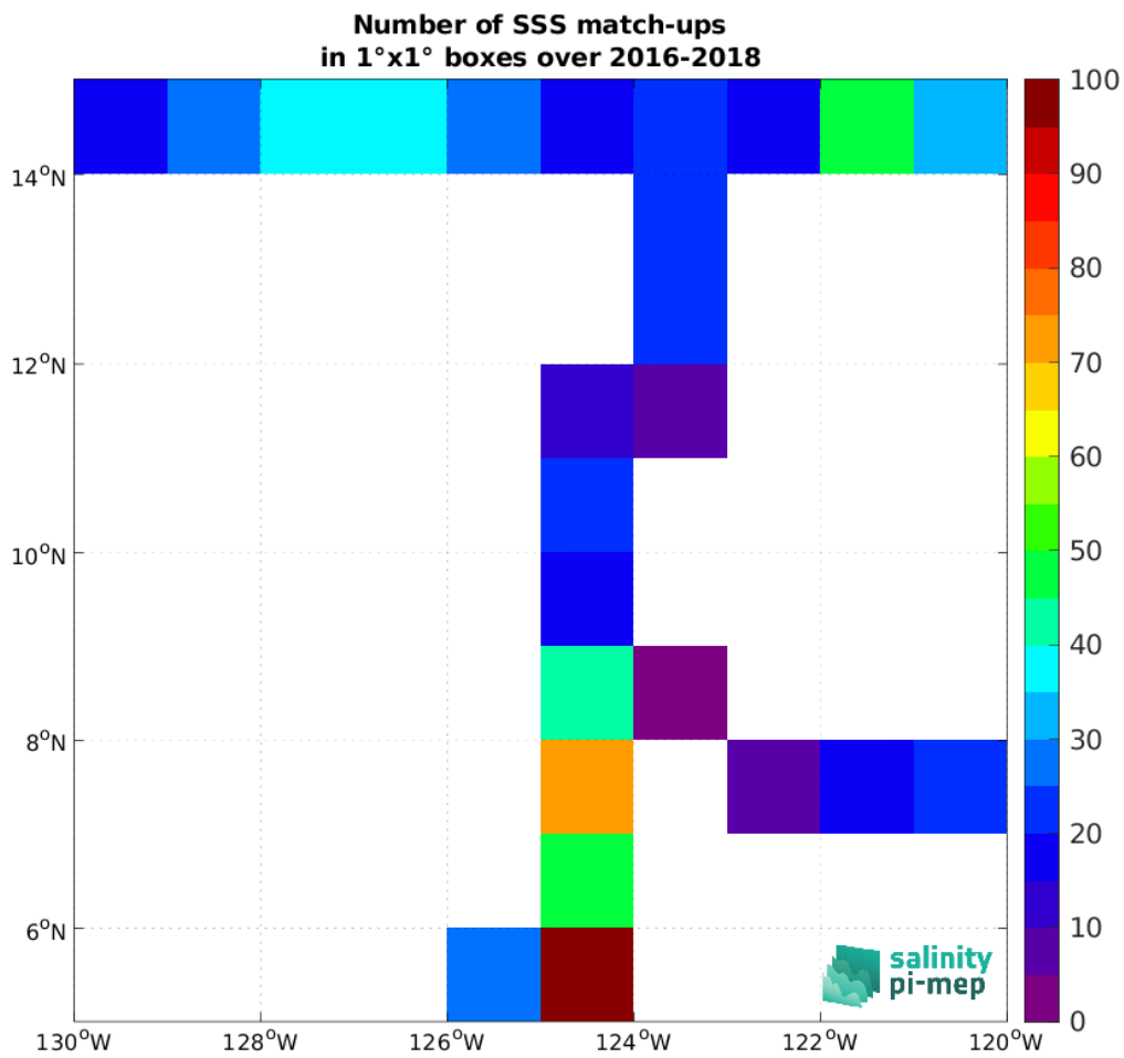
Figure 5: Number of SSS match-ups between TSG (SAMOS) SSS and the SMAP SSS L3 v5.0 - Monthly (JPL) SSS product for the SPURS 2 Pi-MEP region over 1^\circ \times 1^\circ boxes and for the full satellite product period.
