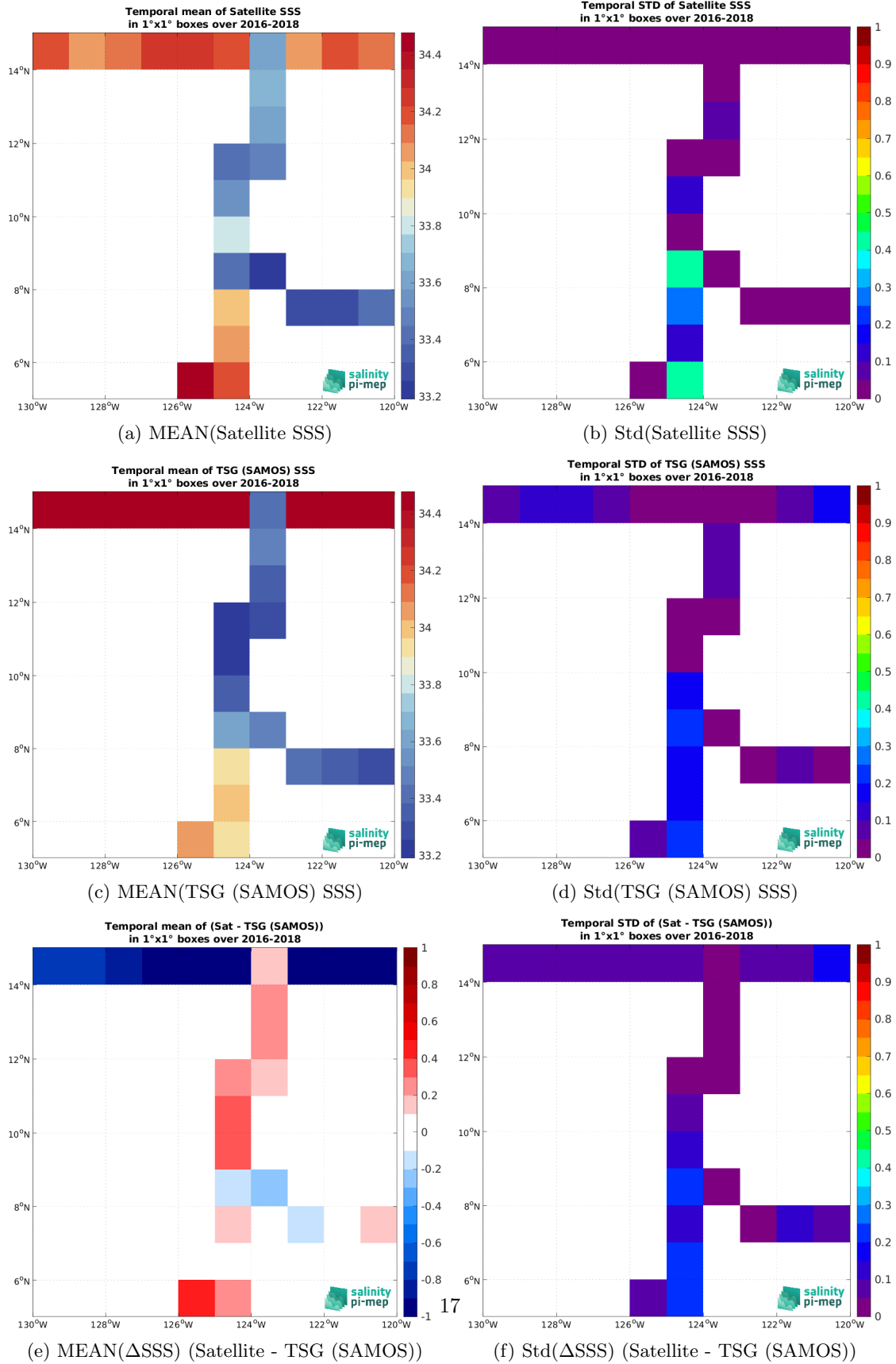
Figure 7: Temporal mean (left) and Std (right) of SSS from SMAP SSS L3 v5.0 - Monthly (JPL) (top), TSG (SAMOS) (middle), and of \Delta SSS (Satellite - TSG (SAMOS)). Only match-up pairs are used to generate these maps.
