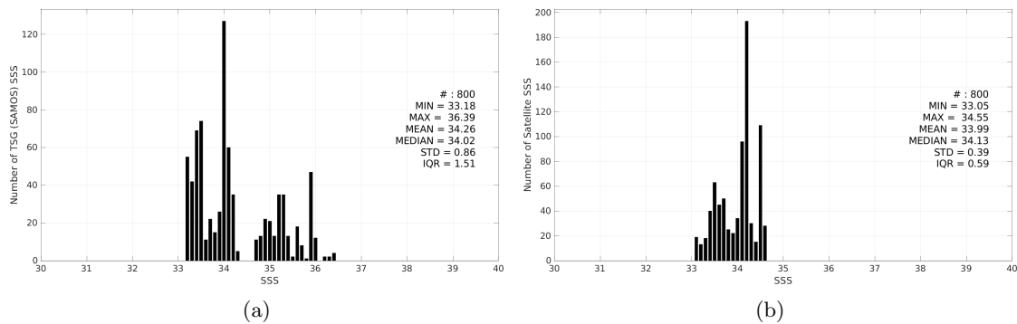
Figure 3: Histograms of SSS from TSG (SAMOS) (a) and SMAP SSS L3 v5.0 - Monthly (JPL) (b) considering all match-up pairs per bins of 0.1 over the SPURS 2 Pi-MEP region and for the full satellite product period.
