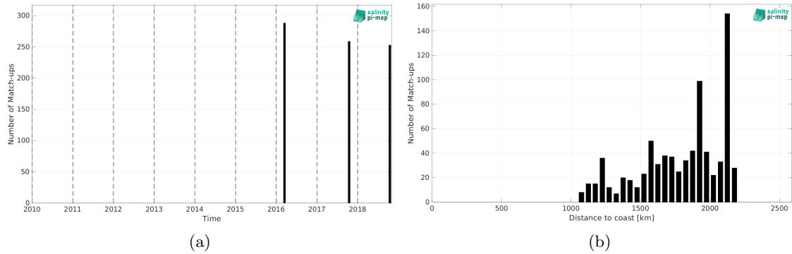
Figure 2: Number of match-ups between TSG (SAMOS) and SMAP SSS L3 v5.0 - Monthly (JPL) SSS as a function of time (a) and as function of the distance to coast (b) over the SPURS 2 Pi-MEP region and for the full satellite product period.
