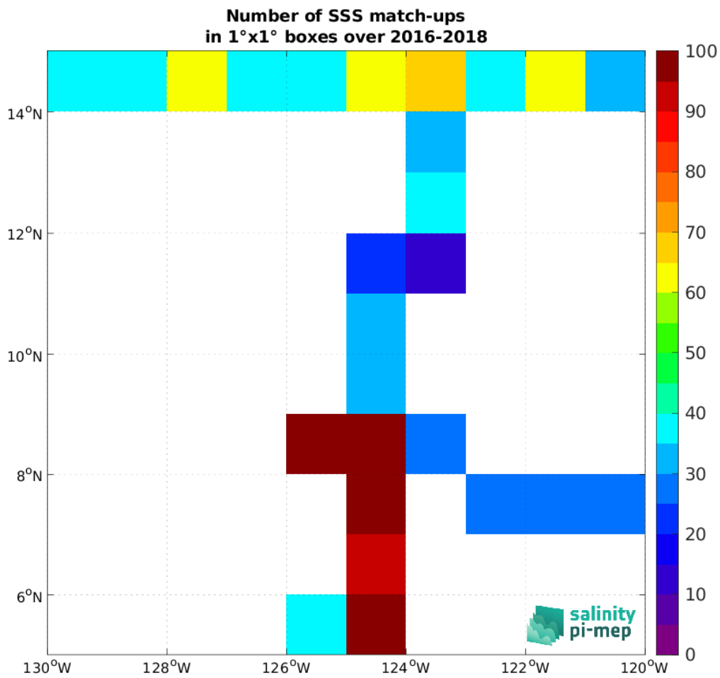
Figure 4: Number of SSS match-ups between TSG (SAMOS) SSS and the SMAP SSS L3 v5.0 - Monthly (JPL) SSS product for the SPURS 2 Pi-MEP region over 1^\circ \times 1^\circ boxes and for the full satellite product period.
