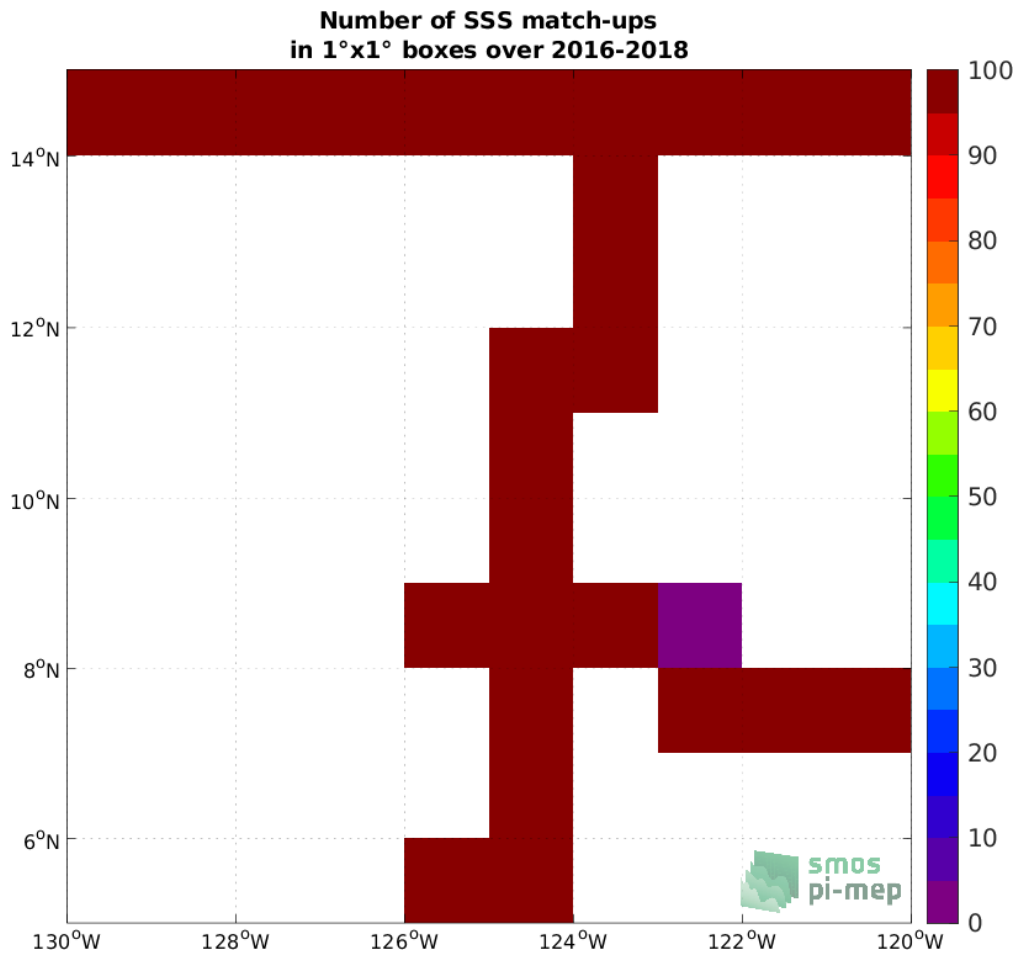
Figure 4: Number of SSS match-ups between TSG (SAMOS) SSS and the SMAP SSS L3 v5.0 - Monthly (JPL) SSS product for the SPURS 2 Pi-MEP region over 1°x1° boxes and for the full satellite product period.
