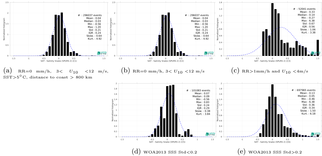
Figure 15: Normalized histogram of \Delta SSS (SMAP SSS L3 v5.0 - Monthly (JPL) - Salinity Snake (SPURS 2)) for 5 different subdatasets corresponding to: RR=0 mm/h, 3 < U_{10} < 12 m/s, SST>5°C, distance to coast > 800 km (a), RR=0 mm/h, 3 < U_{10} < 12 m/s (b), RR>1mm/h and U_{10} < 4 m/s (c), WOA2013 SSS Std<0.2 (d), WOA2013 SSS Std>0.2 (e).
