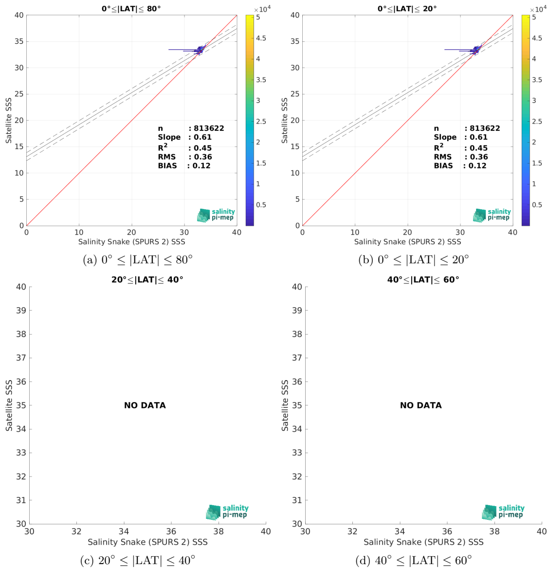
Figure 10: Contour maps of the concentration of SMAP SSS L3 v5.0 - Monthly (JPL) SSS (y-axis) versus Salinity Snake (SPURS 2) SSS (x-axis) at match-up pairs for different latitude bands. For each plot, the red line shows x=y . The black thin and dashed lines indicate a linear fit through the data cloud and the \pm 95\% confidence levels, respectively. The number match-up pairs n , the slope and R^2 coefficient of the linear fit, the root mean square (RMS) and the mean bias between satellite and in situ data are indicated for each latitude band in each plots.
