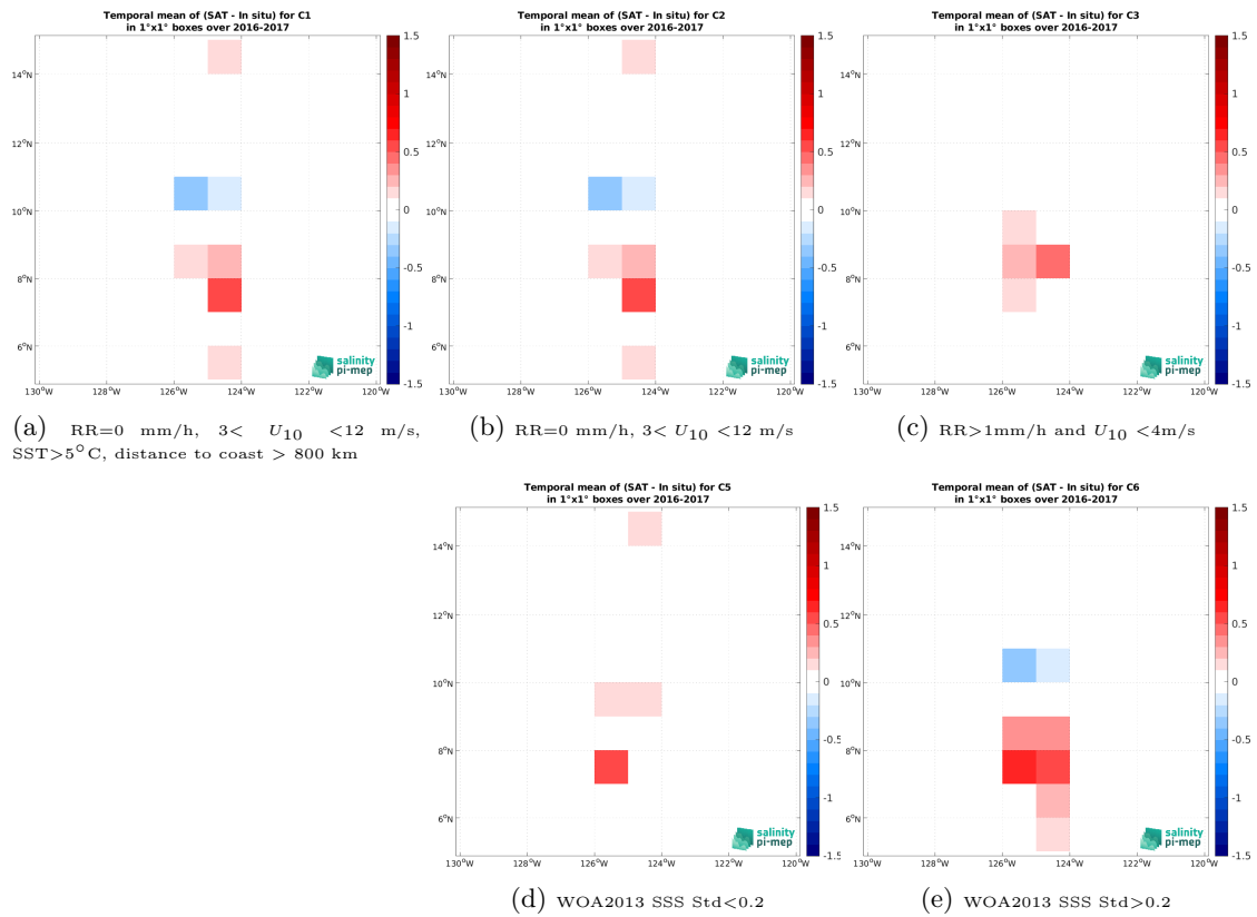
Figure 14: Temporal mean gridded over spatial boxes of size 1^\circ \times 1^\circ of \Delta\text{SSS} (SMAP SSS L3 v5.0 - Monthly (JPL) - Salinity Snake (SPURS 2)) for 5 different subdatasets corresponding to:RR=0 mm/h, 3 < U_{10} < 12 m/s, SST>5°C, distance to coast > 800 km (a), RR=0 mm/h, 3 < U_{10} < 12 m/s (b), RR>1mm/h and U_{10} < 4 m/s (c), WOA2013 SSS Std<0.2 (d), WOA2013 SSS Std>0.2 (e).
