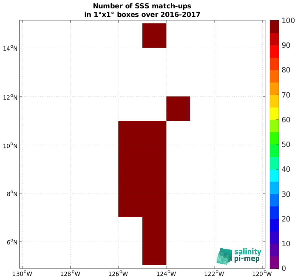
Figure 5: Number of SSS match-ups between Salinity Snake (SPURS 2) SSS and the SMAP SSS L3 v5.0 - Monthly (JPL) SSS product for the SPURS 2 Pi-MEP region over 1^\circ \times 1^\circ boxes and for the full satellite product period.
