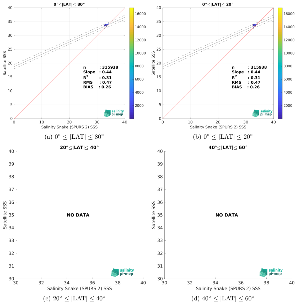
Figure 10: Contour maps of the concentration of SMAP SSS L3 v5.0 - Monthly (JPL) SSS (y-axis) versus Salinity Snake (SPURS 2) SSS (x-axis) at match-up pairs for different latitude bands. For each plot, the red line shows x=y . The black thin and dashed lines indicate a linear fit through the data cloud and the \pm 95\% confidence levels, respectively. The number match-up pairs n , the slope and R^2 coefficient of the linear fit, the root mean square (RMS) and the mean bias between satellite and in situ data are indicated for each latitude band in each plots.
