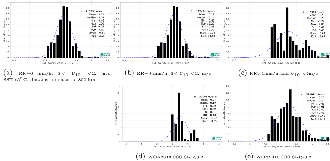
Figure 15: Normalized histogram of \Delta SSS (SMAP SSS L3 v5.0 - Monthly (JPL) - Salinity Snake (SPURS 2)) for 5 different subdatasets corresponding to: RR=0 mm/h, 3 < U_{10} < 12 m/s, SST > 5°C, distance to coast > 800 km (a), RR=0 mm/h, 3 < U_{10} < 12 m/s (b), RR > 1mm/h and U_{10} < 4 m/s (c), WOA2013 SSS Std < 0.2 (d), WOA2013 SSS Std > 0.2 (e).
