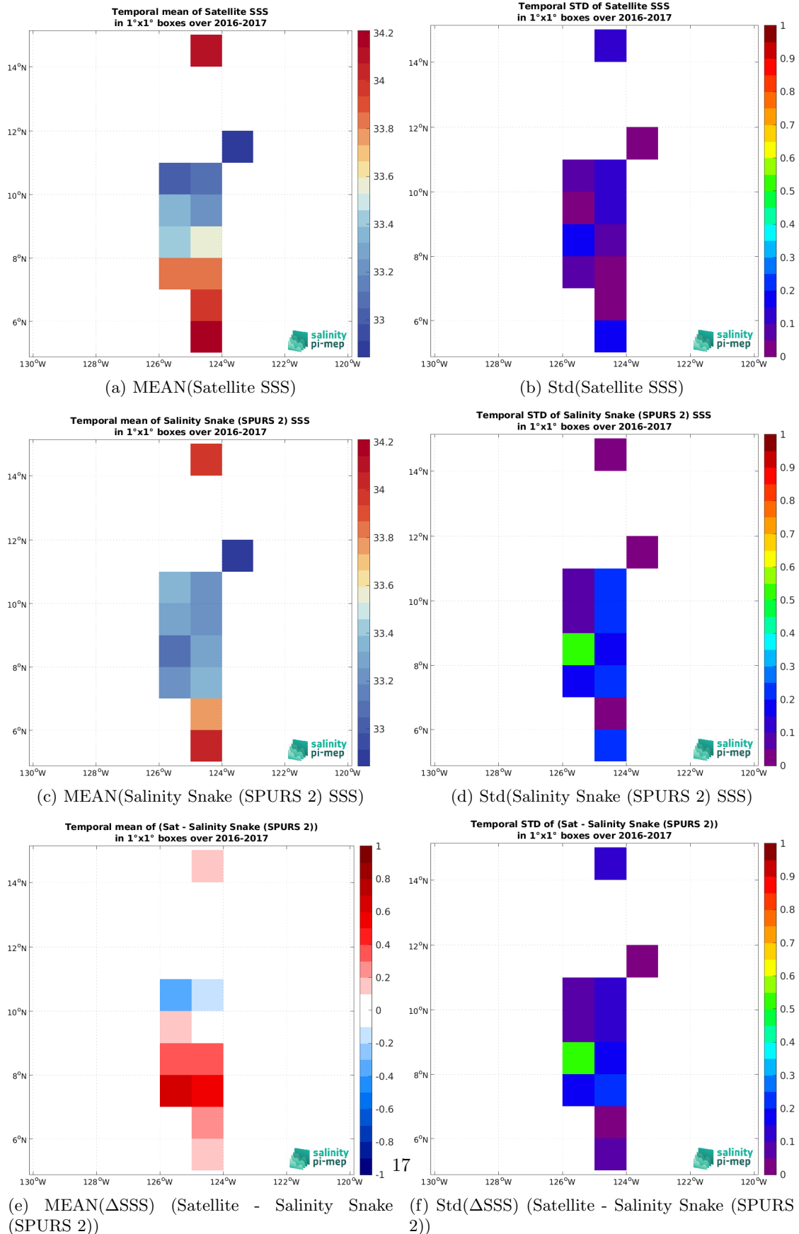
Figure 7: Temporal mean (left) and Std (right) of SSS from SMAP SSS L3 v5.0 - Monthly (JPL) (top), Salinity Snake (SPURS 2) (middle), and of \Delta SSS (Satellite - Salinity Snake (SPURS 2)). Only match-up pairs are used to generate these maps.
