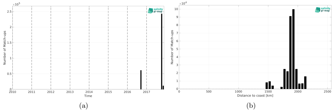
Figure 2: Number of match-ups between Salinity Snake (SPURS 2) and SMAP SSS L3 v5.0 - Monthly (JPL) SSS as a function of time (a) and as function of the distance to coast (b) over the SPURS 2 Pi-MEP region and for the full satellite product period.
