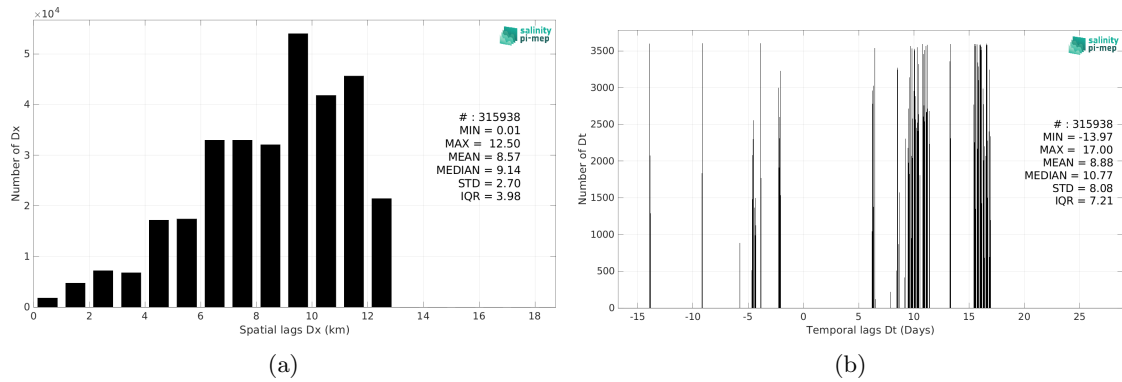
Figure 6: Histograms of the spatial (a) and temporal (b) lags between the location/time of the Salinity Snake (SPURS 2) measurement and the date of the corresponding SMAP SSS L3 v5.0 - Monthly (JPL) SSS pixel.
