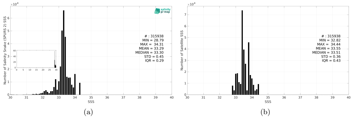
Figure 3: Histograms of SSS from Salinity Snake (SPURS 2) (a) and SMAP SSS L3 v5.0 - Monthly (JPL) (b) considering all match-up pairs per bins of 0.1 over the SPURS 2 Pi-MEP region and for the full satellite product period.
