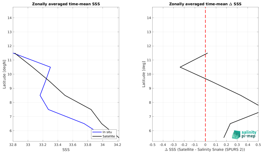
Figure 9: Left panel: Zonal mean SSS from SMAP SSS L3 v5.0 - Monthly (JPL) satellite product (black) and from Salinity Snake (SPURS 2) (blue). Right panel: Zonal mean of \Delta SSS (Satellite - Salinity Snake (SPURS 2)) for all the collected Pi-MEP match-up pairs estimated over the full satellite product period.
