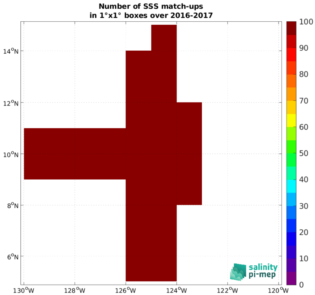
Figure 4: Number of SSS match-ups between Salinity Snake (SPURS 2) SSS and the SMAP SSS L3 v5.0 - Monthly (JPL) SSS product for the SPURS 2 Pi-MEP region over 1^\circ \times 1^\circ boxes and for the full satellite product period.
