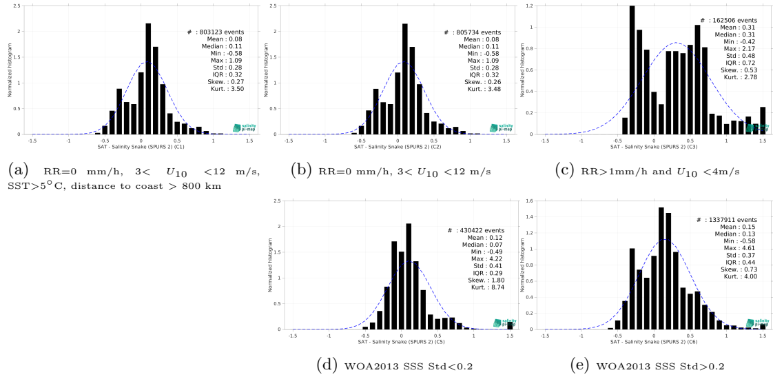
Figure 13: Normalized histogram of \Delta SSS (SMAP SSS L3 v5.0 - Monthly (JPL) - Salinity Snake (SPURS 2)) for 5 different subdatasets corresponding to: RR=0 mm/h, 3 < U_{10} < 12 m/s, SST>5°C, distance to coast > 800 km (a), RR=0 mm/h, 3 < U_{10} < 12 m/s (b), RR>1mm/h and U_{10} < 4 m/s (c), WOA2013 SSS Std<0.2 (d), WOA2013 SSS Std>0.2 (e).
