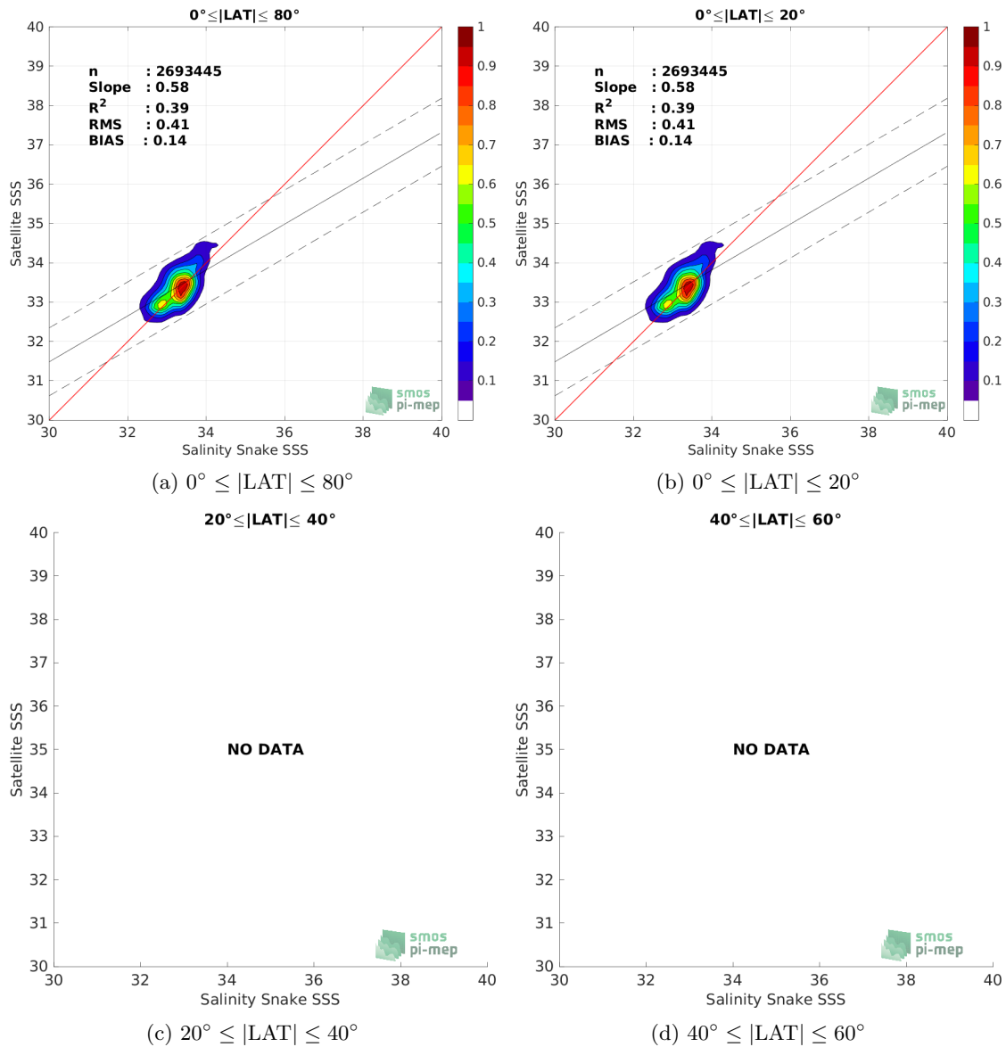
Figure 9: Contour maps of the concentration of SMAP SSS L3 v5.0 - Monthly (JPL) SSS (y-axis) versus Salinity Snake SSS (x-axis) at match-up pairs for different latitude bands. For each plot, the red line shows x=y . The black thin and dashed lines indicate a linear fit through the data cloud and the \pm 95\% confidence levels, respectively. The number match-up pairs n , the slope and R^2 coefficient of the linear fit, the root mean square (RMS) and the mean bias between satellite and in situ data are indicated for each latitude band in each plots.
