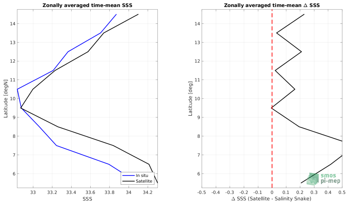
Figure 8: Left panel: Zonal mean SSS from SMAP SSS L3 v5.0 - Monthly (JPL) satellite product (black) and from Salinity Snake (blue). Right panel: Zonal mean of \Delta SSS (Satellite - Salinity Snake) for all the collected Pi-MEP match-up pairs estimated over the full satellite product period.
