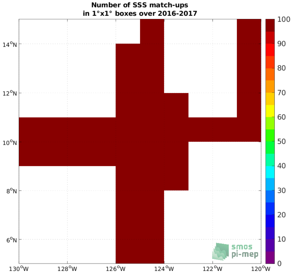
Figure 4: Number of SSS match-ups between Salinity Snake SSS and the SMAP SSS L3 v5.0 - Monthly (JPL) SSS product for the SPURS 2 Pi-MEP region over 1°x1° boxes and for the full satellite product period.
