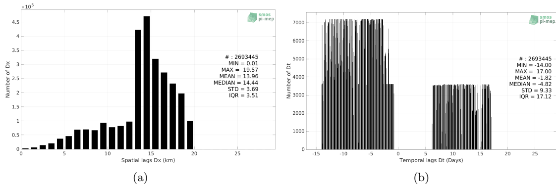
Figure 5: Histograms of the spatial (a) and temporal (b) lags between the location/time of the Salinity Snake measurement and the date of the corresponding SMAP SSS L3 v5.0 - Monthly (JPL) SSS pixel.
