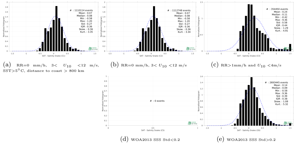
Figure 13: Normalized histogram of \Delta SSS (SMAP SSS L3 v5.0 - Monthly (JPL) - Salinity Snake) for 5 different subdatasets corresponding to: RR=0 mm/h, 3 < U_{10} < 12 m/s, SST > 5°C, distance to coast > 800 km (a), RR=0 mm/h, 3 < U_{10} < 12 m/s (b), RR > 1mm/h and U_{10} < 4 m/s (c), WOA2013 SSS Std < 0.2 (d), WOA2013 SSS Std > 0.2 (e).
