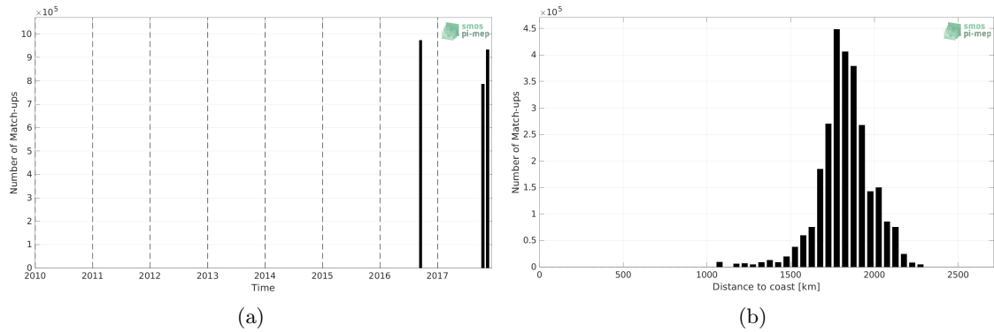
Figure 1: Number of match-ups between Salinity Snake and SMAP SSS L3 v5.0 - Monthly (JPL) SSS as a function of time (a) and as function of the distance to coast (b) over the SPURS 2 Pi-MEP region and for the full satellite product period.
