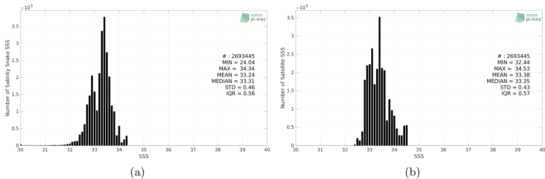
Figure 2: Histograms of SSS from Salinity Snake (a) and SMAP SSS L3 v5.0 - Monthly (JPL) (b) considering all match-up pairs per bins of 0.1 over the SPURS 2 Pi-MEP region and for the full satellite product period.
