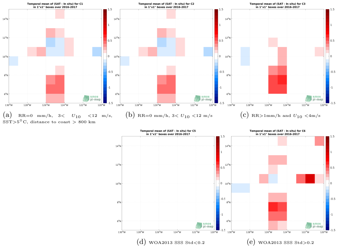
Figure 12: Temporal mean gridded over spatial boxes of size 1^\circ \times 1^\circ of \Delta SSS (SMAP SSS L3 v5.0 - Monthly (JPL) - Salinity Snake) for 5 different subdatasets corresponding to:RR=0 mm/h, 3 < U_{10} < 12 m/s, SST > 5°C, distance to coast > 800 km (a), RR=0 mm/h, 3 < U_{10} < 12 m/s (b), RR > 1mm/h and U_{10} < 4 m/s (c), WOA2013 SSS Std < 0.2 (d), WOA2013 SSS Std > 0.2 (e).
