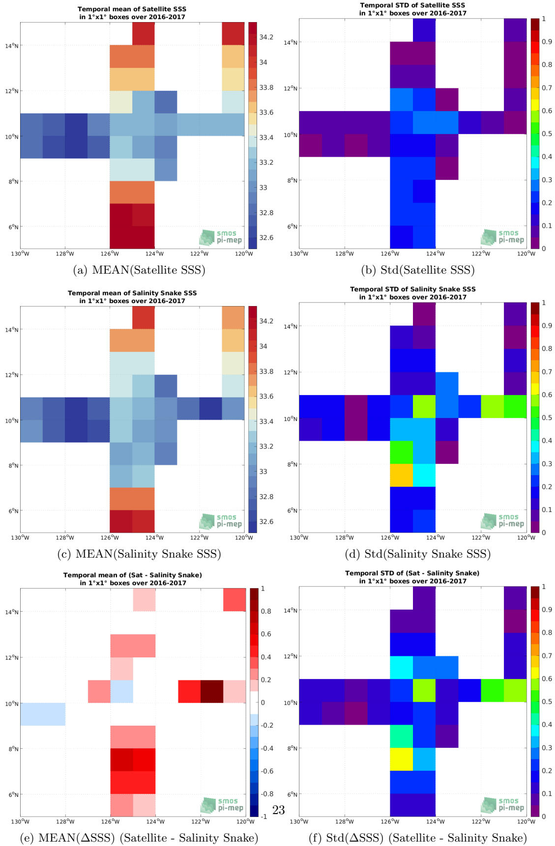
Figure 6: Temporal mean (left) and Std (right) of SSS from SMAP SSS L3 v5.0 - Monthly (JPL) (top), Salinity Snake (middle), and of \Delta SSS (Satellite - Salinity Snake). Only match-up pairs are used to generate these maps.
