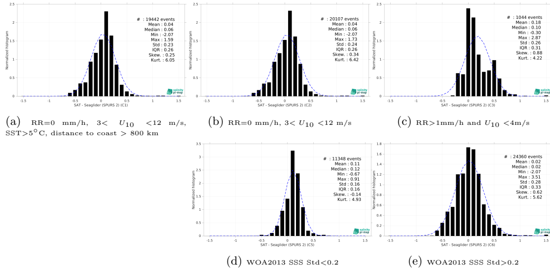
Figure 15: Normalized histogram of \Delta SSS (SMAP SSS L3 v5.0 - Monthly (JPL) - Seaglider (SPURS 2)) for 5 different subdatasets corresponding to: RR=0 mm/h, 3 < U_{10} < 12 m/s, SST > 5°C, distance to coast > 800 km (a), RR=0 mm/h, 3 < U_{10} < 12 m/s (b), RR > 1mm/h and U_{10} < 4 m/s (c), WOA2013 SSS Std < 0.2 (d), WOA2013 SSS Std > 0.2 (e).
