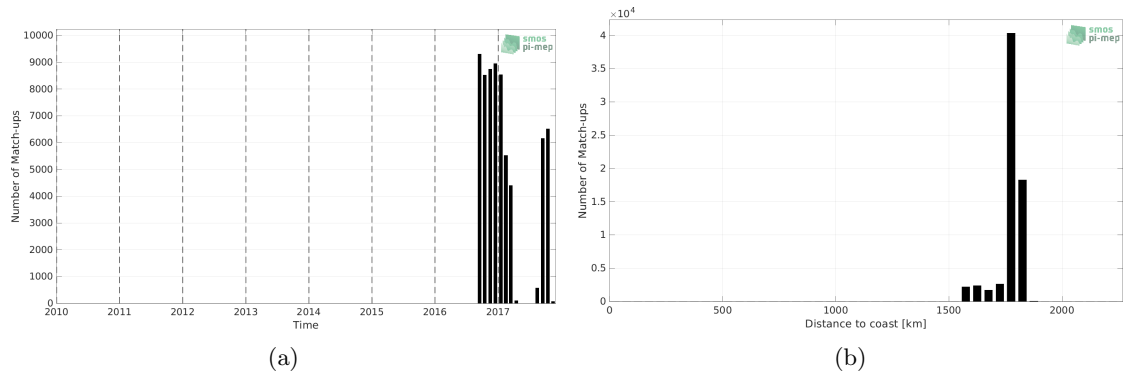
Figure 1: Number of match-ups between Seagliders (SPURS 2) and SMAP SSS L3 v5.0 - Monthly (JPL) SSS as a function of time (a) and as function of the distance to coast (b) over the SPURS 2 Pi-MEP region and for the full satellite product period.
