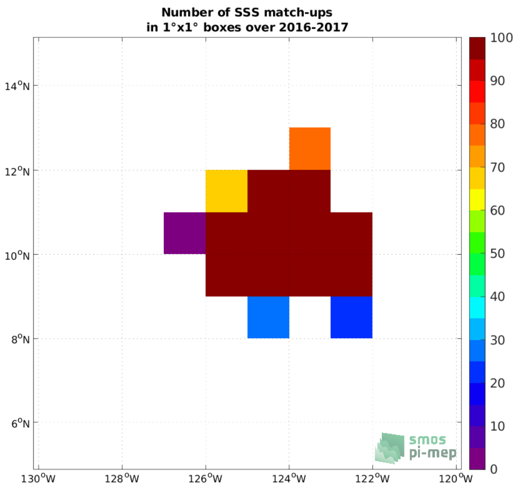
Figure 4: Number of SSS match-ups between Seaglider (SPURS 2) SSS and the SMAP SSS L3 v5.0 - Monthly (JPL) SSS product for the SPURS 2 Pi-MEP region over 1^\circ \times 1^\circ boxes and for the full satellite product period.
