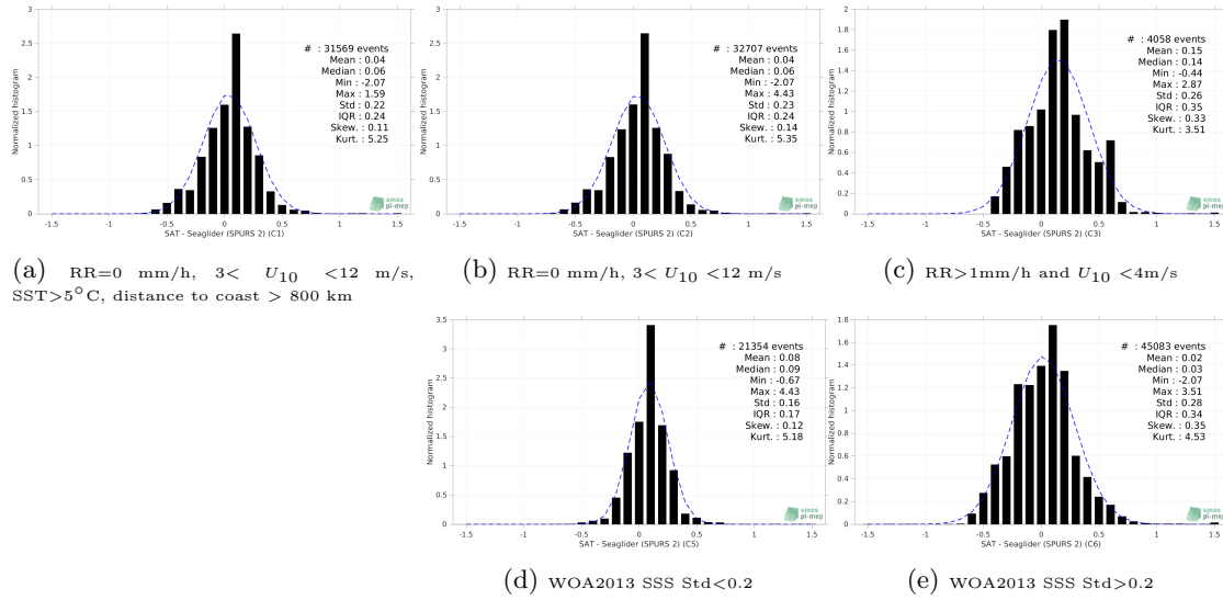
Figure 13: Normalized histogram of \Delta SSS (SMAP SSS L3 v5.0 - Monthly (JPL) - Seaglider (SPURS 2)) for 5 different subdatasets corresponding to: RR=0 mm/h, 3 < U_{10} < 12 m/s, SST>5°C, distance to coast > 800 km (a), RR=0 mm/h, 3 < U_{10} < 12 m/s (b), RR>1mm/h and U_{10} < 4 m/s (c), WOA2013 SSS Std<0.2 (d), WOA2013 SSS Std>0.2 (e).
