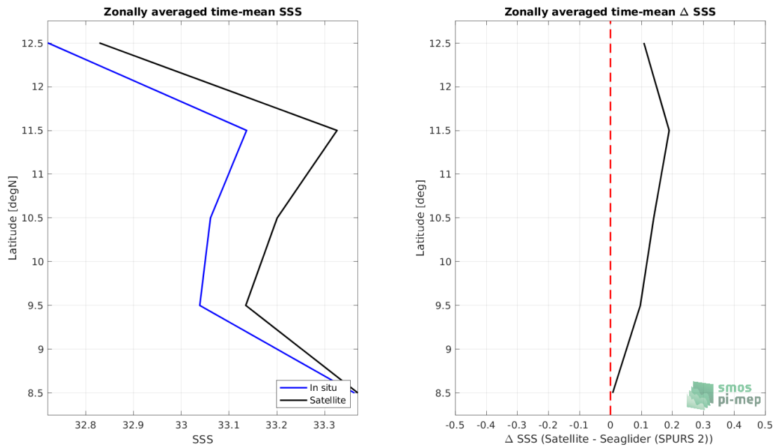
Figure 8: Left panel: Zonal mean SSS from SMAP SSS L3 v5.0 - Monthly (JPL) satellite product (black) and from Seaglider (SPURS 2) (blue). Right panel: Zonal mean of \Delta SSS (Satellite - Seaglider (SPURS 2)) for all the collected Pi-MEP match-up pairs estimated over the full satellite product period.
