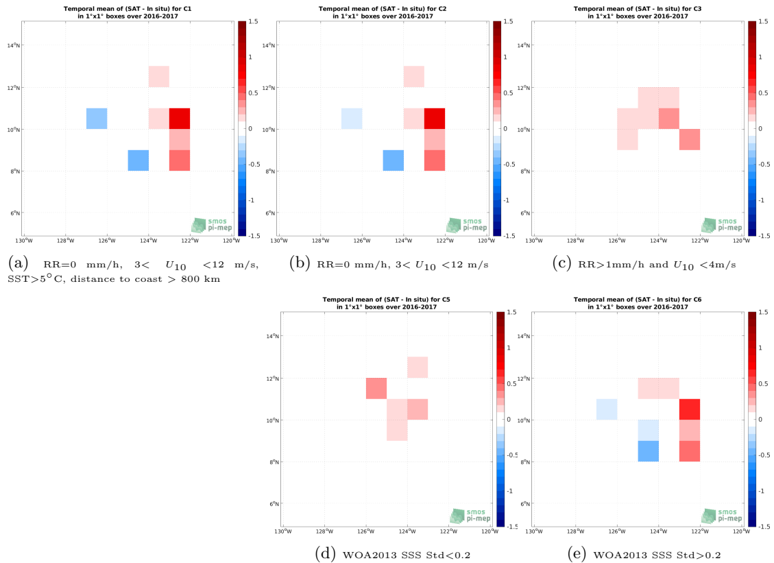
Figure 12: Temporal mean gridded over spatial boxes of size 1^\circ \times 1^\circ of \Delta SSS (SMAP SSS L3 v5.0 - Monthly (JPL) - Seaglider (SPURS 2)) for 5 different subdatasets corresponding to:RR=0 mm/h, 3 < U_{10} < 12 m/s, SST > 5^\circ\text{C} , distance to coast > 800 km (a), RR=0 mm/h, 3 < U_{10} < 12 m/s (b), RR > 1 mm/h and U_{10} < 4 m/s (c), WOA2013 SSS Std < 0.2 (d), WOA2013 SSS Std > 0.2 (e).
