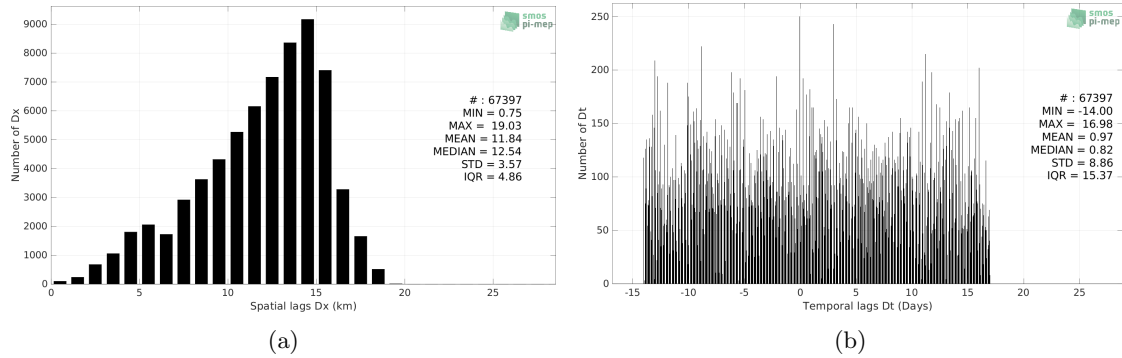
Figure 5: Histograms of the spatial (a) and temporal (b) lags between the location/time of the Seaglider (SPURS 2) measurement and the date of the corresponding SMAP SSS L3 v5.0 - Monthly (JPL) SSS pixel.
