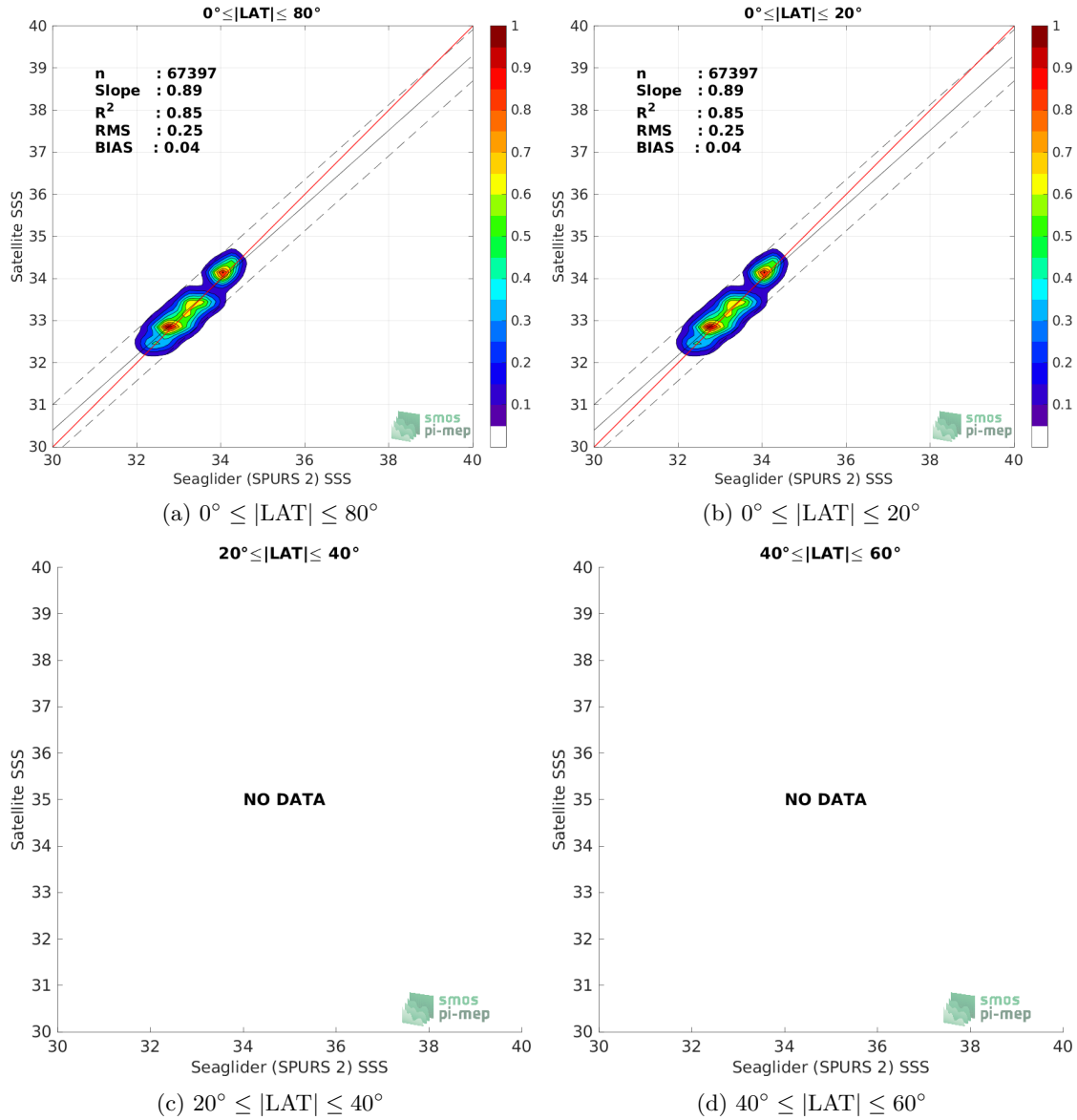
Figure 9: Contour maps of the concentration of SMAP SSS L3 v5.0 - Monthly (JPL) SSS (y-axis) versus Seaglider (SPURS 2) SSS (x-axis) at match-up pairs for different latitude bands. For each plot, the red line shows x=y . The black thin and dashed lines indicate a linear fit through the data cloud and the \pm 95\% confidence levels, respectively. The number match-up pairs n , the slope and R^2 coefficient of the linear fit, the root mean square (RMS) and the mean bias between satellite and in situ data are indicated for each latitude band in each plots.
