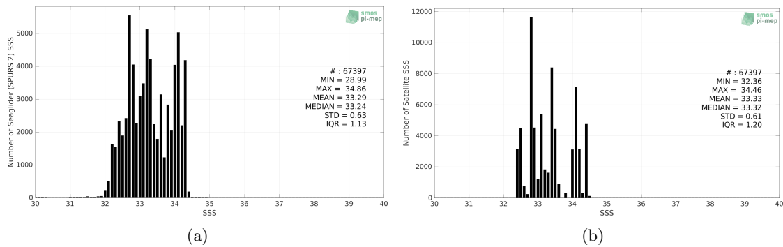
Figure 2: Histograms of SSS from Seagliders (SPURS 2) (a) and SMAP SSS L3 v5.0 - Monthly (JPL) (b) considering all match-up pairs per bins of 0.1 over the SPURS 2 Pi-MEP region and for the full satellite product period.
