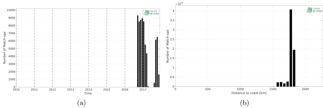
Figure 1: Number of match-ups between Seaglider and SMAP SSS L3 v5.0 - Monthly (JPL) SSS as a function of time (a) and as function of the distance to coast (b) over the SPURS 2 Pi-MEP region and for the full satellite product period.
