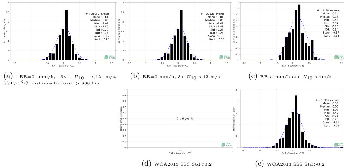
Figure 13: Normalized histogram of \Delta SSS (SMAP SSS L3 v5.0 - Monthly (JPL) - Seaglider) for 5 different subdatasets corresponding to: RR=0 mm/h, 3 < U_{10} < 12 m/s, SST > 5°C, distance to coast > 800 km (a), RR=0 mm/h, 3 < U_{10} < 12 m/s (b), RR > 1mm/h and U_{10} < 4 m/s (c), WOA2013 SSS Std < 0.2 (d), WOA2013 SSS Std > 0.2 (e).
