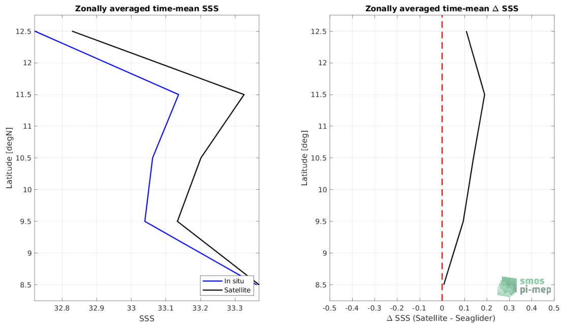
Figure 8: Left panel: Zonal mean SSS from SMAP SSS L3 v5.0 - Monthly (JPL) satellite product (black) and from Seaglider (blue). Right panel: Zonal mean of \Delta SSS (Satellite - Seaglider) for all the collected Pi-MEP match-up pairs estimated over the full satellite product period.
