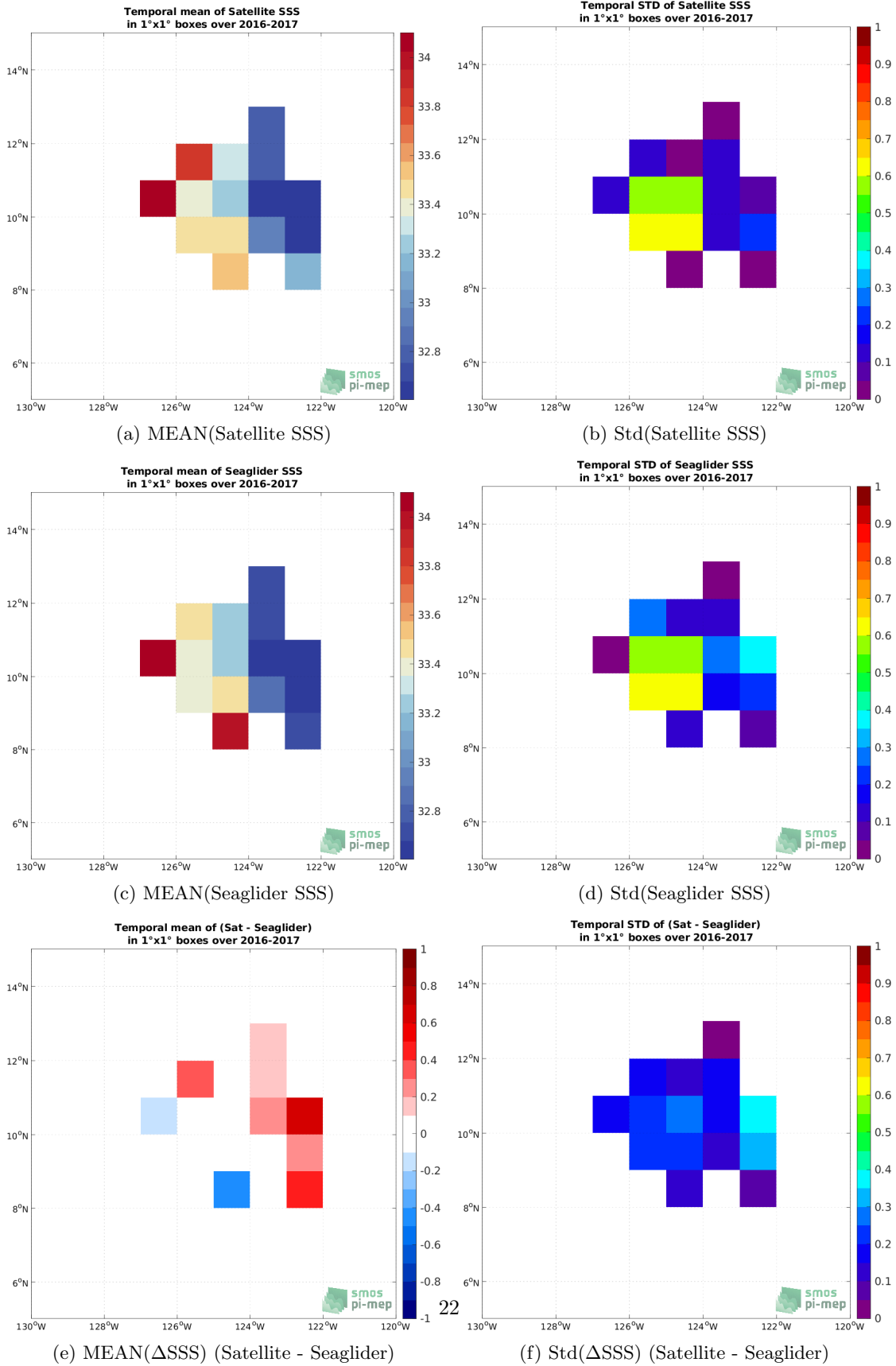
Figure 6: Temporal mean (left) and Std (right) of SSS from SMAP SSS L3 v5.0 - Monthly (JPL) (top), Seaglider (middle), and of \Delta SSS (Satellite - Seaglider). Only match-up pairs are used to generate these maps.
