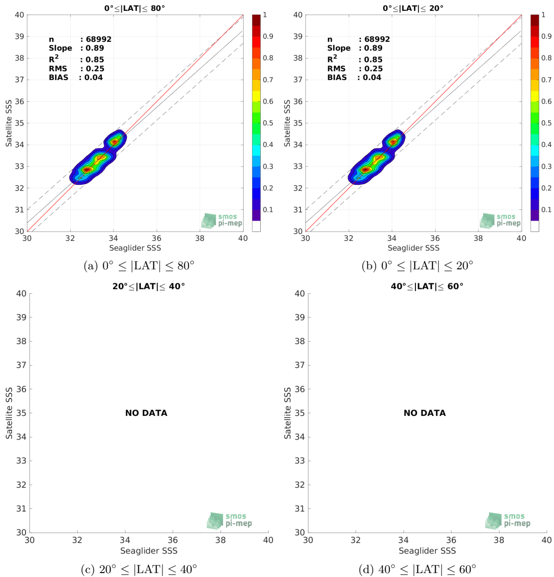
Figure 9: Contour maps of the concentration of SMAP SSS L3 v5.0 - Monthly (JPL) SSS (y-axis) versus Seaglider SSS (x-axis) at match-up pairs for different latitude bands. For each plot, the red line shows x=y . The black thin and dashed lines indicate a linear fit through the data cloud and the \pm 95\% confidence levels, respectively. The number match-up pairs n , the slope and R^2 coefficient of the linear fit, the root mean square (RMS) and the mean bias between satellite and in situ data are indicated for each latitude band in each plots.
