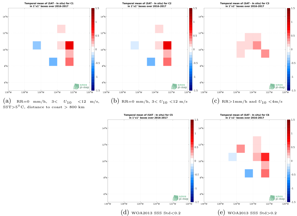
Figure 12: Temporal mean gridded over spatial boxes of size 1^\circ \times 1^\circ of \Delta SSS (SMAP SSS L3 v5.0 - Monthly (JPL) - Seaglider) for 5 different subdatasets corresponding to:RR=0 mm/h, 3 < U_{10} < 12 m/s, SST>5°C, distance to coast > 800 km (a), RR=0 mm/h, 3 < U_{10} < 12 m/s (b), RR>1mm/h and U_{10} < 4 m/s (c), WOA2013 SSS Std<0.2 (d), WOA2013 SSS Std>0.2 (e).
