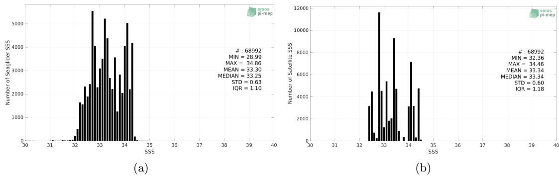
Figure 2: Histograms of SSS from Seaglider (a) and SMAP SSS L3 v5.0 - Monthly (JPL) (b) considering all match-up pairs per bins of 0.1 over the SPURS 2 Pi-MEP region and for the full satellite product period.
