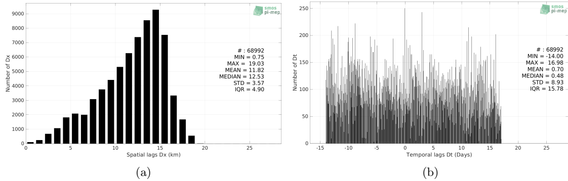
Figure 5: Histograms of the spatial (a) and temporal (b) lags between the location/time of the Seaglider measurement and the date of the corresponding SMAP SSS L3 v5.0 - Monthly (JPL) SSS pixel.
