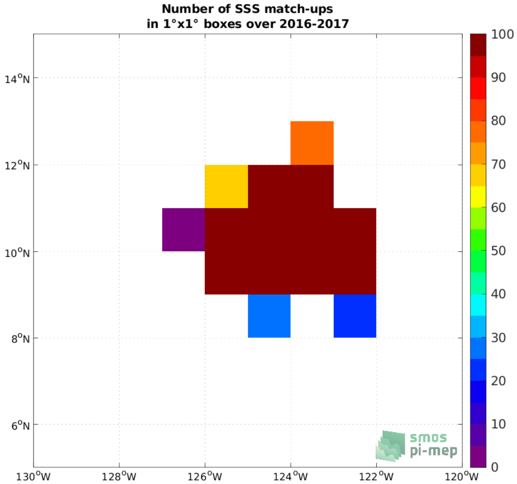
Figure 4: Number of SSS match-ups between Seaglider SSS and the SMAP SSS L3 v5.0 - Monthly (JPL) SSS product for the SPURS 2 Pi-MEP region over 1°x1° boxes and for the full satellite product period.
