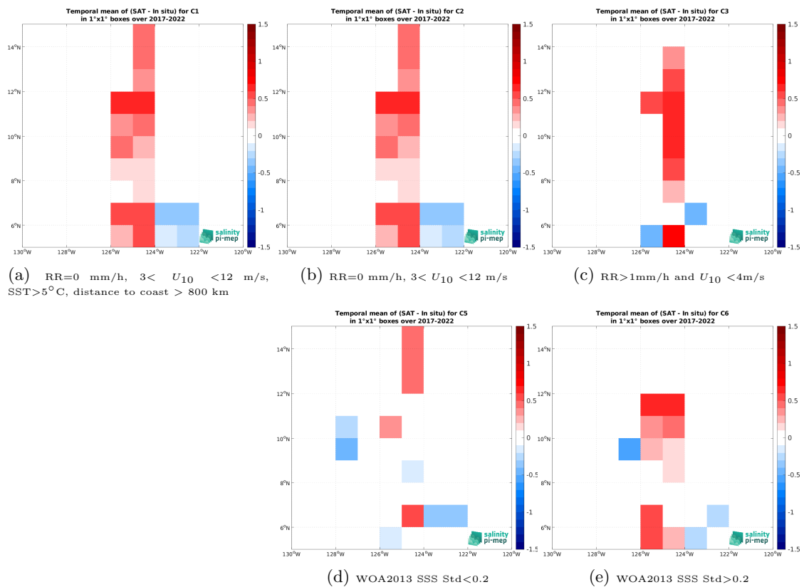
Figure 14: Temporal mean gridded over spatial boxes of size 1^\circ \times 1^\circ of \Delta SSS (SMAP SSS L3 v5.0 - Monthly (JPL) - Saildrone) for 5 different subdatasets corresponding to:RR=0 mm/h, 3 < U_{10} < 12 m/s, SST>5°C, distance to coast > 800 km (a), RR=0 mm/h, 3 < U_{10} < 12 m/s (b), RR>1mm/h and U_{10} < 4 m/s (c), WOA2013 SSS Std<0.2 (d), WOA2013 SSS Std>0.2 (e).
