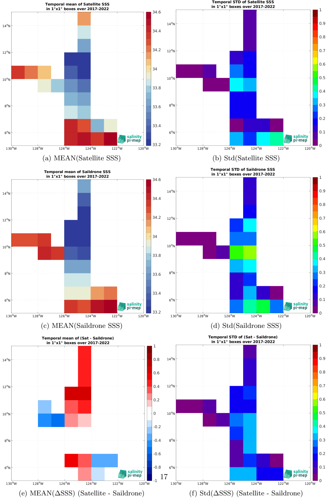
Figure 7: Temporal mean (left) and Std (right) of SSS from SMAP SSS L3 v5.0 - Monthly (JPL) (top), Saildrone (middle), and of \Delta SSS (Satellite - Saildrone). Only match-up pairs are used to generate these maps.
