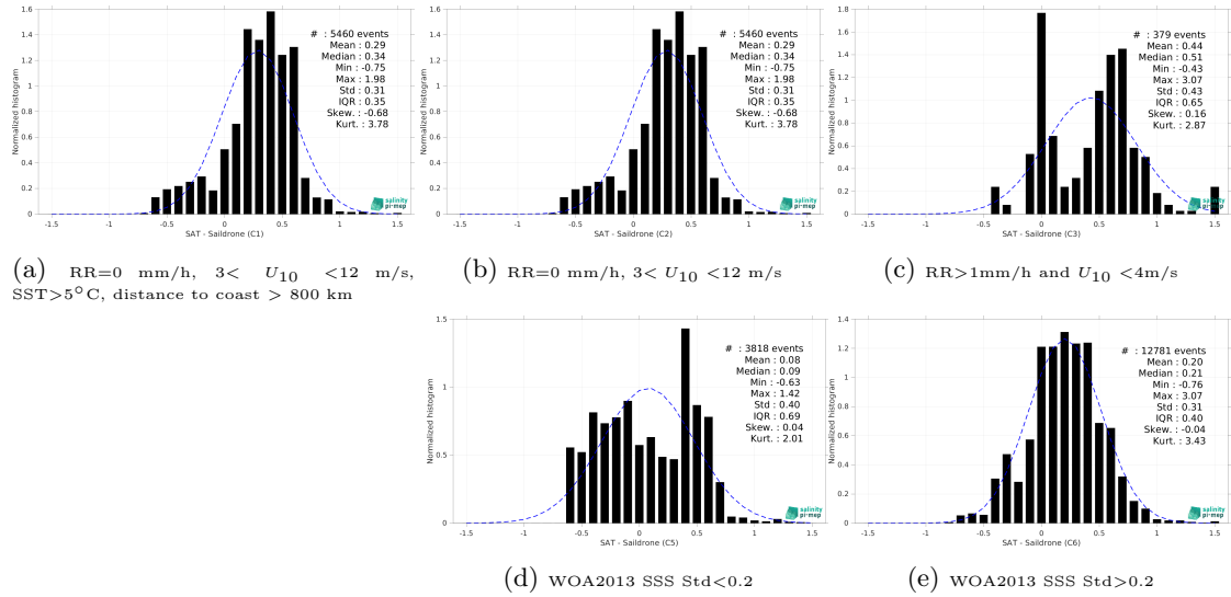
Figure 15: Normalized histogram of \Delta SSS (SMAP SSS L3 v5.0 - Monthly (JPL) - Saildrone) for 5 different subdatasets corresponding to: RR=0 mm/h, 3 < U_{10} < 12 m/s, SST > 5°C, distance to coast > 800 km (a), RR=0 mm/h, 3 < U_{10} < 12 m/s (b), RR > 1mm/h and U_{10} < 4 m/s (c), WOA2013 SSS Std < 0.2 (d), WOA2013 SSS Std > 0.2 (e).
