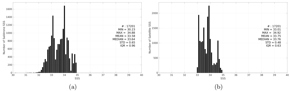
Figure 3: Histograms of SSS from Saildrone (a) and SMAP SSS L3 v5.0 - Monthly (JPL) (b) considering all match-up pairs per bins of 0.1 over the SPURS 2 Pi-MEP region and for the full satellite product period.
