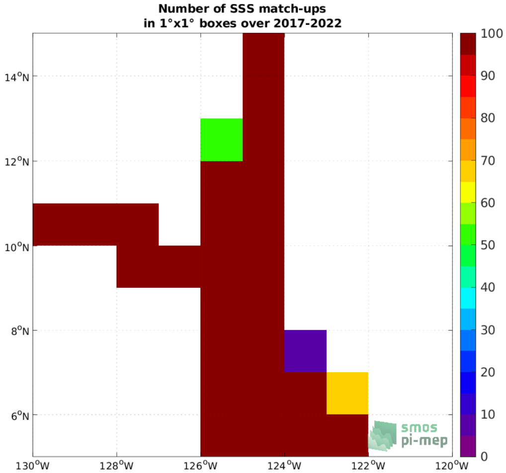
Figure 4: Number of SSS match-ups between Saildrone SSS and the SMAP SSS L3 v5.0 - Monthly (JPL) SSS product for the SPURS 2 Pi-MEP region over 1°×1° boxes and for the full satellite product period.
