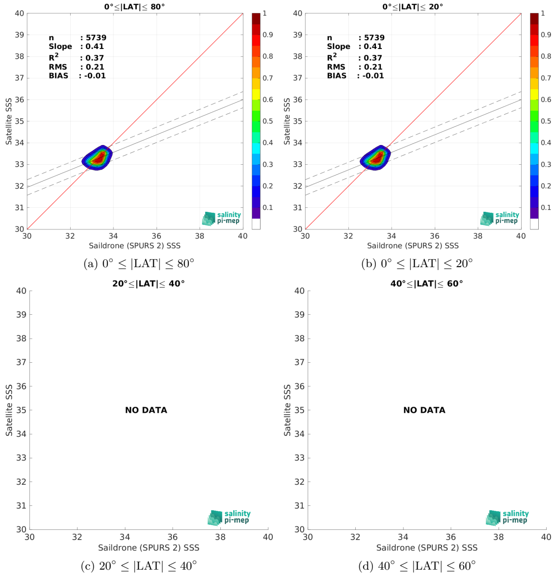
Figure 10: Contour maps of the concentration of SMAP SSS L3 v5.0 - Monthly (JPL) SSS (y-axis) versus Saildrone (SPURS 2) SSS (x-axis) at match-up pairs for different latitude bands. For each plot, the red line shows x=y . The black thin and dashed lines indicate a linear fit through the data cloud and the \pm 95\% confidence levels, respectively. The number match-up pairs n , the slope and R^2 coefficient of the linear fit, the root mean square (RMS) and the mean bias between satellite and in situ data are indicated for each latitude band in each plots.
