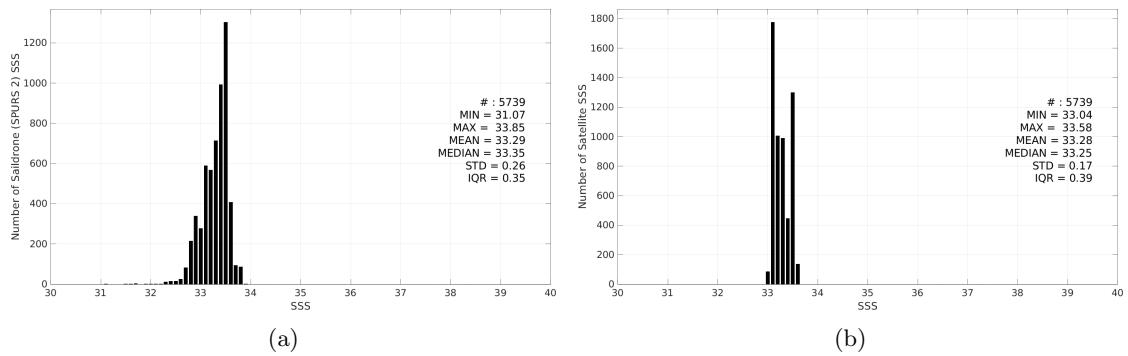
Figure 3: Histograms of SSS from Saildrone (SPURS 2) (a) and SMAP SSS L3 v5.0 - Monthly (JPL) (b) considering all match-up pairs per bins of 0.1 over the SPURS 2 Pi-MEP region and for the full satellite product period.
