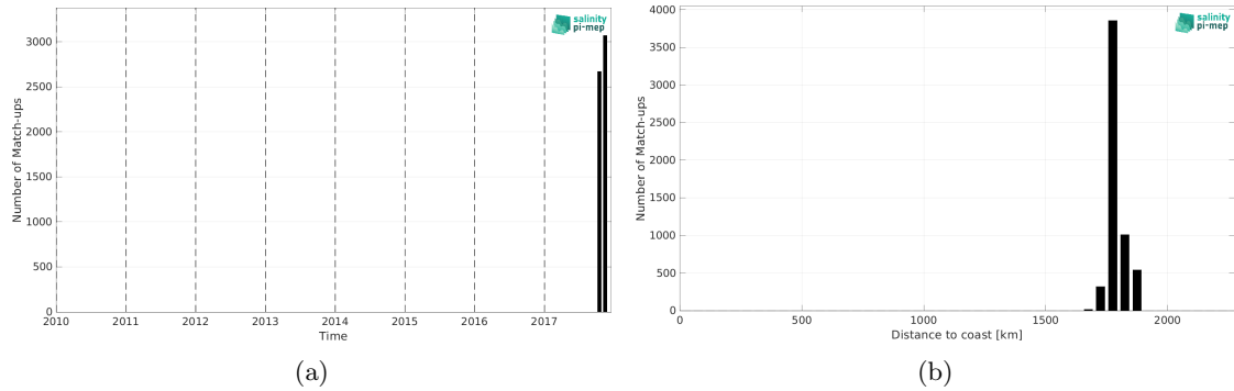
Figure 2: Number of match-ups between Saildrone (SPURS 2) and SMAP SSS L3 v5.0 - Monthly (JPL) SSS as a function of time (a) and as function of the distance to coast (b) over the SPURS 2 Pi-MEP region and for the full satellite product period.
