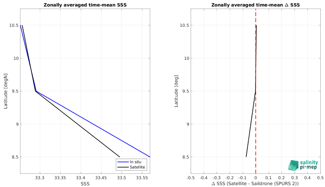
Figure 9: Left panel: Zonal mean SSS from SMAP SSS L3 v5.0 - Monthly (JPL) satellite product (black) and from Sairdron (SPURS 2) (blue). Right panel: Zonal mean of \Delta SSS (Satellite - Sairdron (SPURS 2)) for all the collected Pi-MEP match-up pairs estimated over the full satellite product period.
