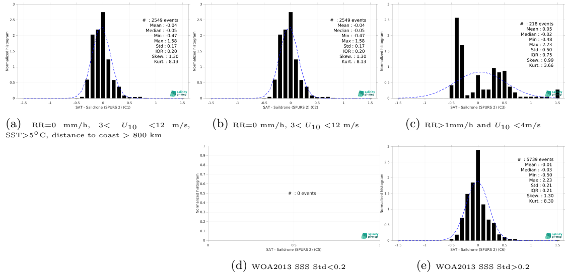
Figure 15: Normalized histogram of \Delta SSS (SMAP SSS L3 v5.0 - Monthly (JPL) - Sailability (SPURS 2)) for 5 different subdatasets corresponding to: RR=0 mm/h, 3 < U_{10} < 12 m/s, SST > 5°C, distance to coast > 800 km (a), RR=0 mm/h, 3 < U_{10} < 12 m/s (b), RR > 1mm/h and U_{10} < 4 m/s (c), WOA2013 SSS Std < 0.2 (d), WOA2013 SSS Std > 0.2 (e).
