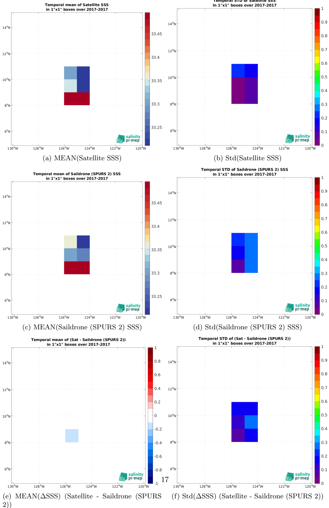
Figure 7: Temporal mean (left) and Std (right) of SSS from SMAP SSS L3 v5.0 - Monthly (JPL) (top), Saildrone (SPURS 2) (middle), and of \Delta SSS (Satellite - Saildrone (SPURS 2)). Only match-up pairs are used to generate these maps.
