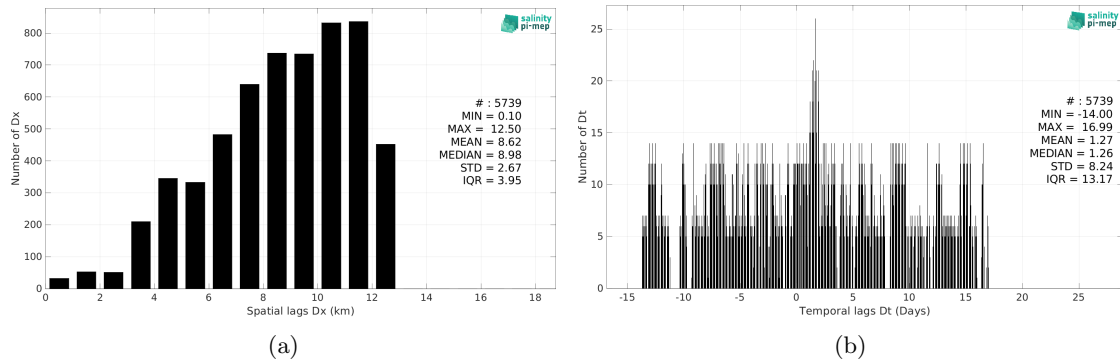
Figure 6: Histograms of the spatial (a) and temporal (b) lags between the location/time of the Saildrone (SPURS 2) measurement and the date of the corresponding SMAP SSS L3 v5.0 - Monthly (JPL) SSS pixel.
