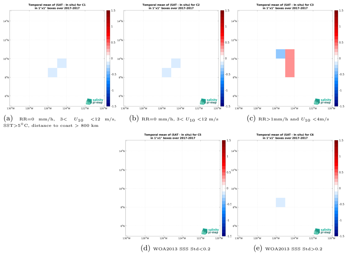
Figure 14: Temporal mean gridded over spatial boxes of size 1^\circ \times 1^\circ of \Delta SSS (SMAP SSS L3 v5.0 - Monthly (JPL) - Sailability (SPURS 2)) for 5 different subdatasets corresponding to:RR=0 mm/h, 3 < U_{10} < 12 m/s, SST>5°C, distance to coast > 800 km (a), RR=0 mm/h, 3 < U_{10} < 12 m/s (b), RR>1mm/h and U_{10} < 4 m/s (c), WOA2013 SSS Std<0.2 (d), WOA2013 SSS Std>0.2 (e).
