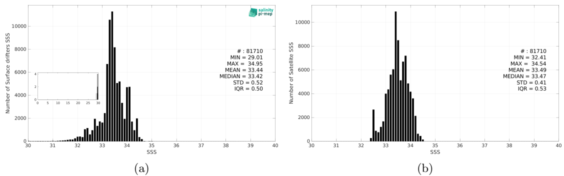
Figure 3: Histograms of SSS from Surface drifters (a) and SMAP SSS L3 v5.0 - Monthly (JPL) (b) considering all match-up pairs per bins of 0.1 over the SPURS 2 Pi-MEP region and for the full satellite product period.
