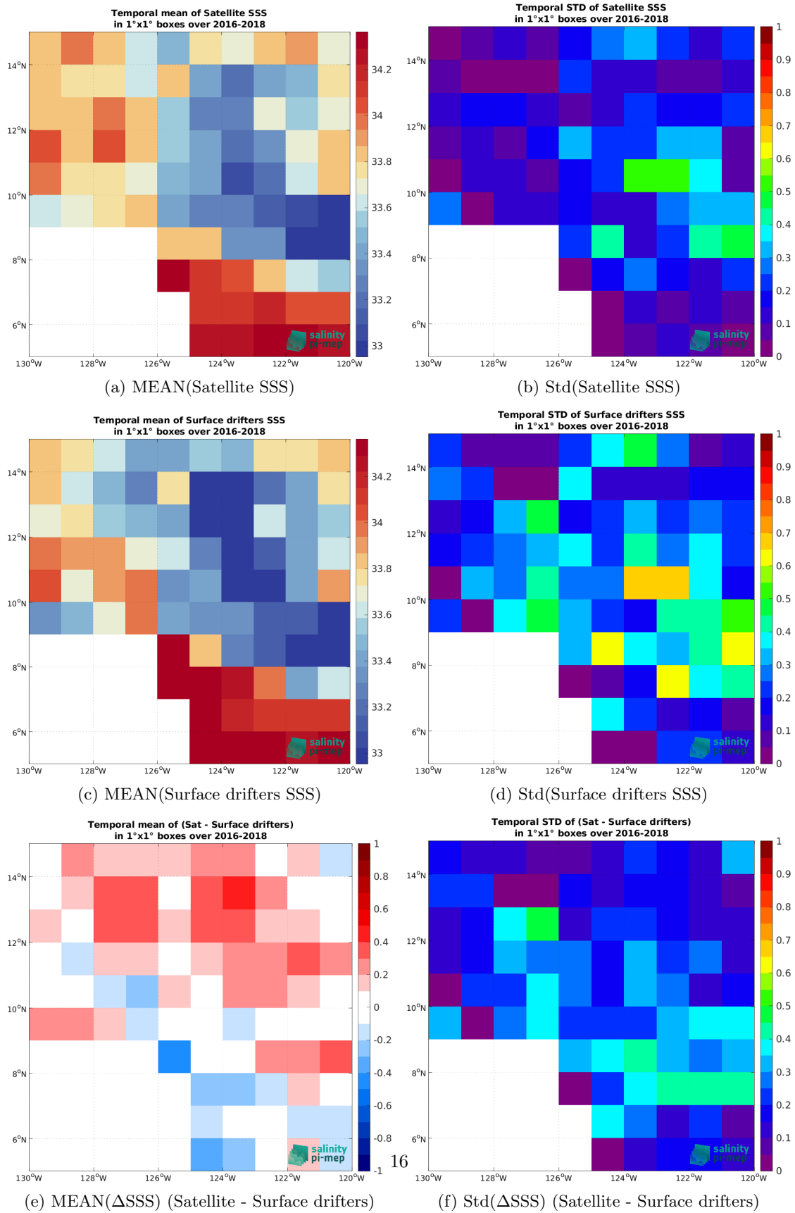
Figure 6: Temporal mean (left) and Std (right) of SSS from SMAP SSS L3 v5.0 - Monthly (JPL) (top), Surface drifters (middle), and of \Delta SSS (Satellite - Surface drifters). Only match-up pairs are used to generate these maps.
