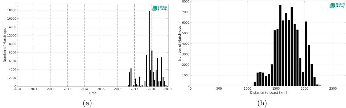
Figure 2: Number of match-ups between Surface drifters and SMAP SSS L3 v5.0 - Monthly (JPL) SSS as a function of time (a) and as function of the distance to coast (b) over the SPURS 2 Pi-MEP region and for the full satellite product period.
