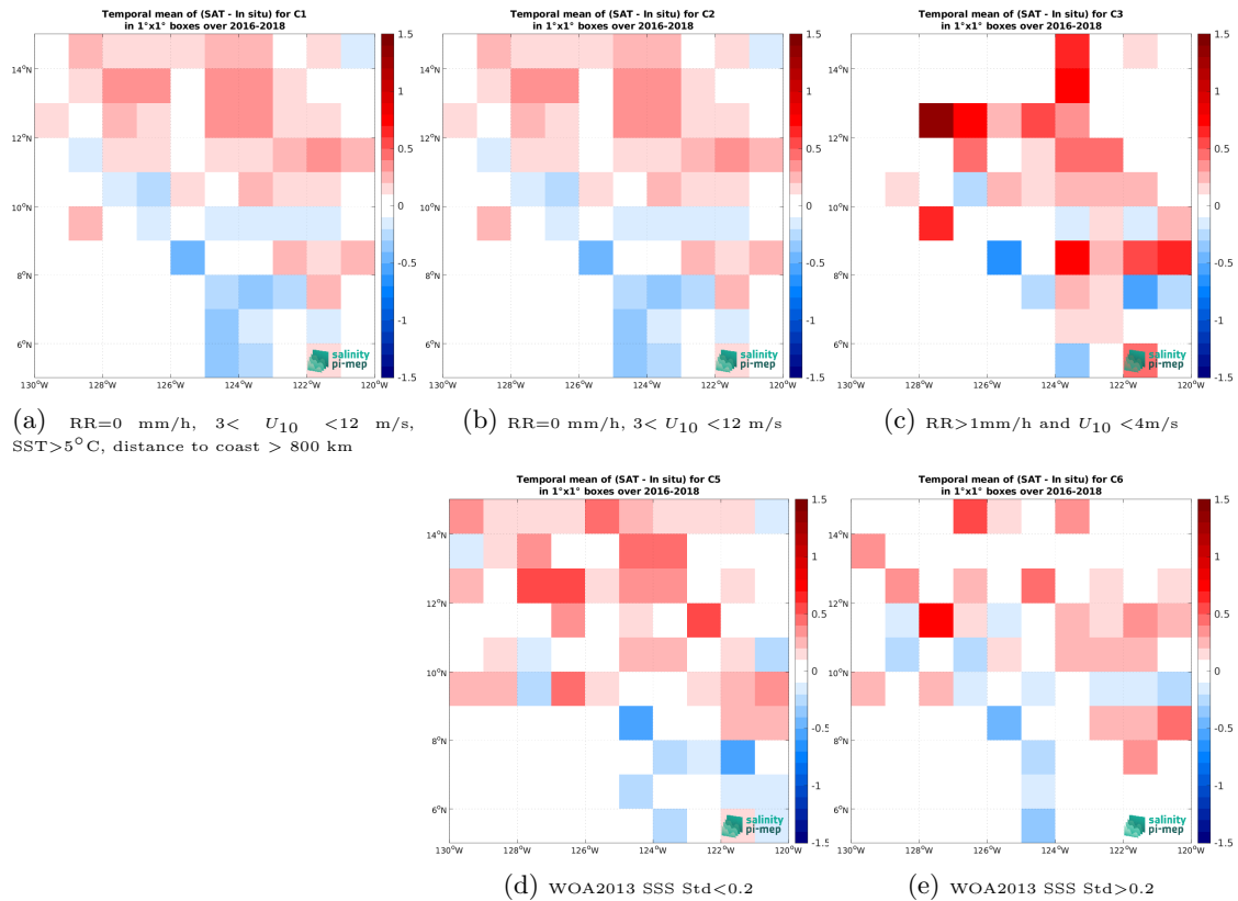
Figure 13: Temporal mean gridded over spatial boxes of size 1^\circ \times 1^\circ of \Delta\text{SSS} (SMAP SSS L3 v5.0 - Monthly (JPL) - Surface drifters) for 5 different subdatasets corresponding to:RR=0 mm/h, 3 < U_{10} < 12 m/s, SST > 5^\circ\text{C} , distance to coast > 800 km (a), RR=0 mm/h, 3 < U_{10} < 12 m/s (b), RR > 1 mm/h and U_{10} < 4 m/s (c), WOA2013 SSS Std < 0.2 (d), WOA2013 SSS Std > 0.2 (e).
