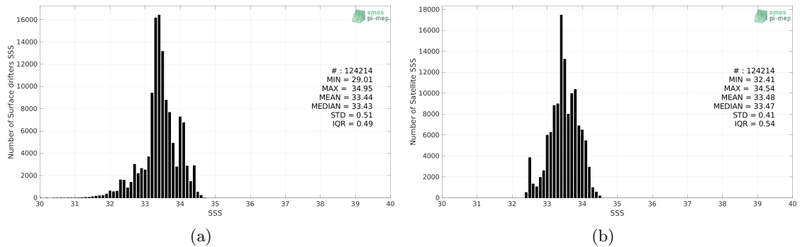
Figure 2: Histograms of SSS from Surface drifters (a) and SMAP SSS L3 v5.0 - Monthly (JPL) (b) considering all match-up pairs per bins of 0.1 over the SPURS 2 Pi-MEP region and for the full satellite product period.
