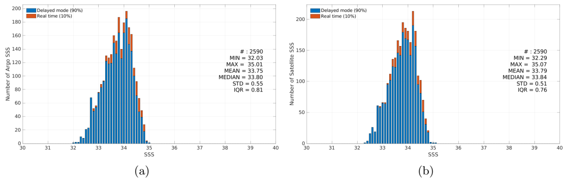
Figure 3: Histograms of SSS from Argo (a) and SMAP SSS L3 v5.0 - Monthly (JPL) (b) considering all match-up pairs per bins of 0.1 over the SPURS 2 Pi-MEP region and for the full satellite product period.
