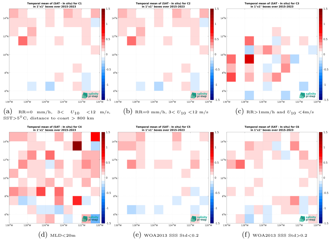
Figure 14: Temporal mean gridded over spatial boxes of size 1^\circ \times 1^\circ of \Delta SSS (SMAP SSS L3 v5.0 - Monthly (JPL) - Argo) for 6 different subdatasets corresponding to:RR=0 mm/h, 3 < U_{10} < 12 m/s, SST >5^\circ C, distance to coast > 800 km (a), RR=0 mm/h, 3 < U_{10} < 12 m/s (b), RR >1 mm/h and U_{10} < 4 m/s (c),MLD <20 m (d),WOA2013 SSS Std <0.2 (e),WOA2013 SSS Std >0.2 (f).
