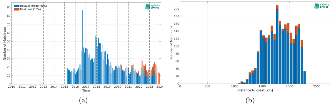
Figure 2: Number of match-ups between Argo and SMAP SSS L3 v5.0 - Monthly (JPL) SSS as a function of time (a) and as function of the distance to coast (b) over the SPURS 2 Pi-MEP region and for the full satellite product period.
