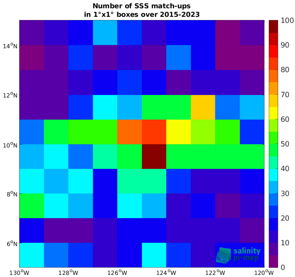
Figure 5: Number of SSS match-ups between Argo SSS and the SMAP SSS L3 v5.0 - Monthly (JPL) SSS product for the SPURS 2 Pi-MEP region over 1°x1° boxes and for the full satellite product period.
