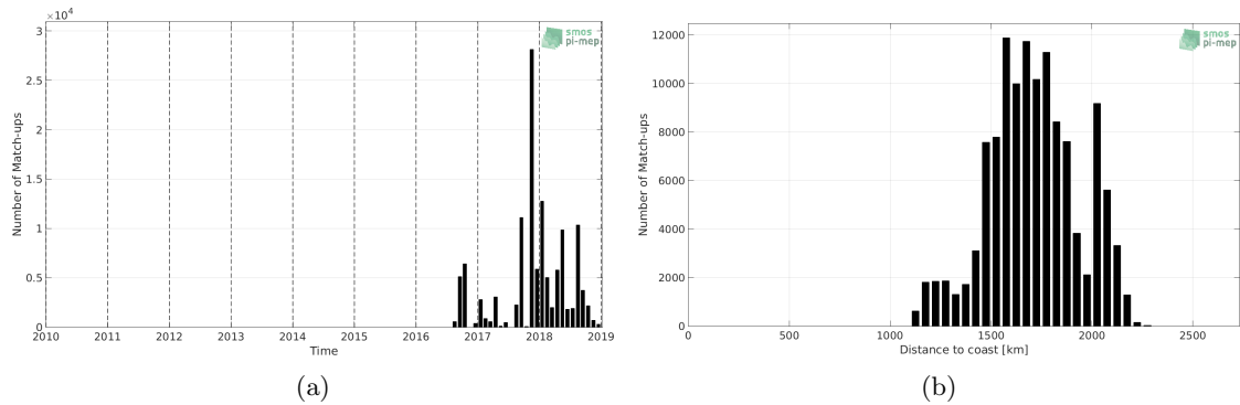
Figure 1: Number of match-ups between Surface drifters and SMAP-L3-JPL-V4.3-MONTHLY-60KM SSS as a function of time (a) and as function of the distance to coast (b) over the SPURS 2 Pi-MEP region and for the full satellite product period.
