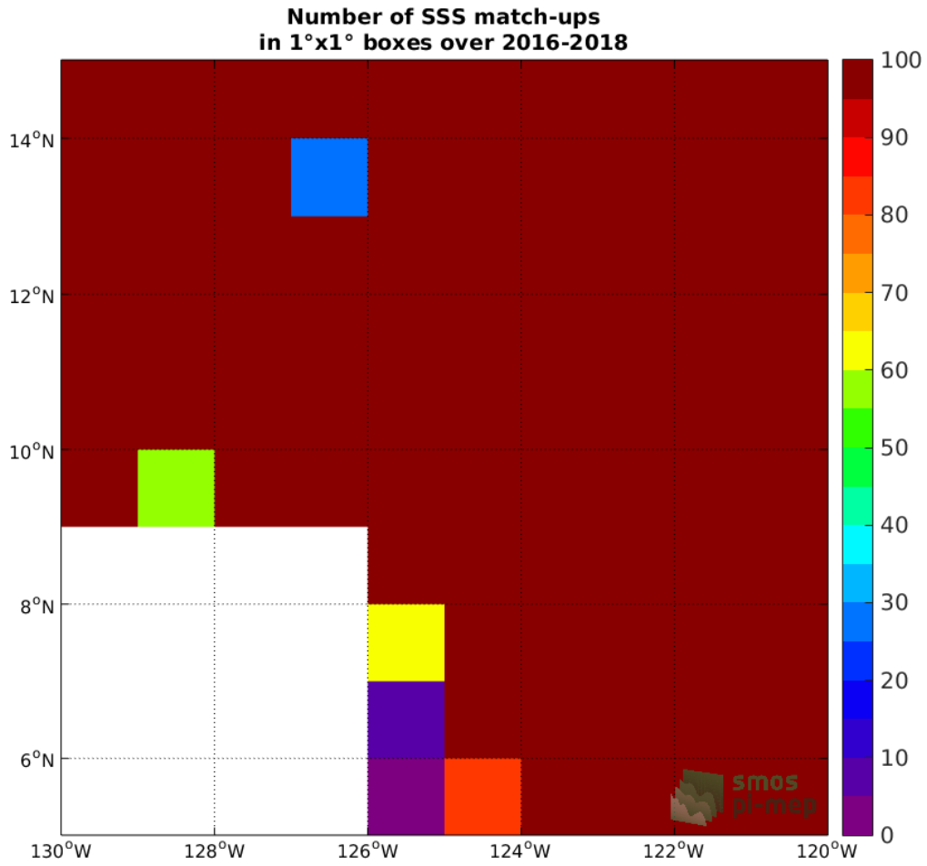
Figure 3: Number of SSS match-ups between Surface drifters SSS and the SMAP-L3-JPL-V4.3-MONTHLY-60KM SSS product for the SPURS 2 Pi-MEP region over 1°x1° boxes and for the full satellite product period.
