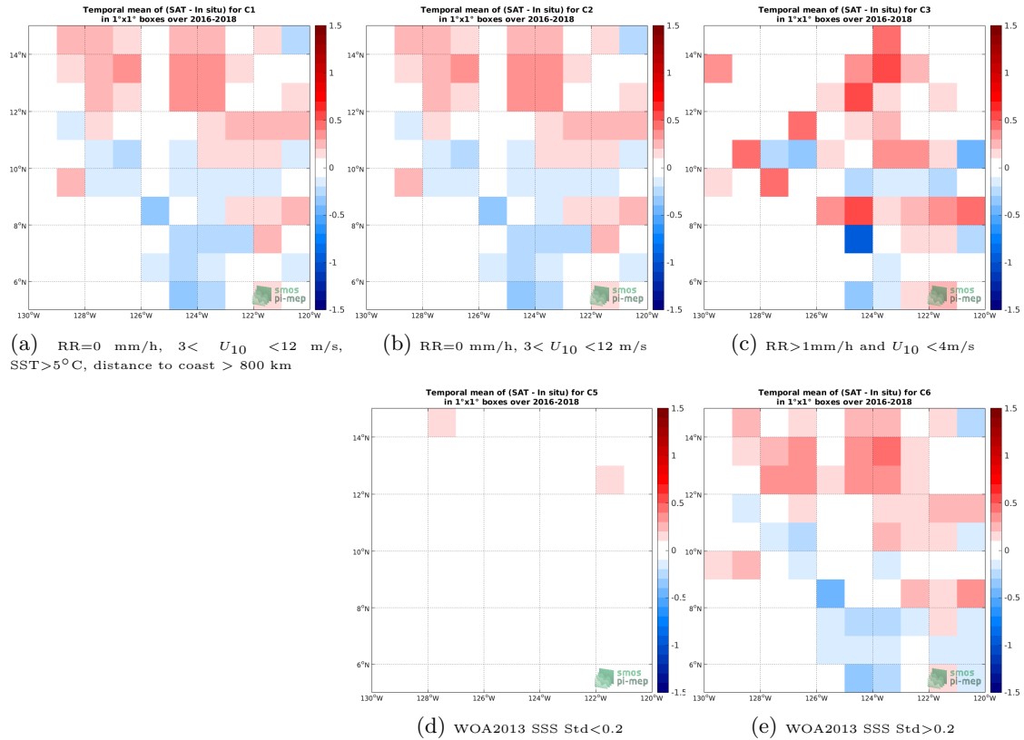
Figure 11: Temporal mean gridded over spatial boxes of size 1^\circ \times 1^\circ of \Delta SSS (SMAP-L3-JPL-V4.3-MONTHLY-60KM - Surface drifters) for 5 different subdatasets corresponding to: RR=0 mm/h, 3 < U_{10} < 12 m/s, SST > 5^\circ C , distance to coast > 800 km (a), RR=0 mm/h, 3 < U_{10} < 12 m/s (b), RR > 1 mm/h and U_{10} < 4 m/s (c), WOA2013 SSS Std < 0.2 (d), WOA2013 SSS Std > 0.2 (e).
