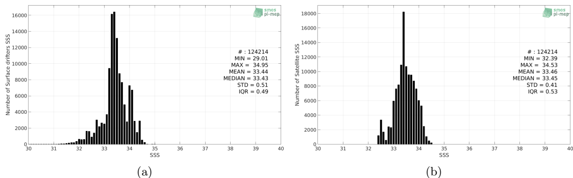
Figure 2: Histograms of SSS from Surface drifters (a) and SMAP-L3-JPL-V4.3-MONTHLY-60KM (b) considering all match-up pairs per bins of 0.1 over the SPURS 2 Pi-MEP region and for the full satellite product period.
