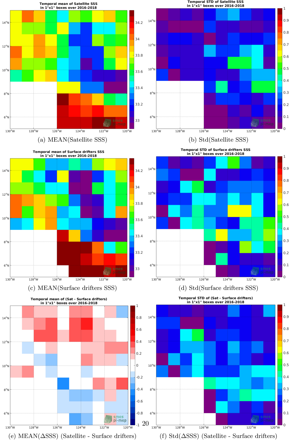
Figure 5: Temporal mean (left) and Std (right) of SSS from SMAP-L3-JPL-V4.3-MONTHLY-60KM (top), Surface drifters (middle), and of \Delta SSS (Satellite - Surface drifters). Only match-up pairs are used to generate these maps.
