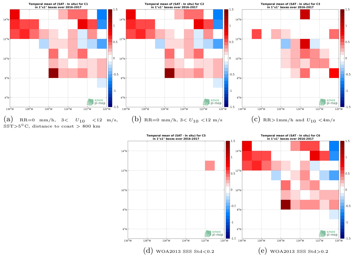
Figure 11: Temporal mean gridded over spatial boxes of size 1^\circ \times 1^\circ of \Delta SSS (SMAP-L3-JPL-V4.3-MONTHLY-60KM - Surface drifters) for 5 different subdatasets corresponding to:RR=0 mm/h, 3 < U_{10} < 12 m/s, SST >5^\circ C, distance to coast > 800 km (a), RR=0 mm/h, 3 < U_{10} < 12 m/s (b), RR >1 mm/h and U_{10} < 4 m/s (c), WOA2013 SSS Std <0.2 (d), WOA2013 SSS Std >0.2 (e).
